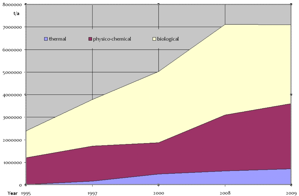
Stationary soil treatment installations in Germany (permitted capacity)
