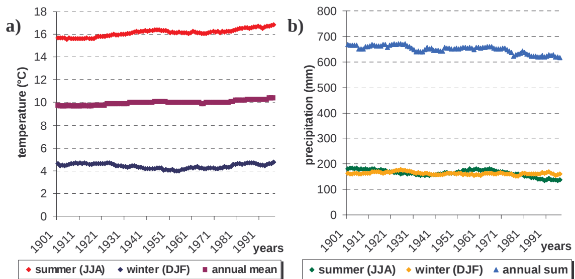
Figure 16 Observed data from meteorological station in Oxford. Shown are 30-year means of a) temperature and b) seasonal and annual precipitation sums. Data provided by MetOffice, UK.
