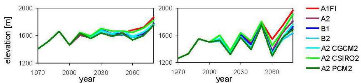
Figure 9 Elevation of snow line (elevation above which the snow cover is reliable) as projected for seven future climate scenarios. The left chart shows the Alptal catchment, the right chart shows the Verzasca-Lavertezzo catchment (Schröter et al., 2004).
