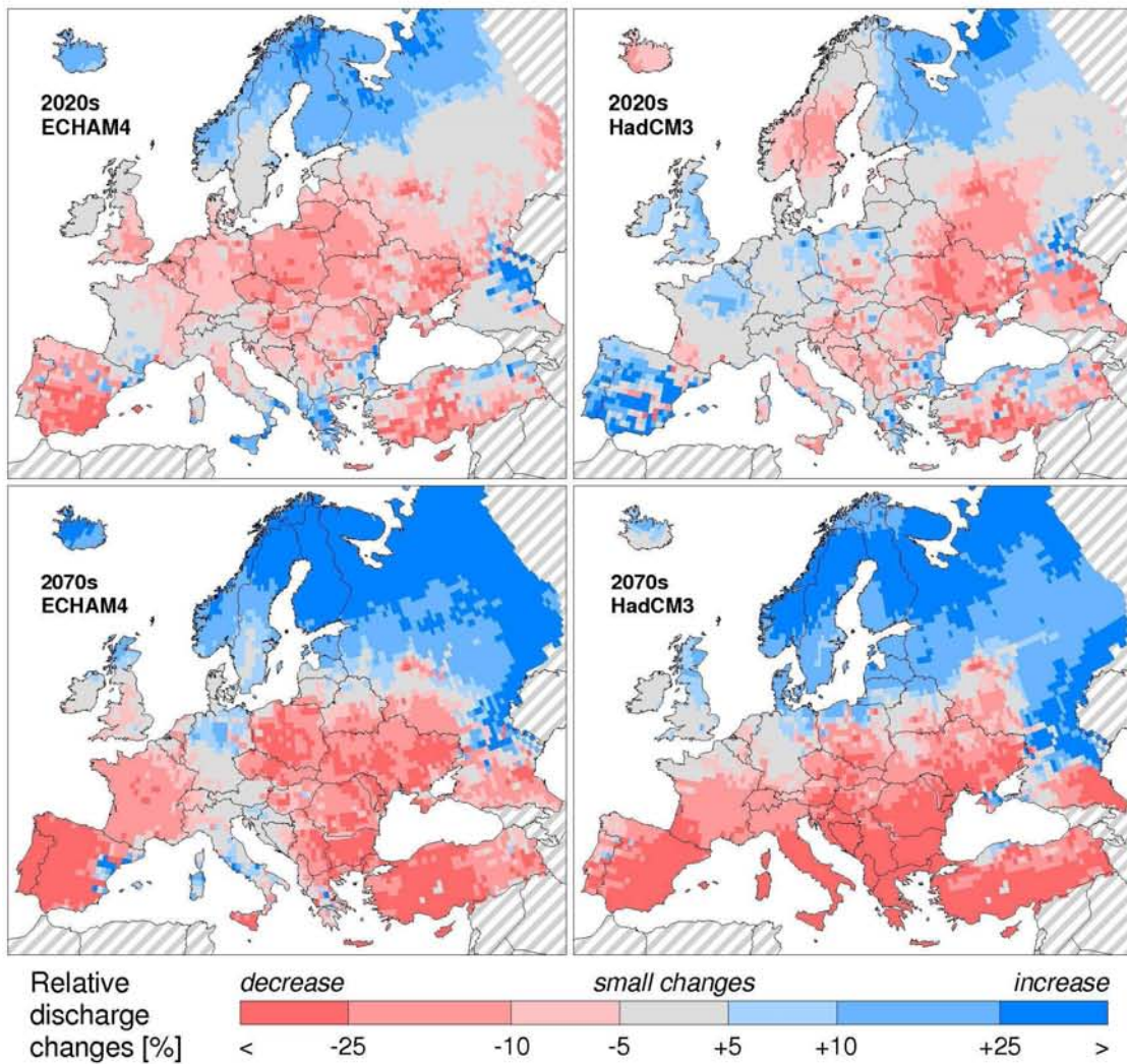
Figure 8 Change in river basin discharge under climate change. Depicted are relative changes of annual average river basin discharge between the climate normal period (1961-90) and two future time slices (2020s) and (2070s). Computations from WaterGAP 2.1 model (Alcamo et al. , 2003; Döll, 2002) with climate scenarios based on the IS92a scenario as computed by the ECHAM4 and HadCM3 global climate models, and with a reference water use scenario (Lehner et al. 2006).
