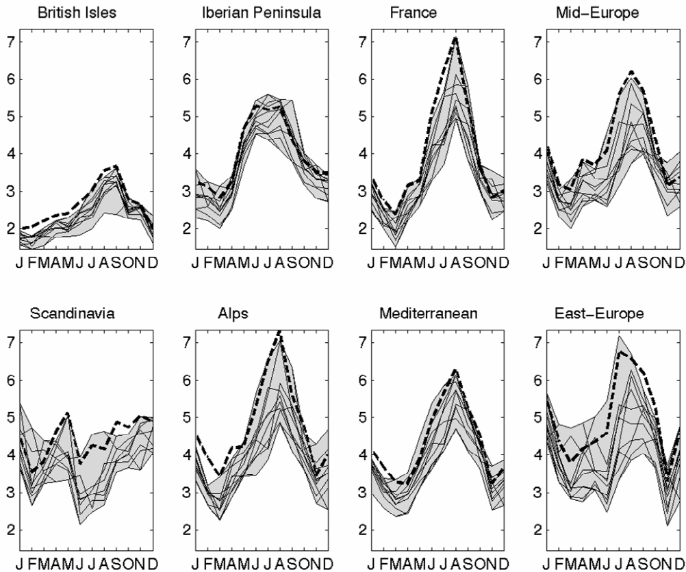
Figure 3 Monthly changes in temperature for different regions in Europe simulated by an ensemble of different RCMs in the project PRUDENCE (Jacob et al. 2007). Shown is the signal in 2m-Temperature, 2071-2100 minus 1961-1990 for the A2 SRES scenario. The thick black line indicates the result of the driving GCM for the region.
