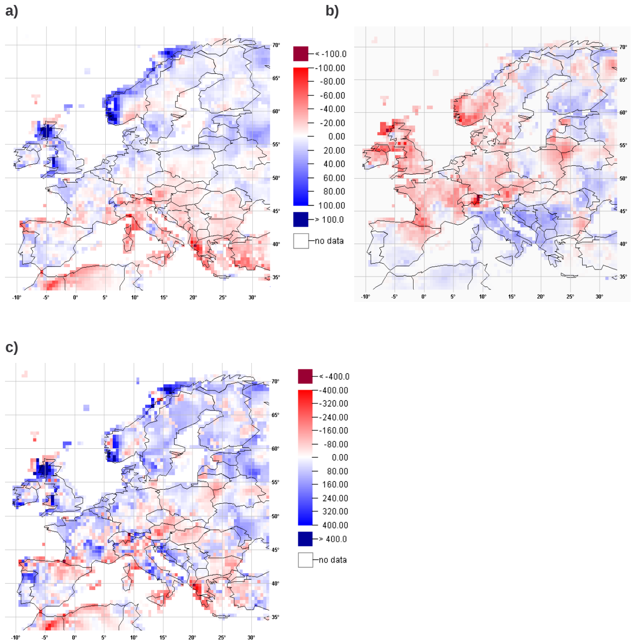
Figure 2 The observed trend in precipitation over the last century (difference mean annual values 1975/2004 and 1931/1960) for a) winter and b) summer season (seasonal sums in mm), and c) annual averages (annual sums in mm). (This reference period was chosen instead of 1901/1930, because many time series do not cover the first decades of the 20 th century). Source: PIK Global Climate Dataset, 2007.
