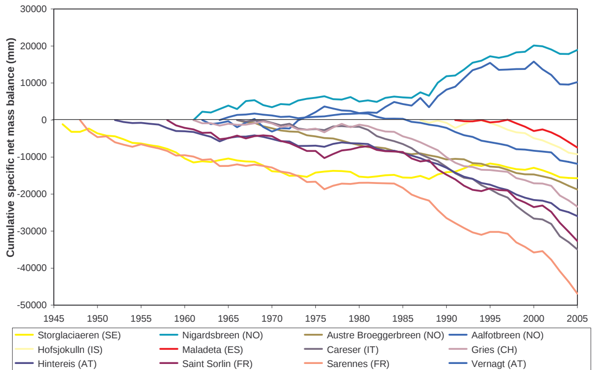
Figure 7 Change in cumulative specific net mass balance of glaciers from all European glacier regions between 1946 and 2005. Source: World Glacier Monitoring Centre, 2007.
