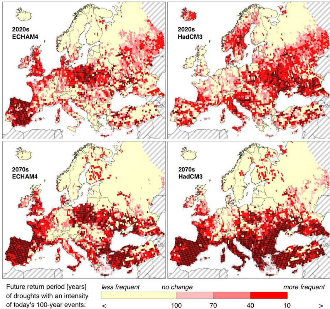
Figure 11 Changes in 100-year return-levels of river discharge in recurrence of 100-year droughts for the 2020s and 2070s using ECHAM4 and HadCM3 climate models and Baseline-A water use scenario (source: Lehner et al. 2005).
