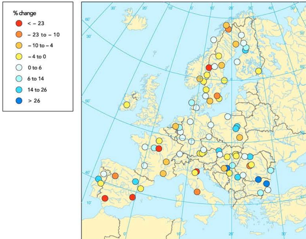
Figure 5 Changes of the mean annual river discharges over the twentieth century (EEA, 2004; permission for reproduction obtained).
