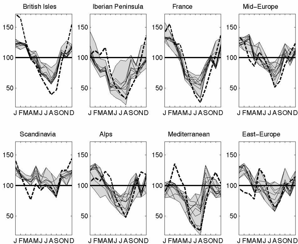
Figure 4 Monthly changes in precipitation for different regions in Europe simulated by an ensemble of different RCMs in the project PRUDENCE (Jacob et al. 2007). Shown is the difference 2071-2100 minus 1961-1990 for the A2 SRES scenario. The thick black line indicates the result of the driving GCM for the region.
