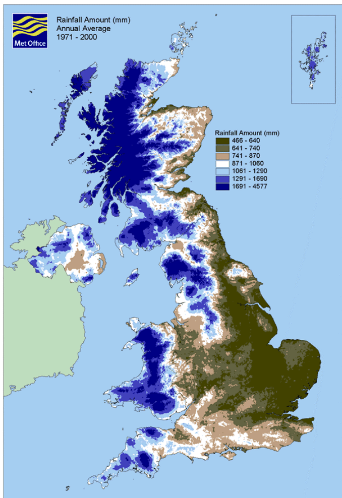
Figure 15 Annual average rainfall amount in the United Kingdom during the period 1971-2000 (Met Office, 2006).
