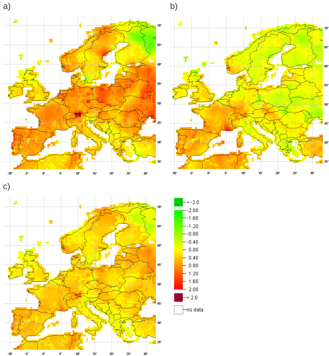
Figure 1 The observed trend in temperature over the last century (difference mean annual values 1975/2004 and 1931/1960) for the a) winter and b) summer season, and c) annual averages (This reference period was chosen instead of 1901/1930, because many time series do not cover the first decades of the 20 th century. Source: PIK Global Climate Dataset, 2007).
