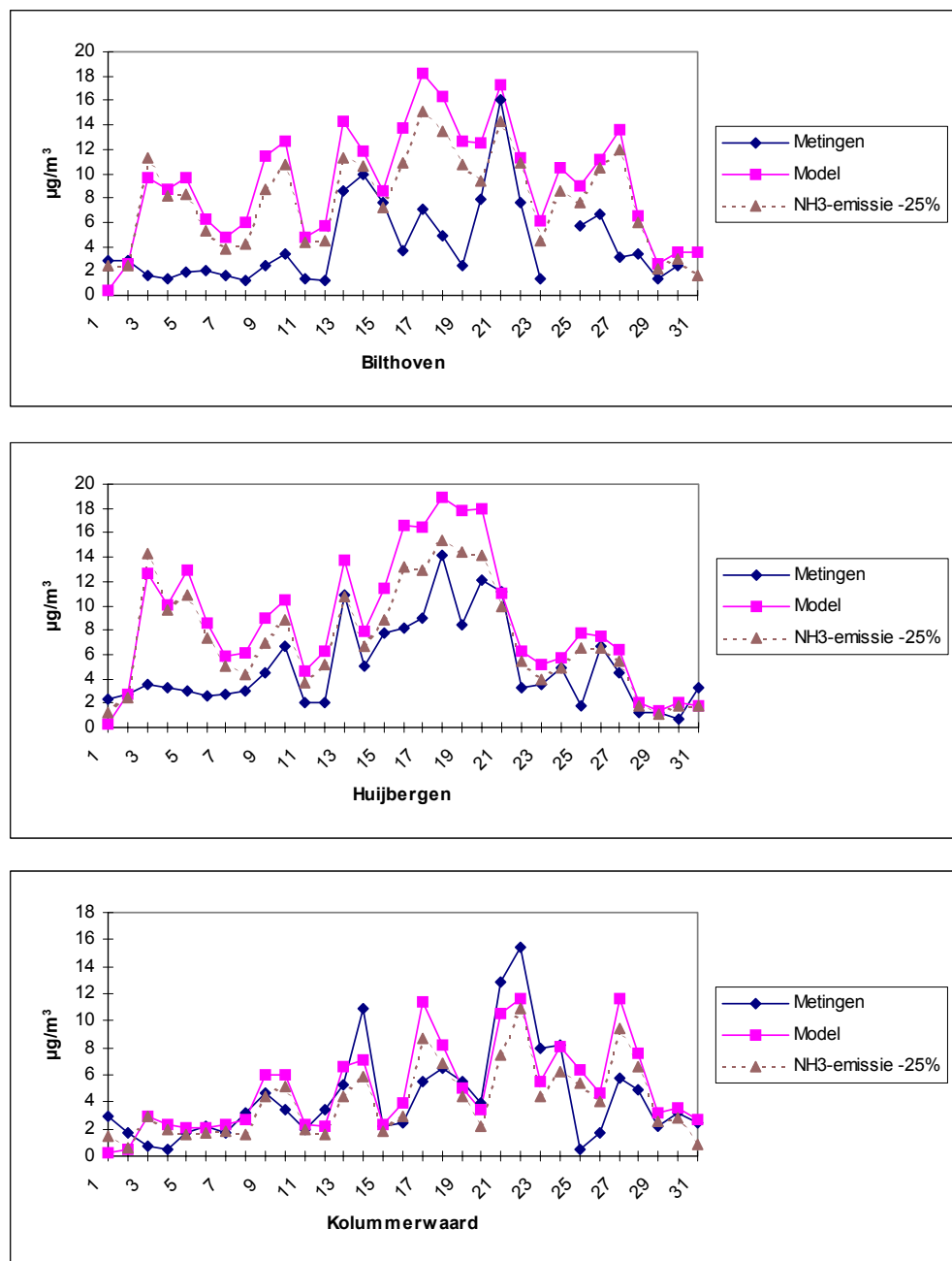
Figure 6.3 Measured and calculated daily averaged nitrate-concentrations for 6 measuring stations in August 1997
