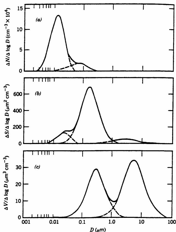
Figure 2.1 Size-, surface and volumedistributions of a typical urban aerosol. Source: Witby and Sverdrup, 1980.
