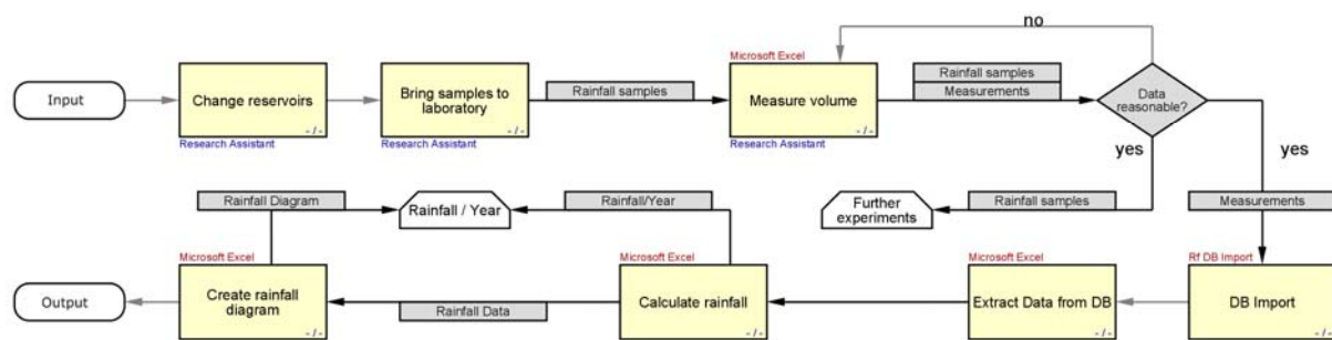
Figure 1. A process describing the calculation of the average rainfall per year
