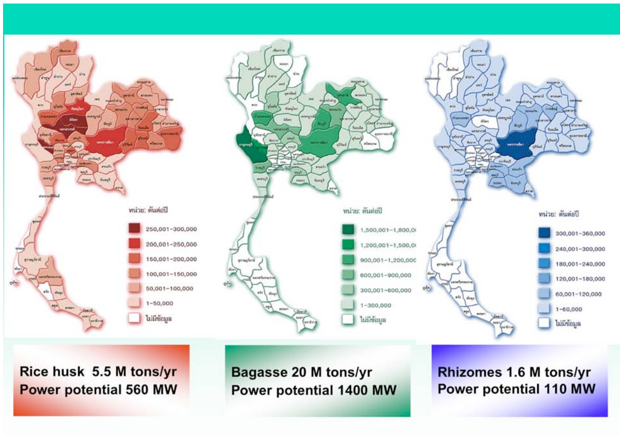
Figure 6.9: Power Potential from Rice Husk, Bagasse and Rhizomes
