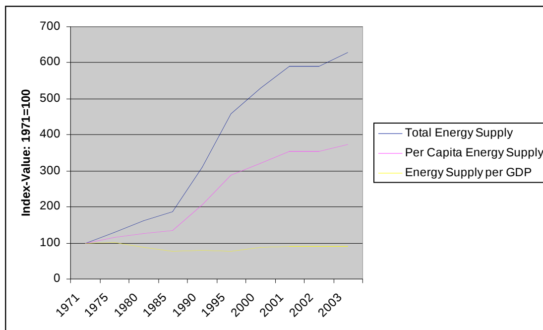
Figure 6.2: Energy Supply: Relative Trends, Thailand 1971-2003
