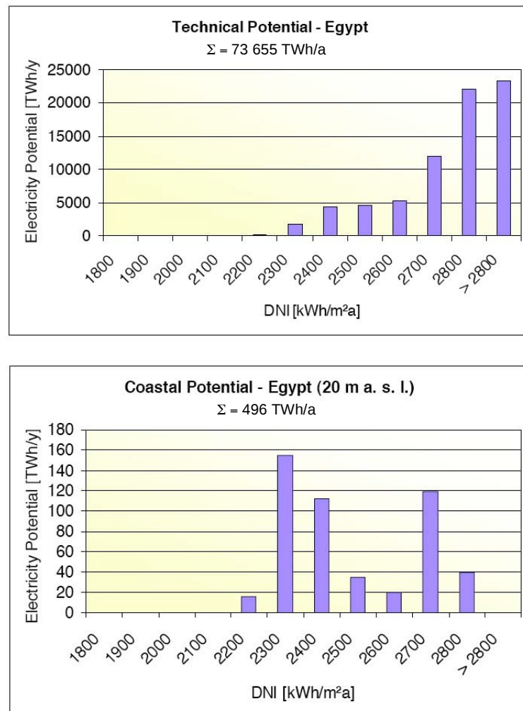
Figure 5.8 Comparison of Egypt's Technical and Coastal CSP Potential in \text{kWh/m}^2/\text{y} DNI
