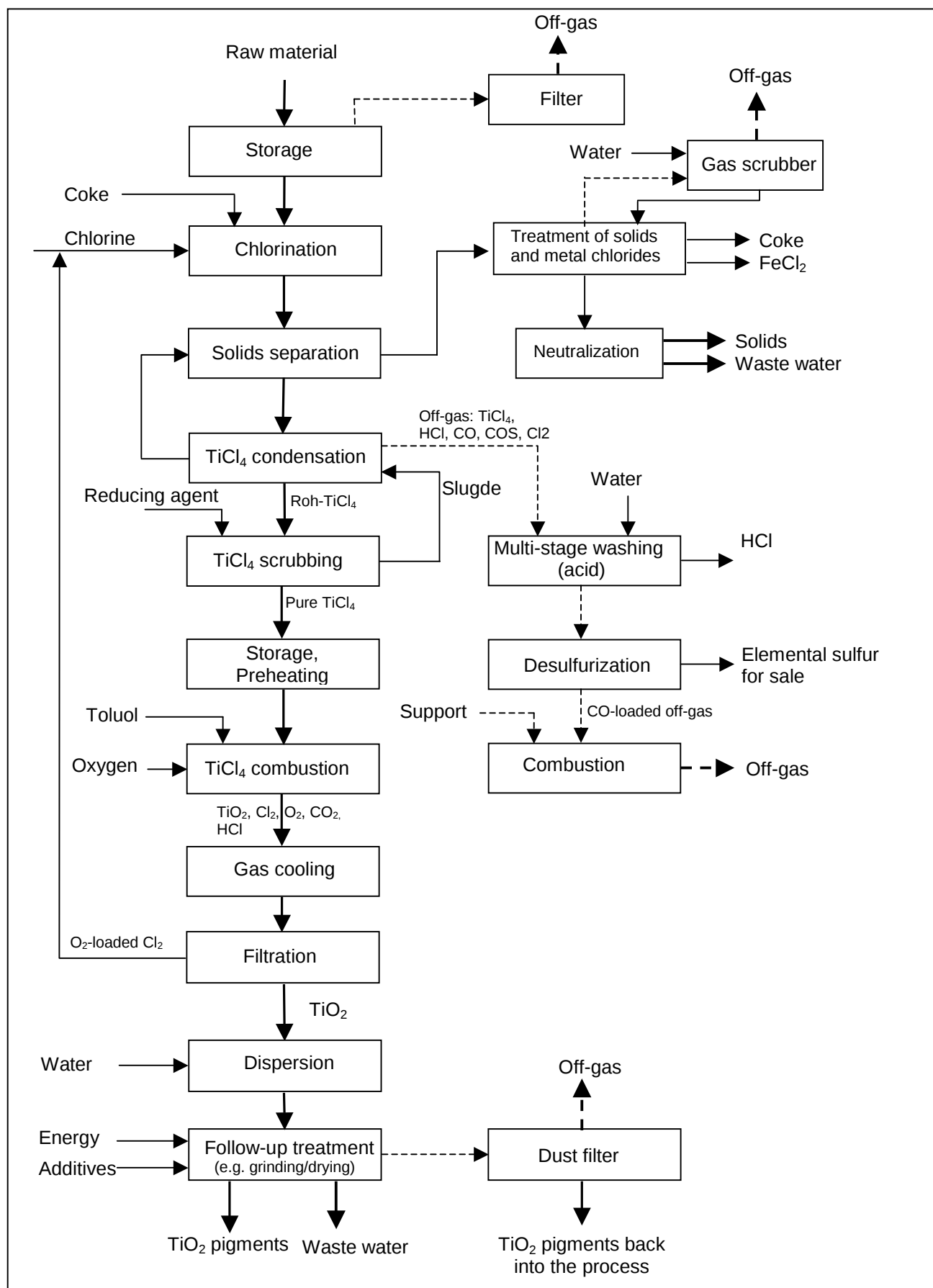
Figure 2.2.1.1: TiO 2 Production by Means of the Chloride Process
