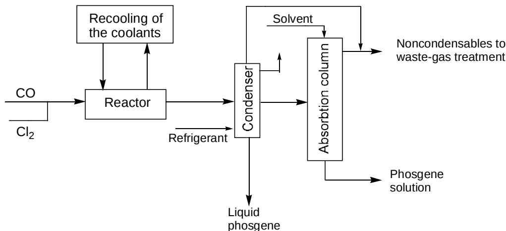
Abb.1: Block diagram of phosgene production
