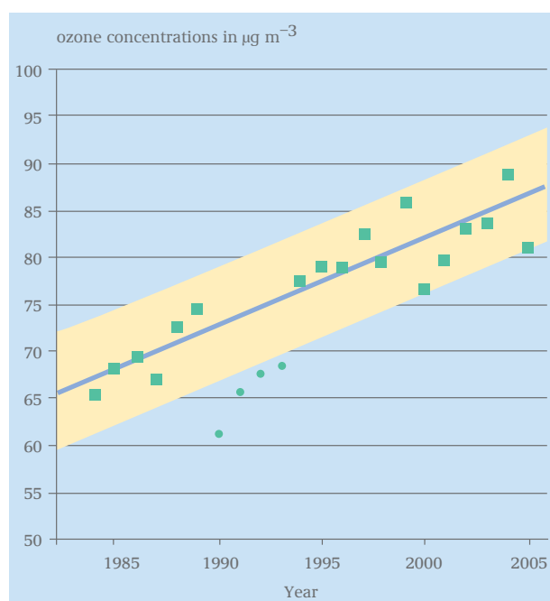
Figure 15: Average annual readings of ozone concentrations selected to wind direction and speed obtained at Westerland monitoring station
