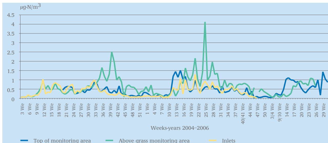
Figure 16: Trend in concentrations of ammonia as sampled at two different heights at the Neuglobsow monitoring station (blue: 2.5 m above ground level, green: 0.5 m above ground level)
