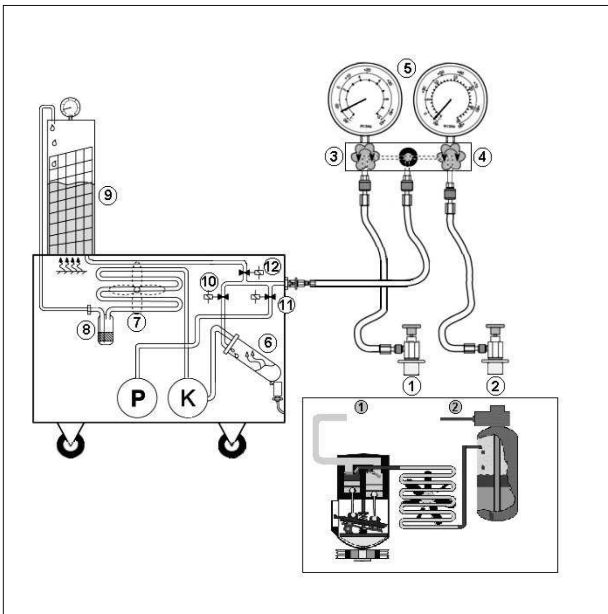
Fig. 1: Typical recovery/recharging station for passenger-car air-conditioning systems - (1) low-pressure hose connection; (2) high-pressure hose connection; (3) and (4) valve cocks; (5) pressure gauge dials; (6) oil separator or trap; (7) condenser; (8) filter dryer; (9) reservoir tank; (10) (11) (12) solenoid valves; (P) vacuum pump; (K) compressor. Bottom right: compressor, condenser and filter-dryer of car air-conditioning system. Grey (1) and (2): low-pressure and high-pressure air-conditioning-system service connections. (Source: DaimlerChrysler 2001 - modified).
