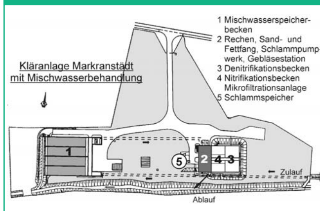
Figure 39: Site map (land use) of the Markranstädt sewage treatment plant
