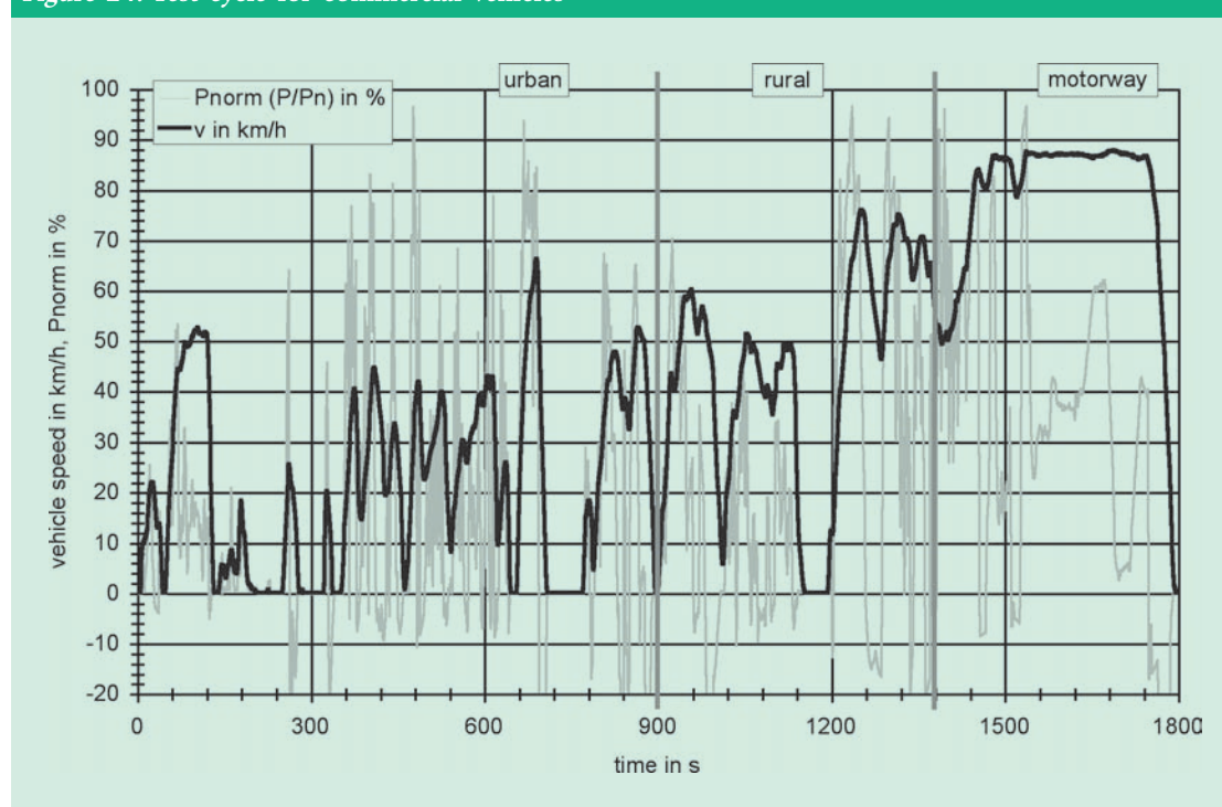
Figure 24: Test cycle for commercial vehicles
