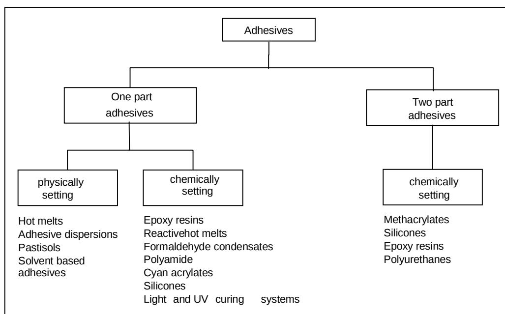
Figure III-4: Classification of the adhesives by the setting mechanism
