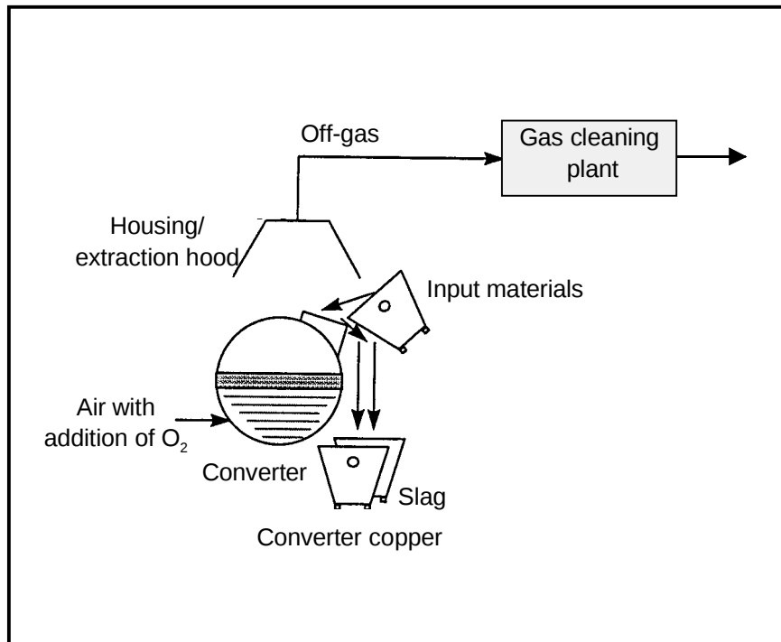
Figure 2-2: Pierce-Smith converter
