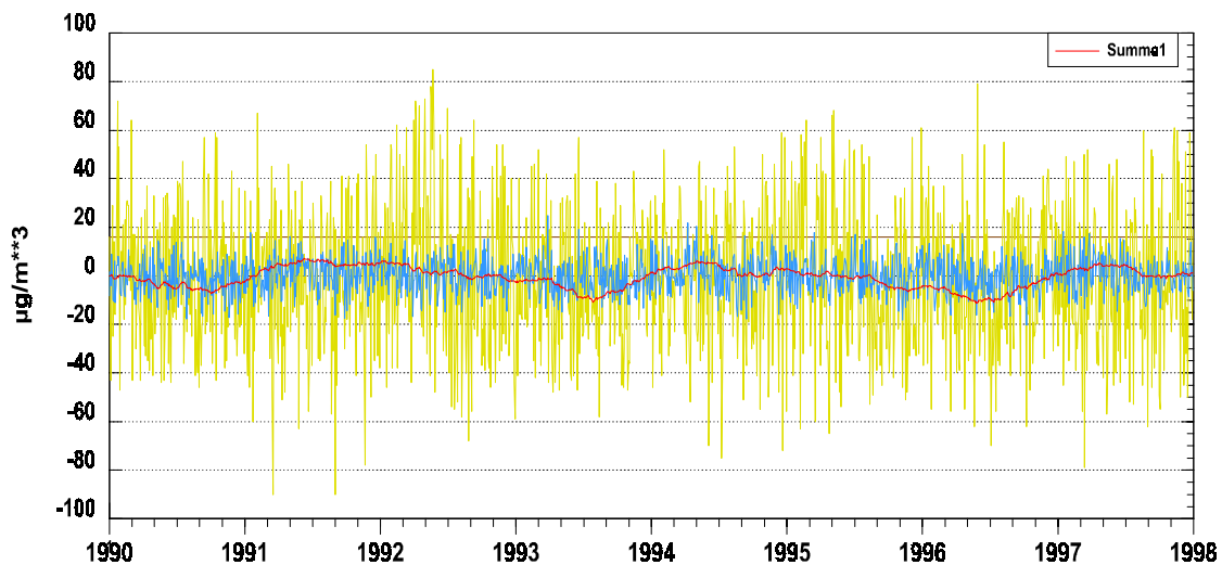
Abb. 75) Summation der Kurve II (rote Kurve = Summenkurve I)
