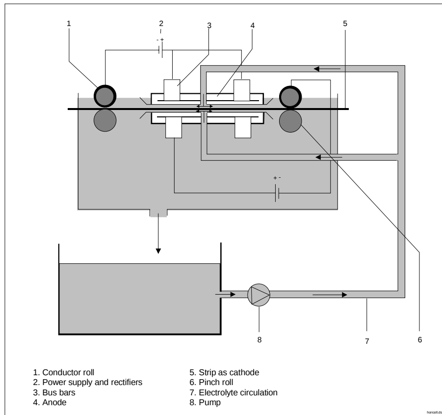
Figure B.2-7: Diagrammatic view of a horizontal cell in an electrolytic coating line
