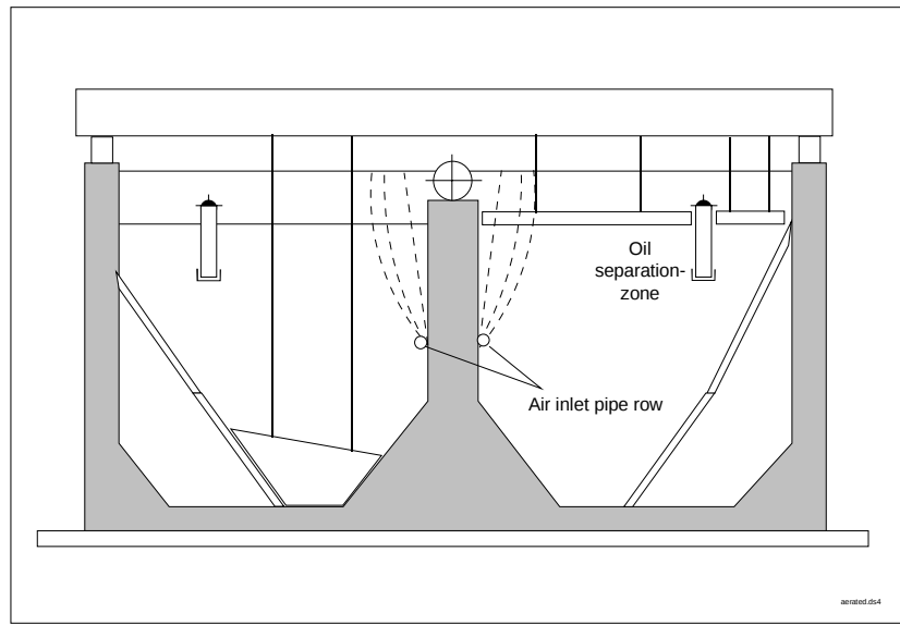
Figure A.4-7: Diagrammatic view of an aerated fine scale-trap
