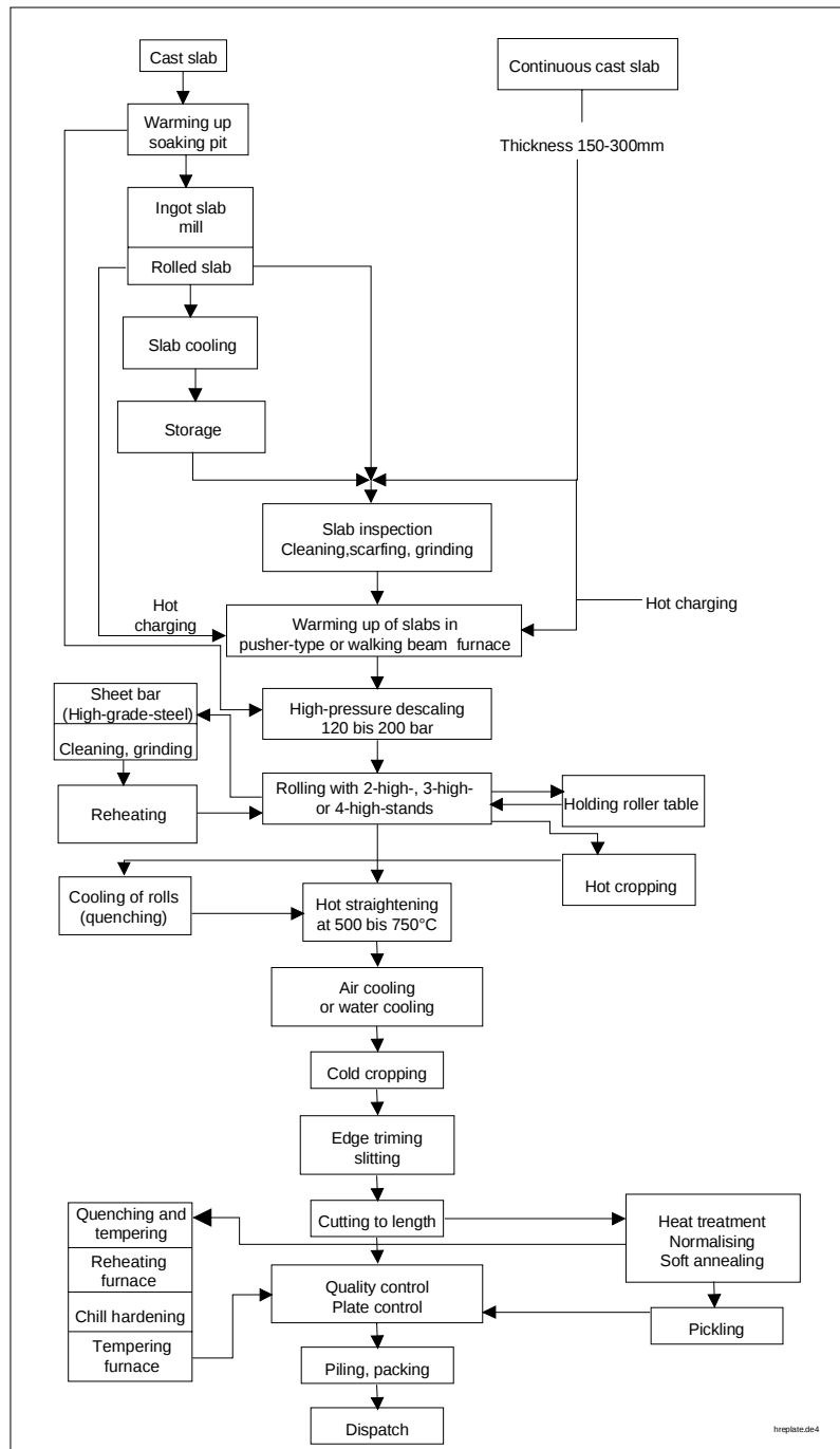
Figure A.2-5: Technological course for the production of heavy plates
