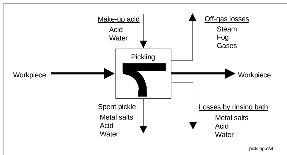
Figure A.3-2: Selected inputs and outputs of the pickling process
