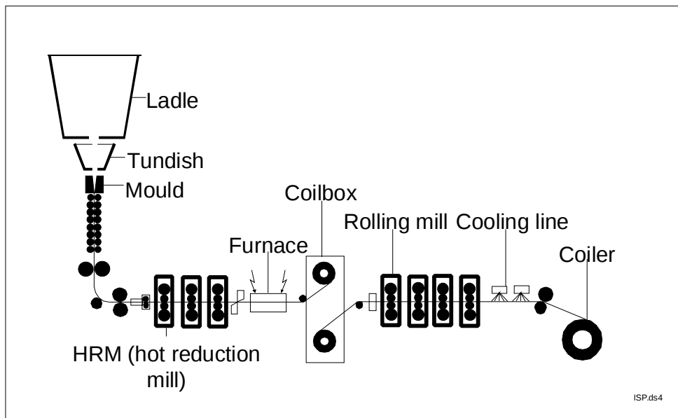
Figure A.5-4: Diagrammatic view of an ISP plant
