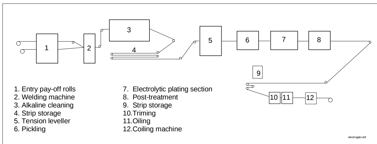
Figure B.2-5: Diagrammatic view of a continuous electro galvanising line
