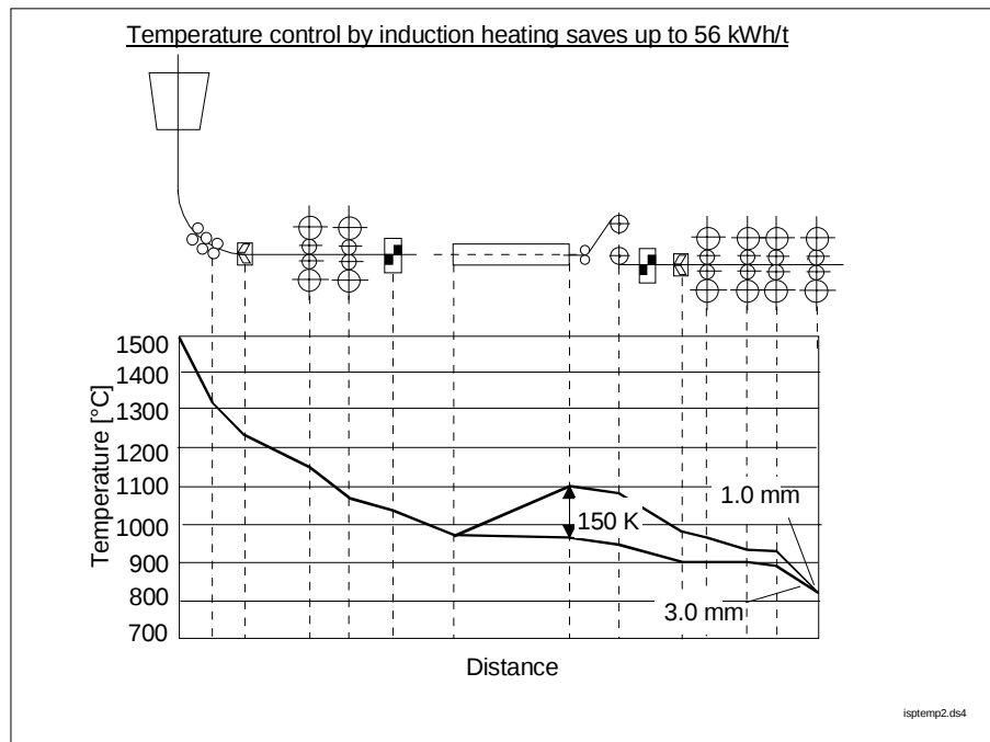
Figure A.5-5: Flexible temperature control by induction heating
