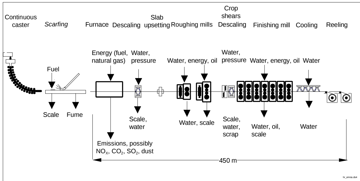
Figure A.3-1: Selected inputs / outputs of a hot strip mill
