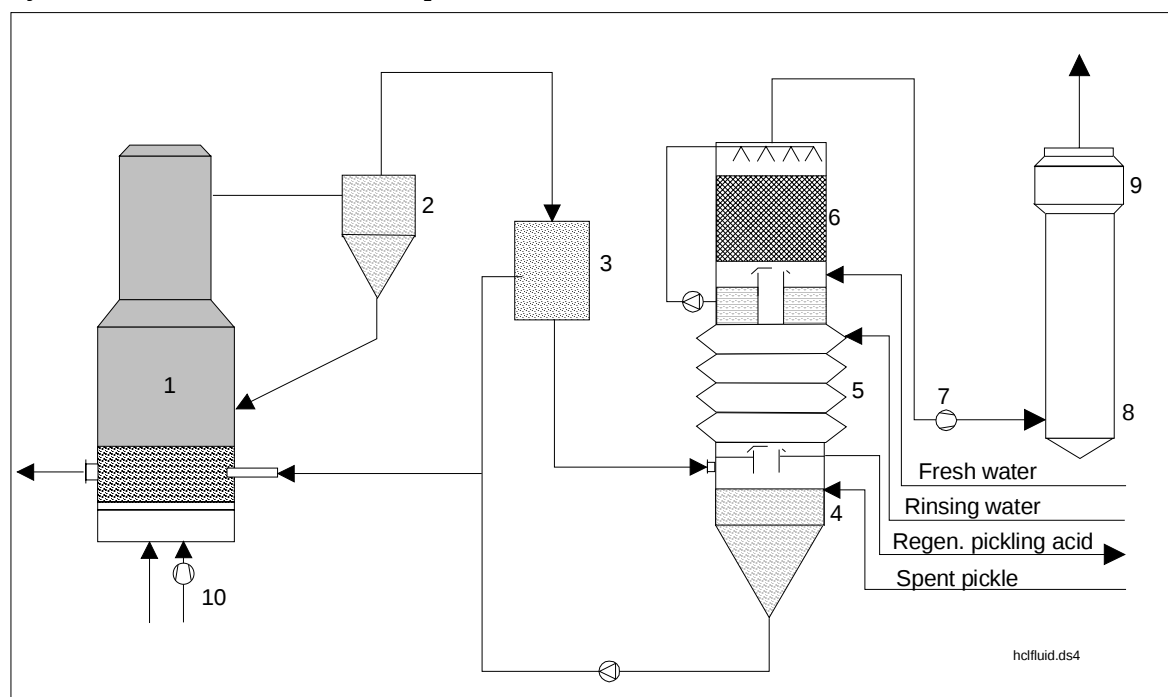
Figure A.4-12: Diagrammatic view of the fluidised bed acid regeneration process (HCl)
