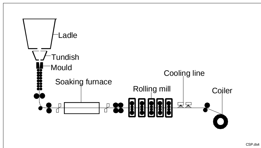
Figure A.5-2: Diagrammatic view of a CSP plant
