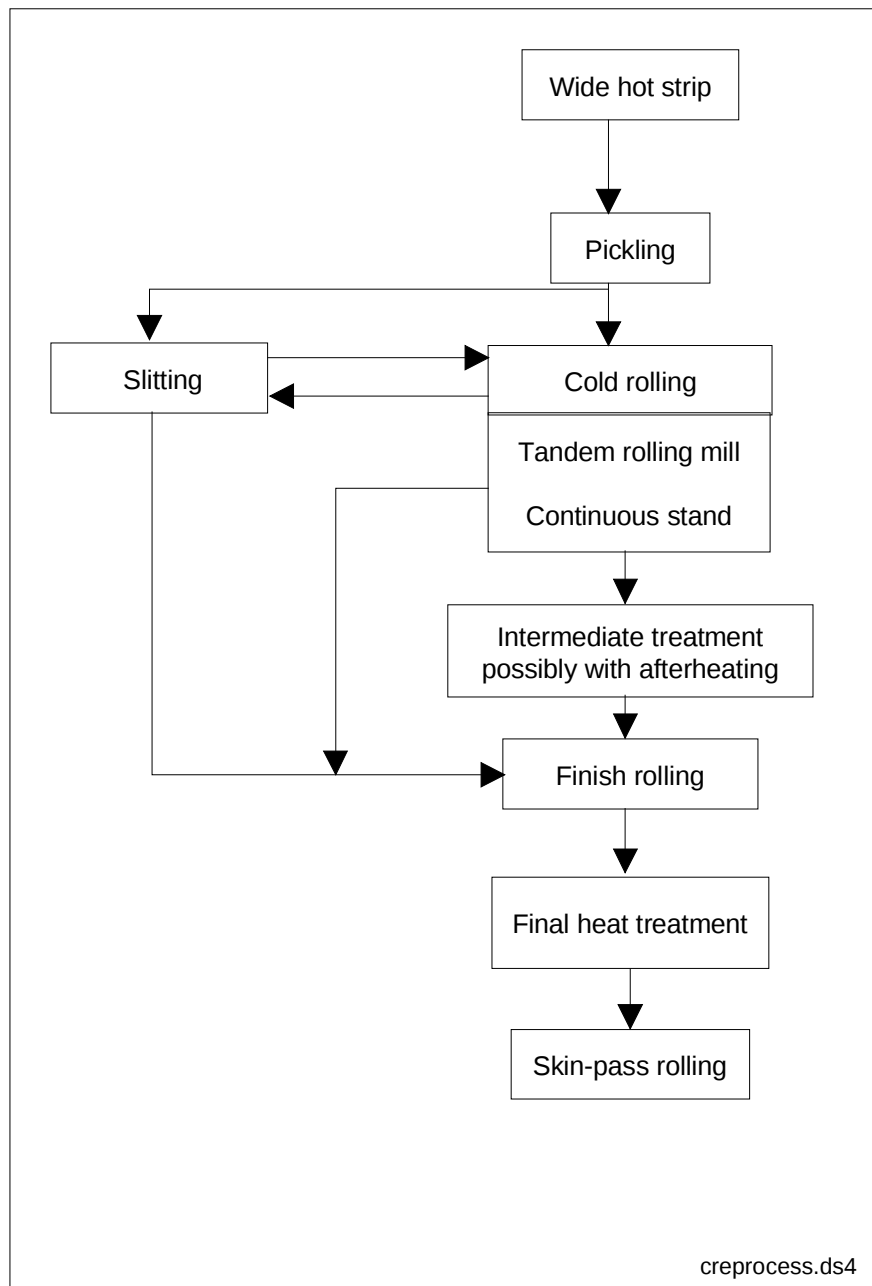
Figure A.2-6: Technological course of cold strip production
