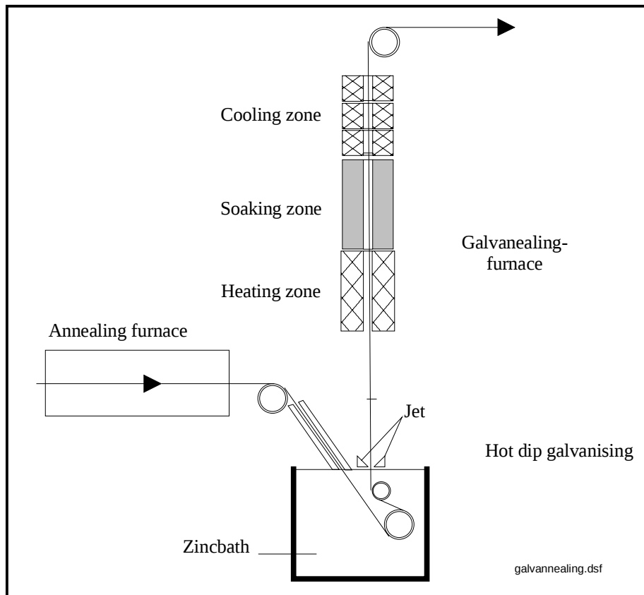
Figure B.2-4: Diagrammatic view of the coating section of a HDG line (galvannealing)
