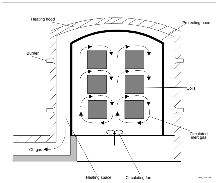
Figure A.2-10: Diagrammatic view of a hood-type annealing furnace
