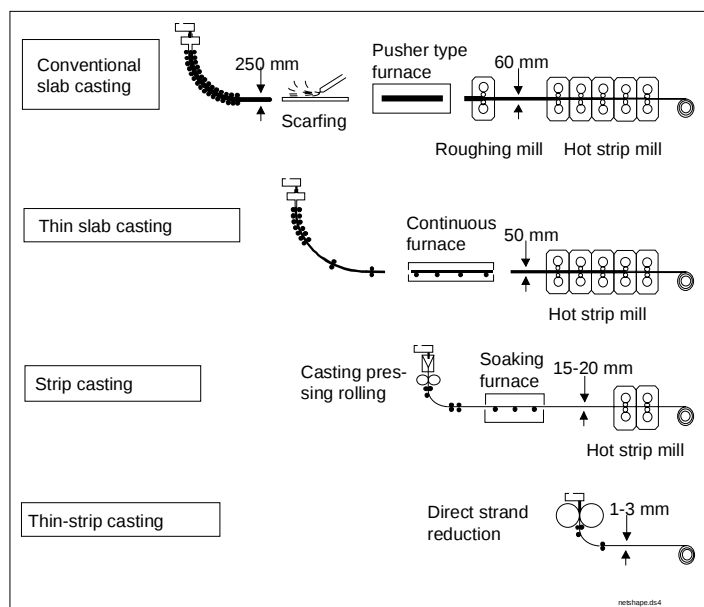
Figure A.2-3: Selected development stages of strip production
