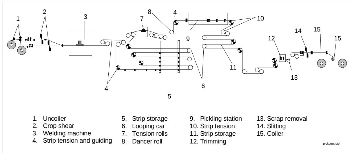
Figure A.2-7: Diagrammatic view of a continuous pickling plant
