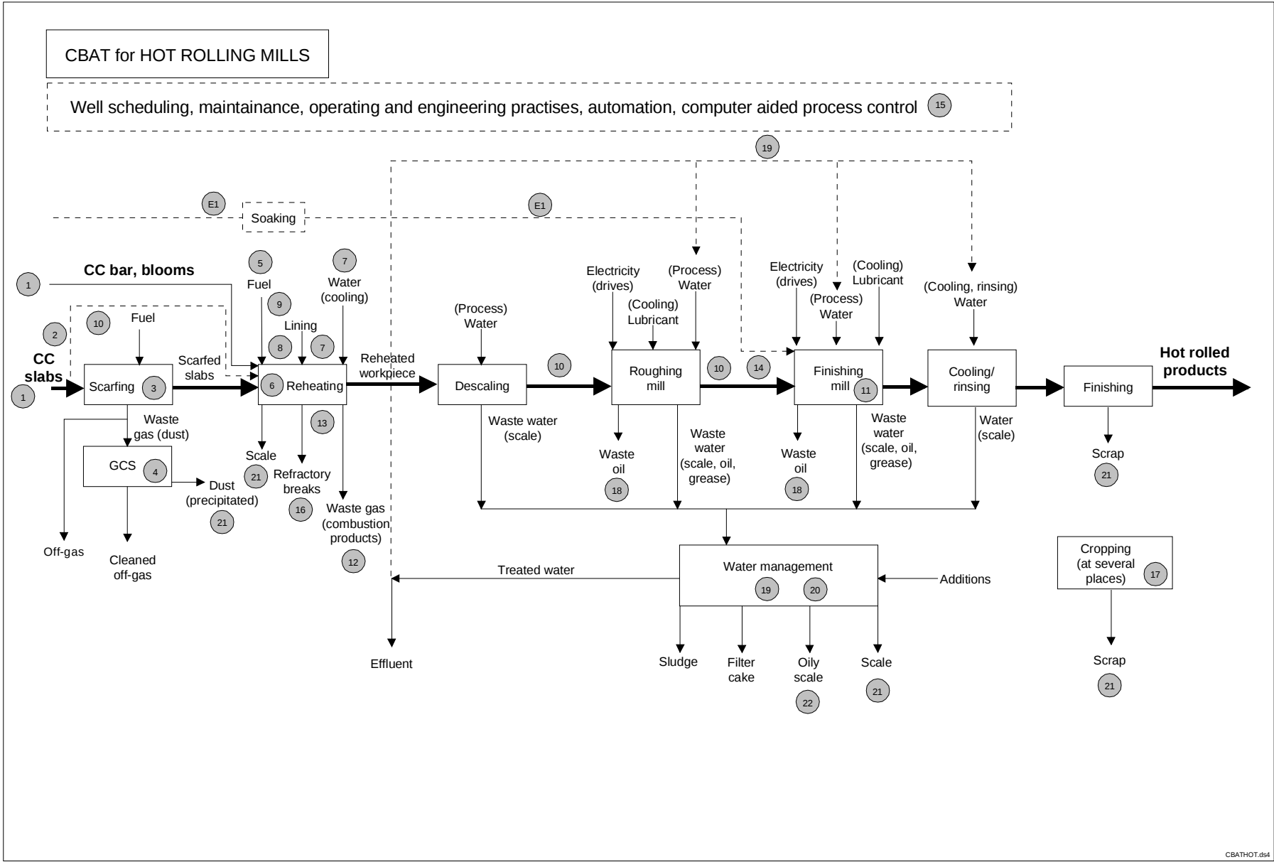
Figure A.4-9: Overview over candidate BAT for hot rolling mills
