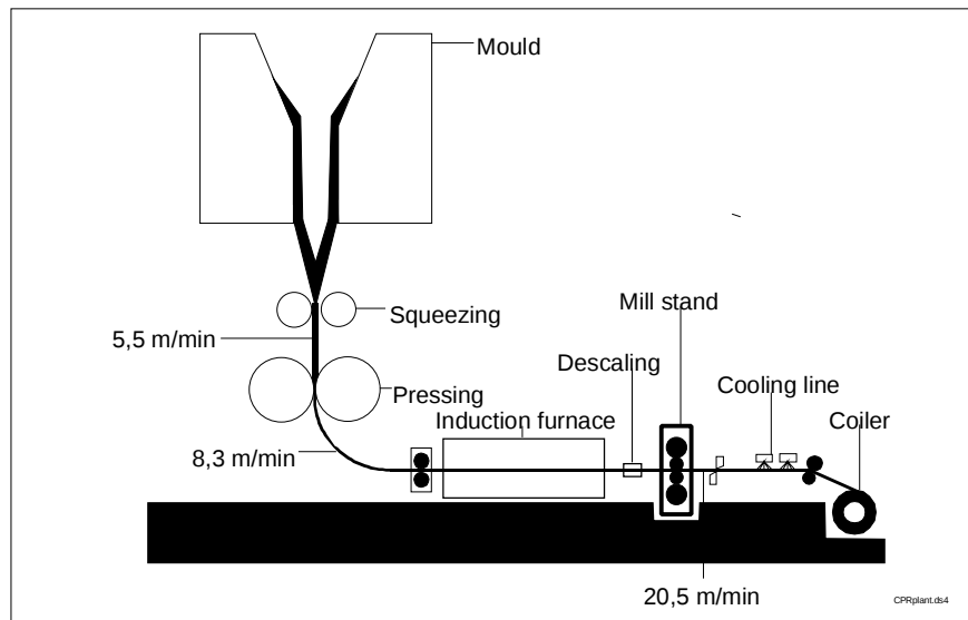
Figure A.5-10: CPR pilot plant
