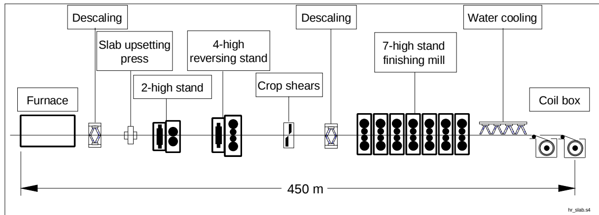
Figure A.2-4: Diagrammatic view of a wide hot strip mill
