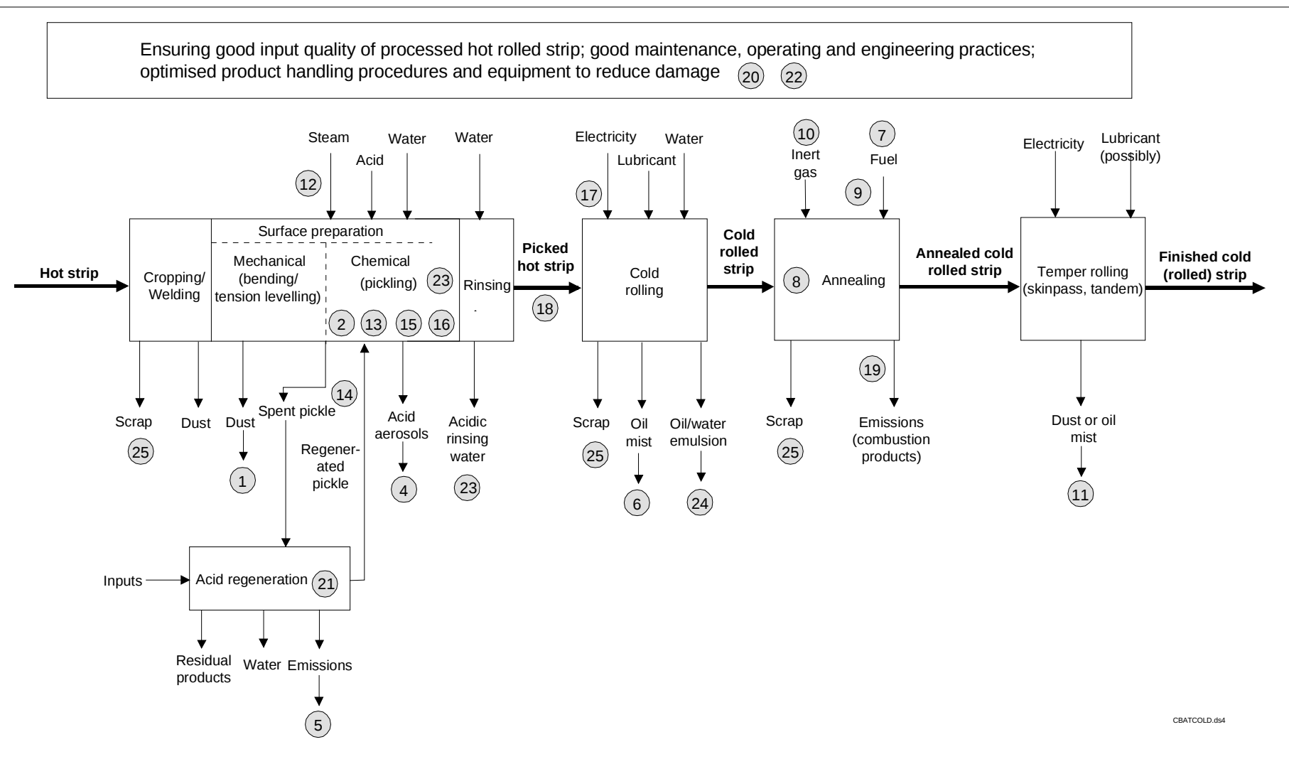
Figure A.4-18: Overview over candidate BAT for cold rolling mills
