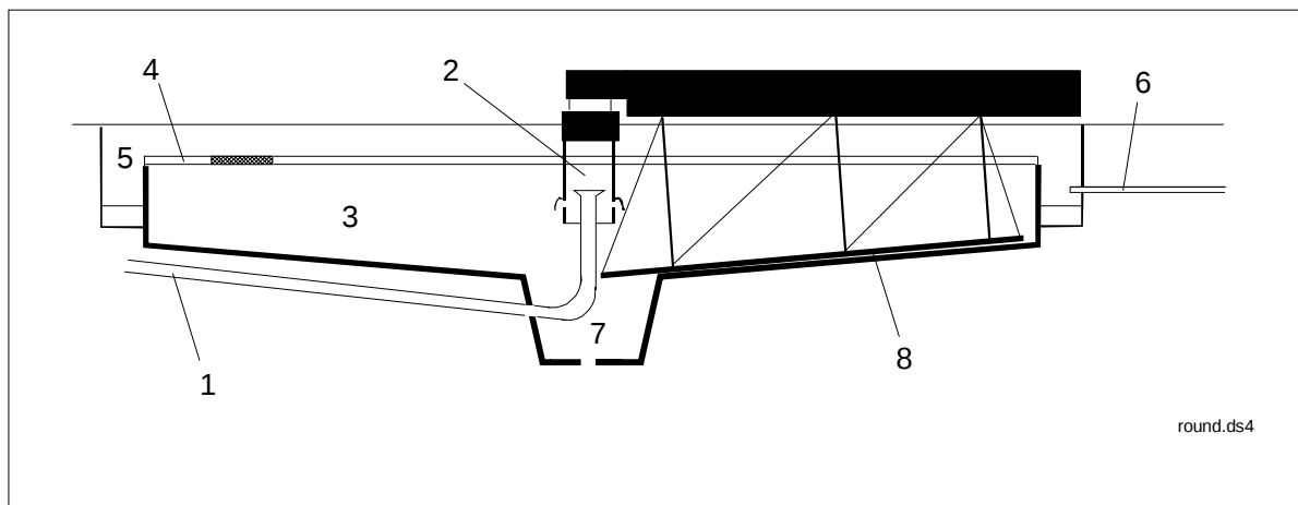
Figure A.4-5: Diagrammatic view of a circular settling tank
