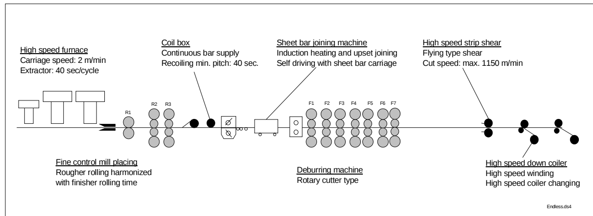
Figure A.5-1: Diagrammatic view of the endless hot strip rolling process
