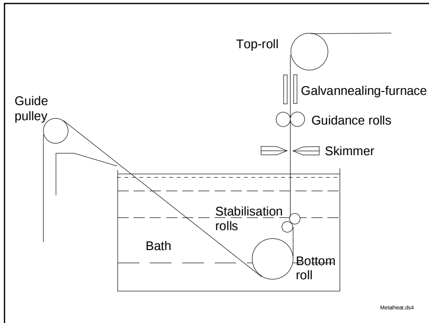
Figure B.3-5: Diagrammatic view of the metal bath of a continuous hot dip galvanising line
