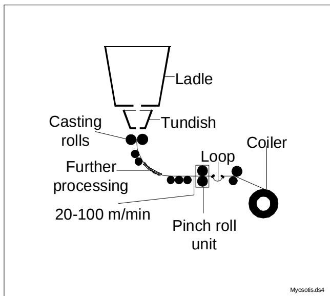
Figure A.5-9: Double-roller pilot plant
