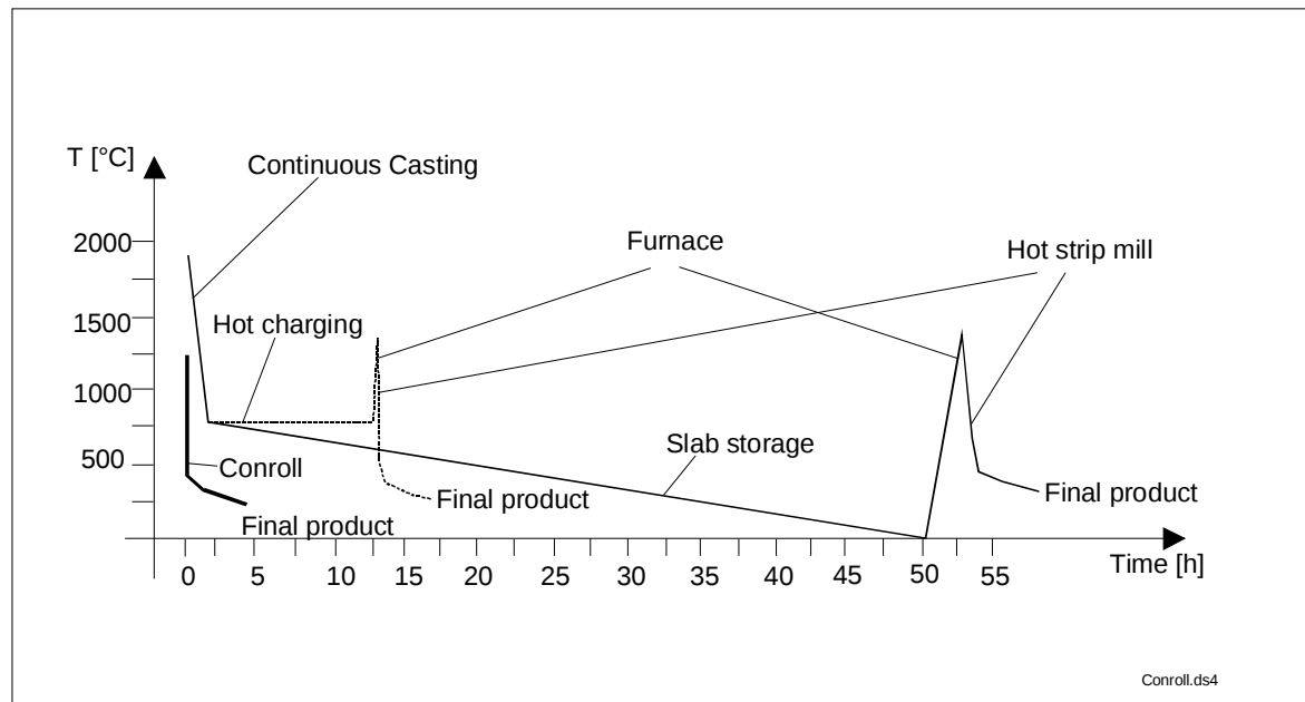
Figure A.5-8: Course of temperature and time for several plant configurations
