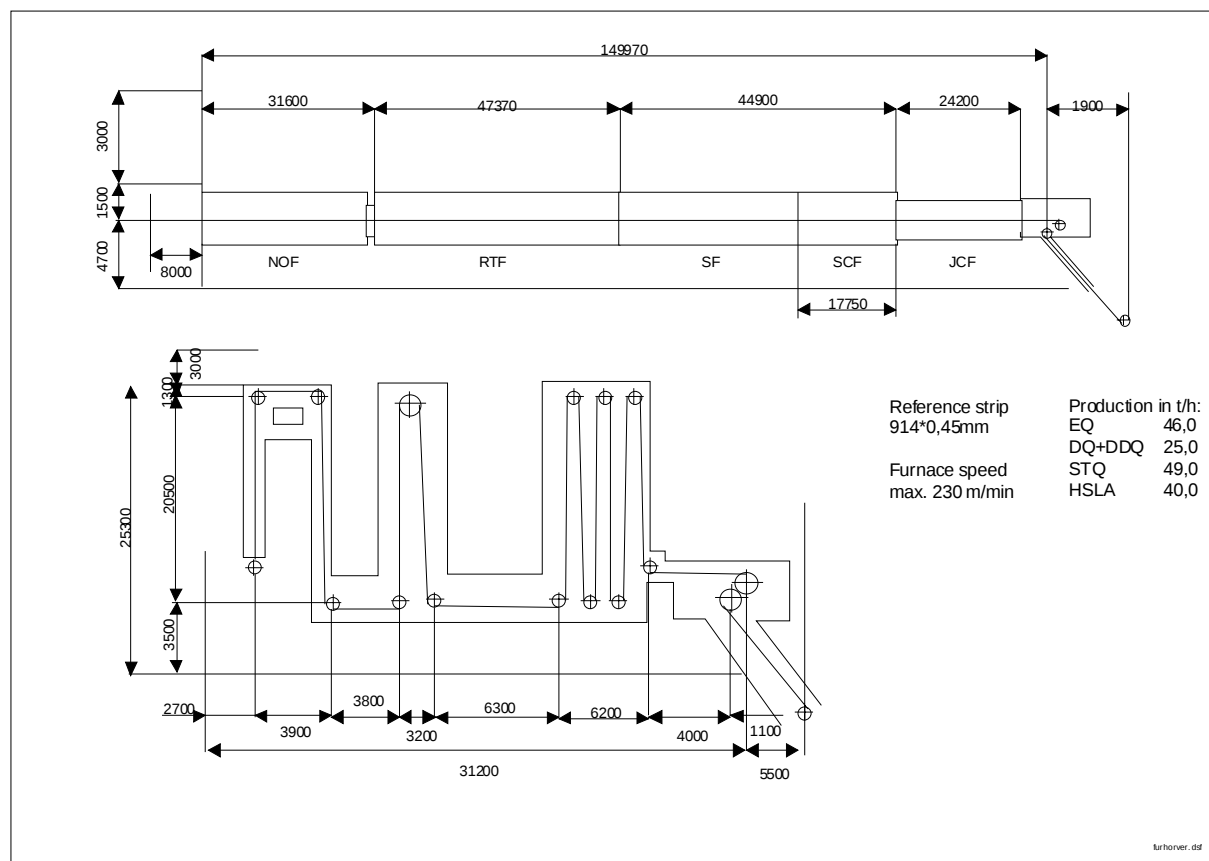
Figure B.3-3: Comparison of dimensions of a horizontal and a vertical furnace
