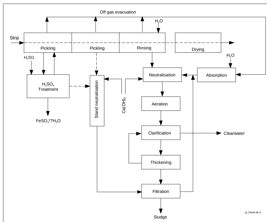
Figure A.4-16: Diagrammatic view of a pickling plant using \text{H}_2\text{SO}_4
