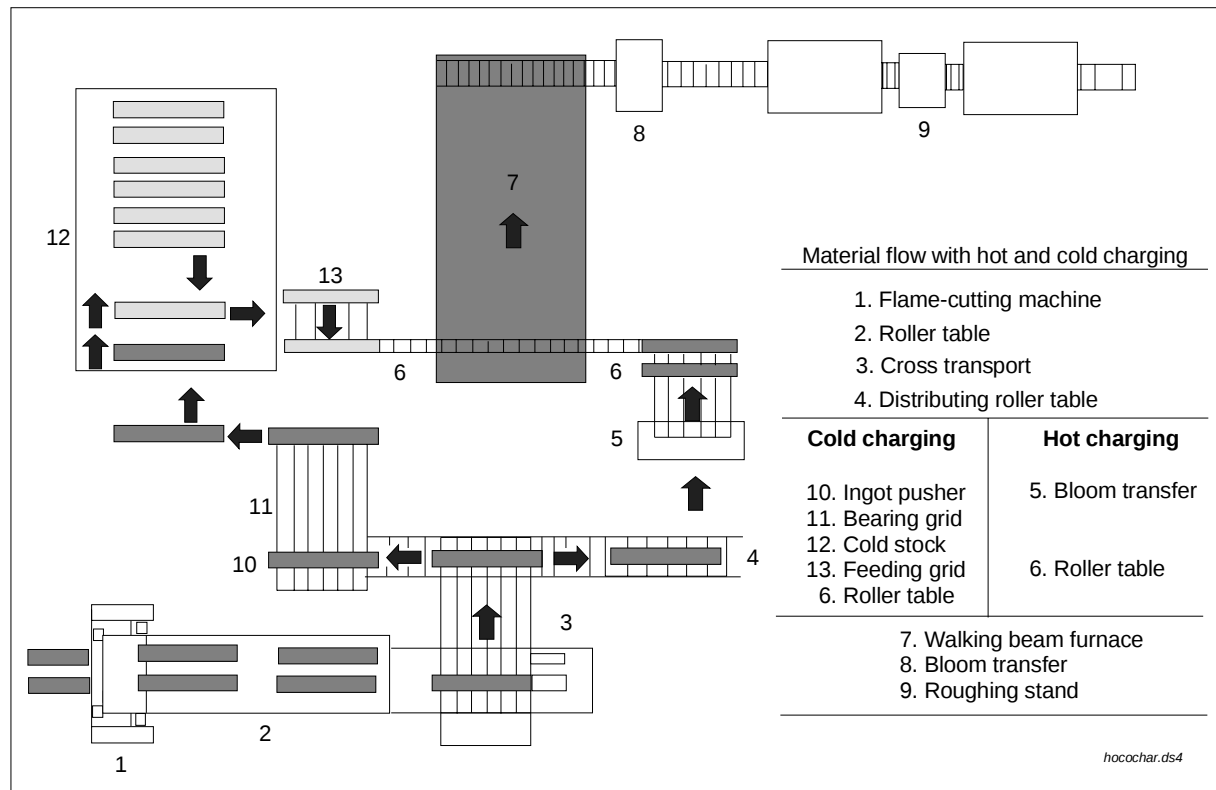
Figure A.4-2: Material flow: cold versus hot charging
