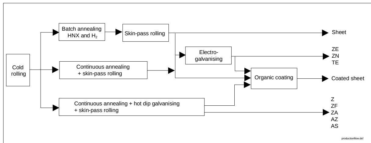
Figure B.2-1: Routes of production for coated sheets
