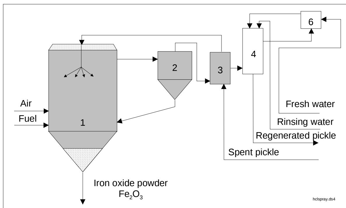
Figure A.4-13: Diagrammatic view of the spray roasting acid regeneration process (HCl)
