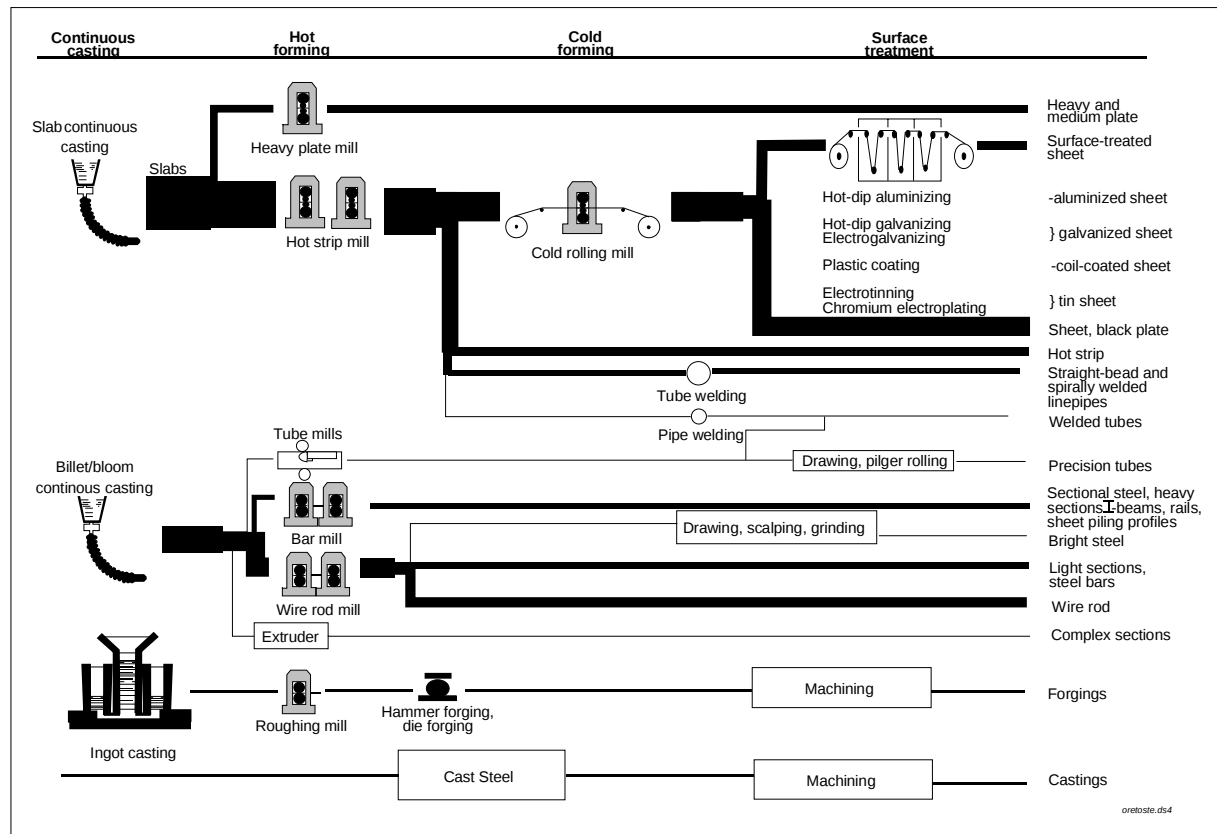
Figure A.2-1: Flow of liquid steel from continuous casting via rolling mills to final products
