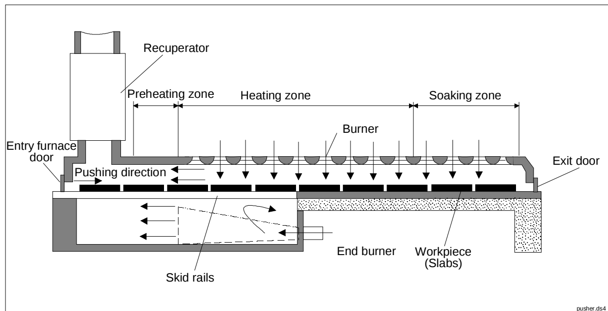
Figure A.4-1: Diagrammatic view of a pusher-type furnace
