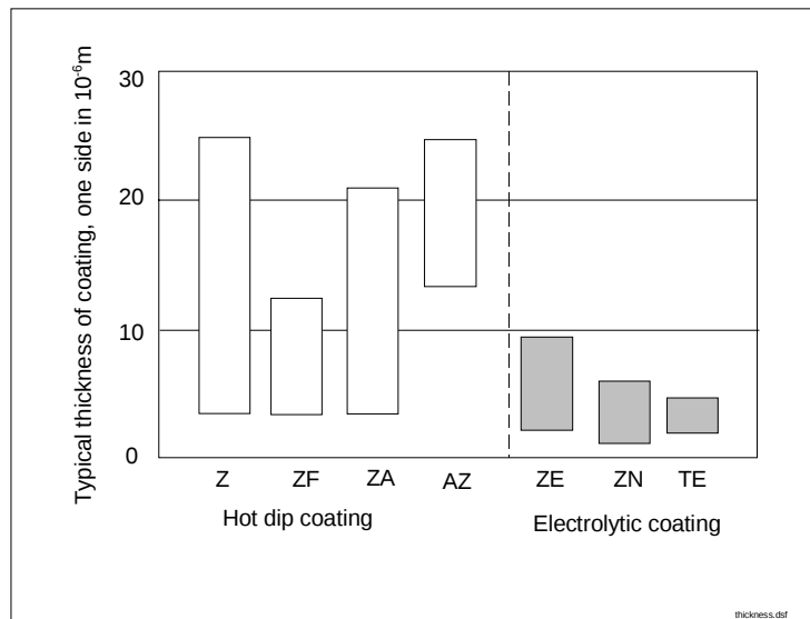
Figure B.2-2: Thickness of metallic coatings
