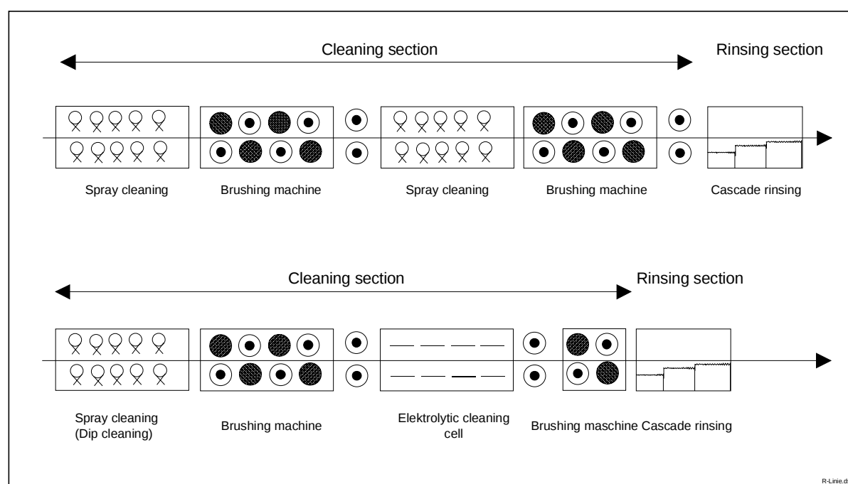
Figure B.3-1: Diagrammatic view of different types of cleaning lines
