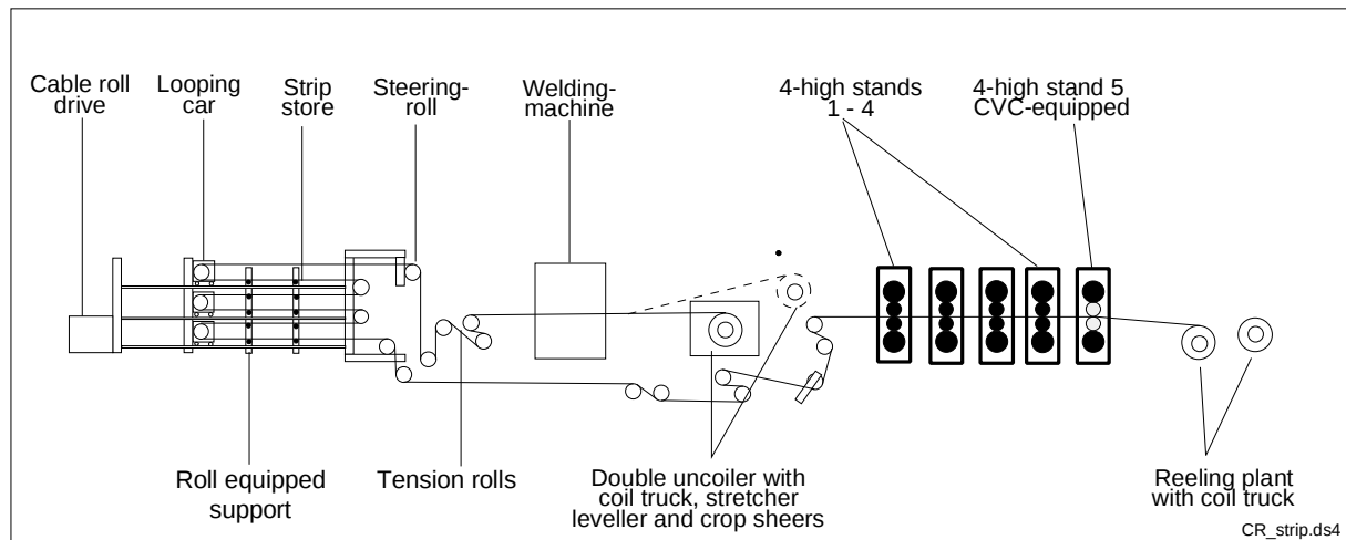
Figure A.2-8: Diagrammatic view of a continuous cold rolling mill
