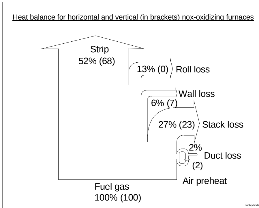
Figure B.3-4: Heat balance for non-oxidising furnaces
