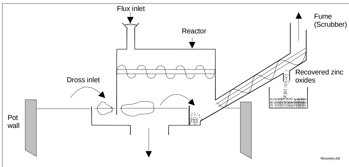
Figure B.3-6: Diagrammatic view of a recovery system for zinc from dross
