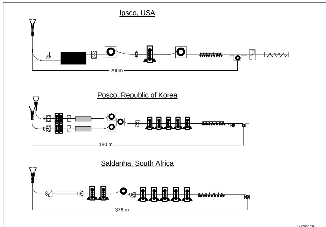
Figure A.5-7: Different plant concepts using the ISP technology
