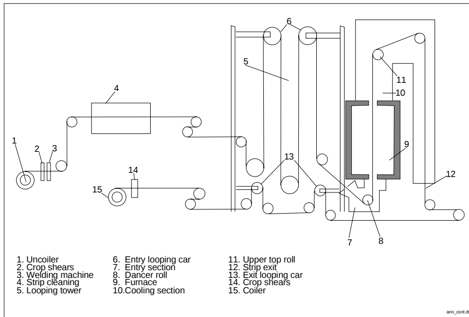
Figure A.2-9: Diagrammatic view of a continuous annealing furnace
