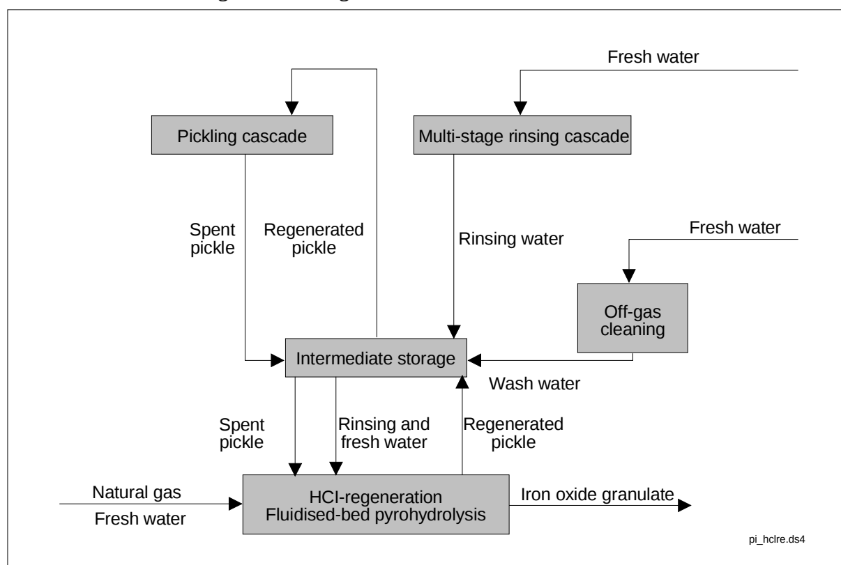
Figure A.4-15: Recycling loop for HCl-pickling plant
