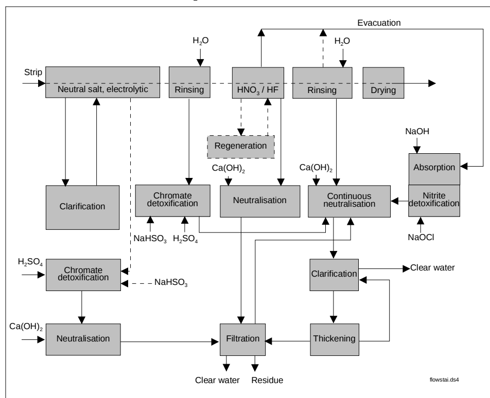
Figure A.4-17: Diagrammatic view of a stainless steel strip pickling plant
