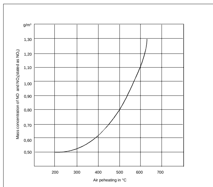
Figure C.1-1: NOx emission limits TA Luft
