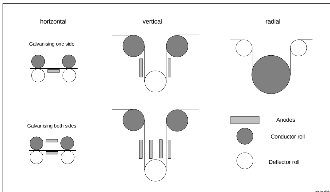
Figure B.2-6: Diagrammatic view of different cell types for electrolytic coating lines
