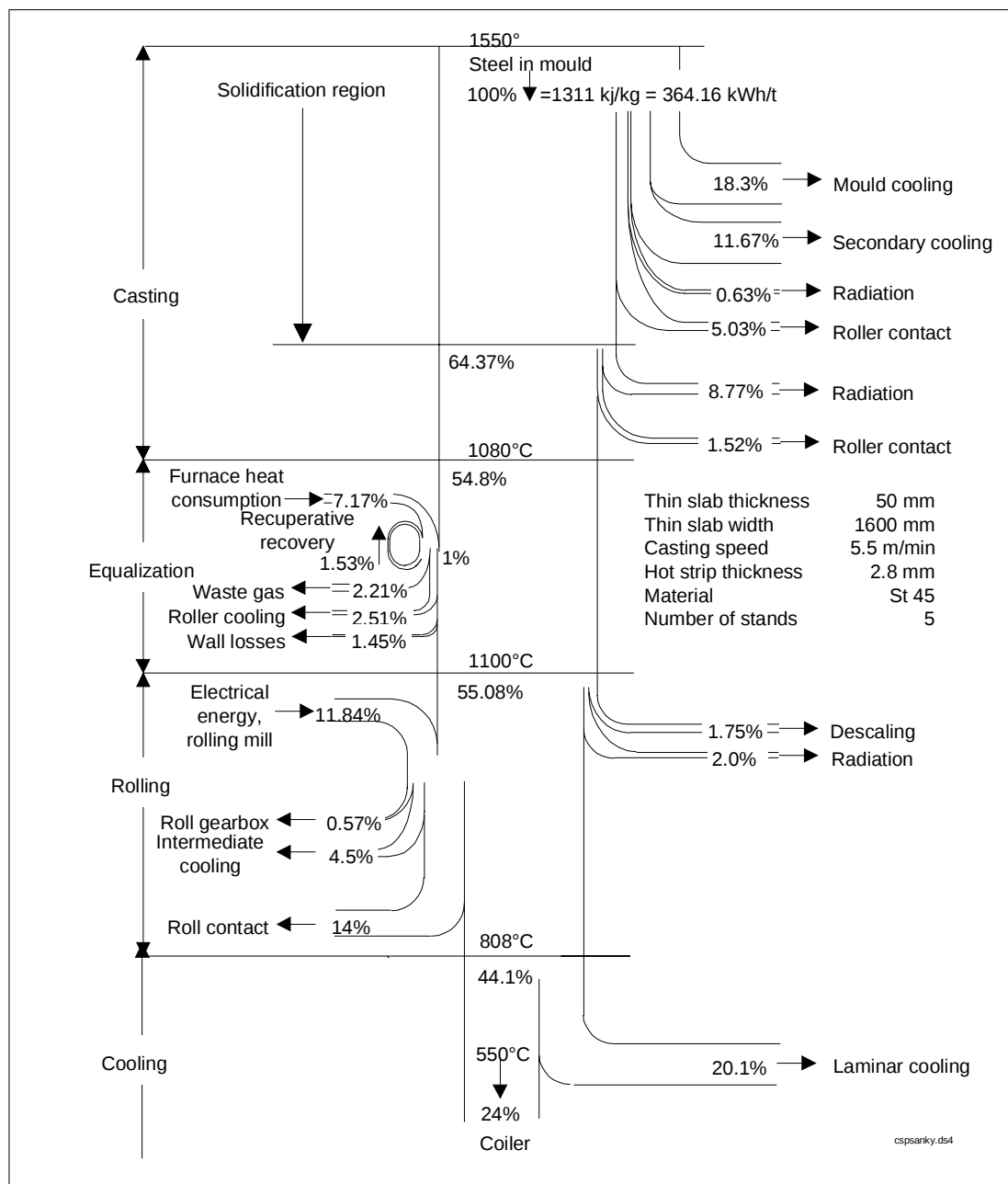
Figure A.5-3: Energy balance for a single-strand CSP plant
