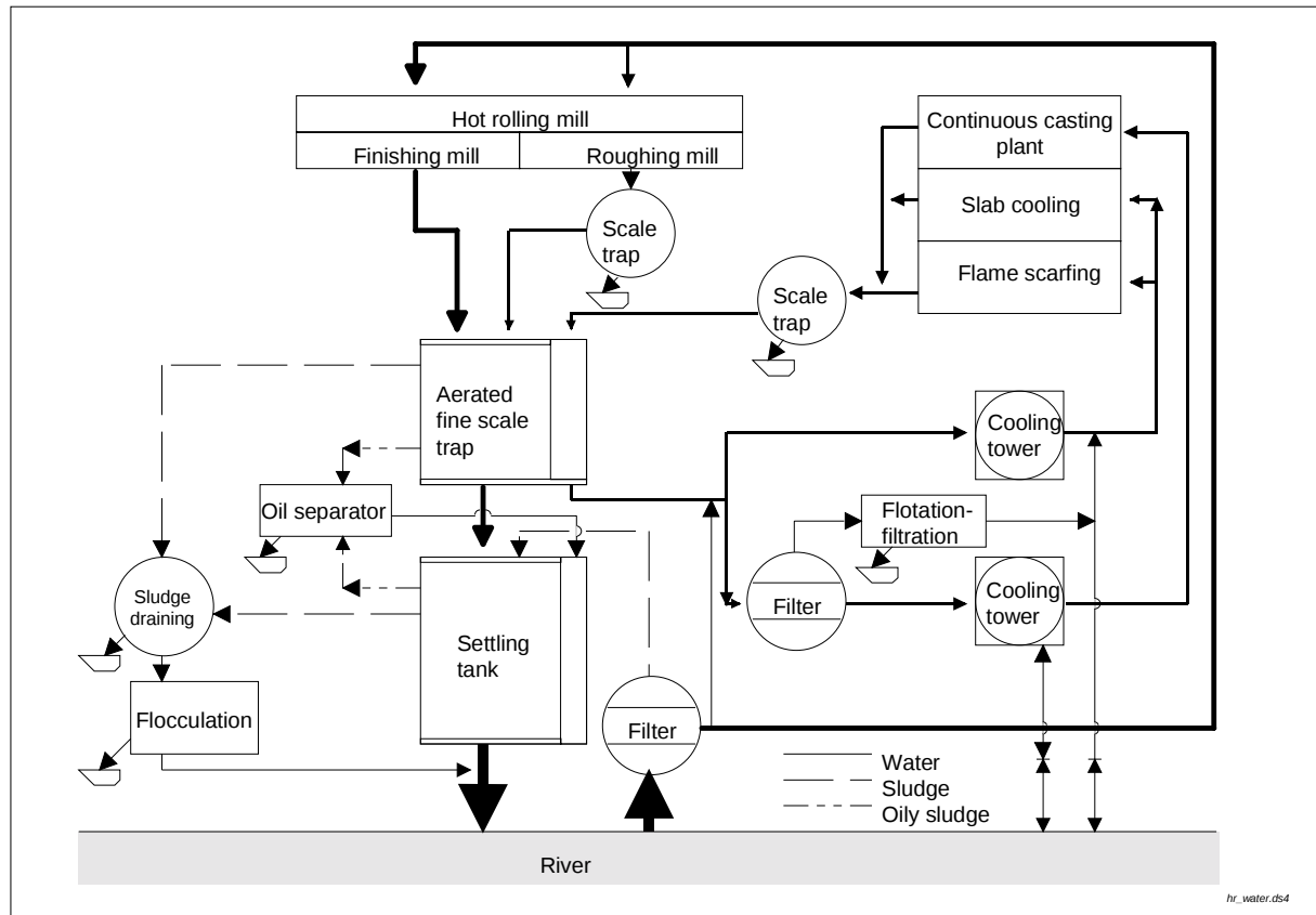
Figure A.4-4: Diagrammatic view of water loops in a hot strip mill
