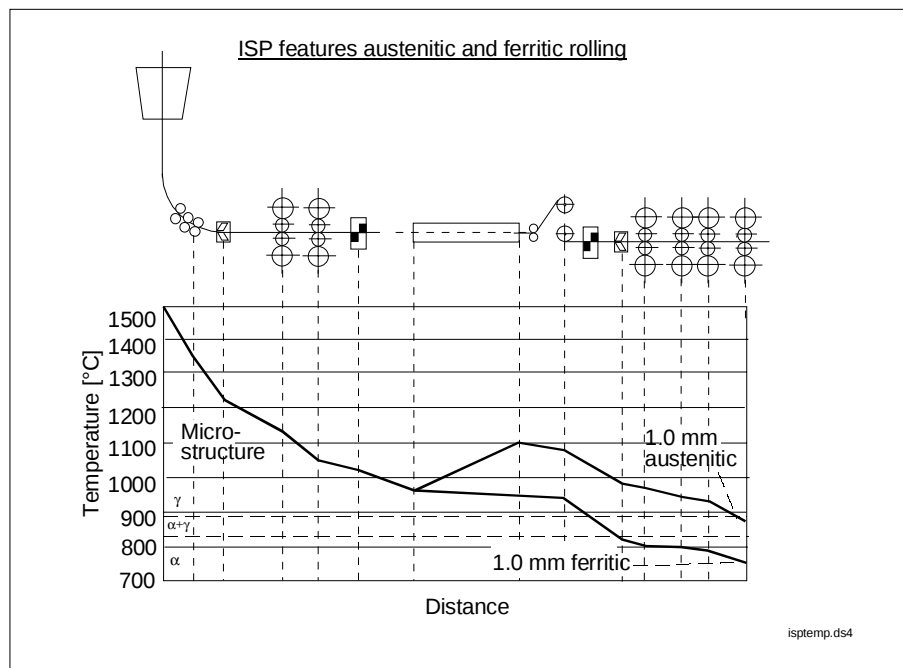
Figure A.5-6: Flexible temperature control yields new rolling technologies
