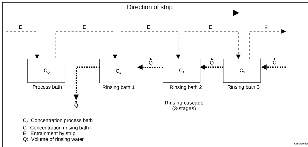
Figure B.3-2: Diagrammatic view of a cascade rinsing system
