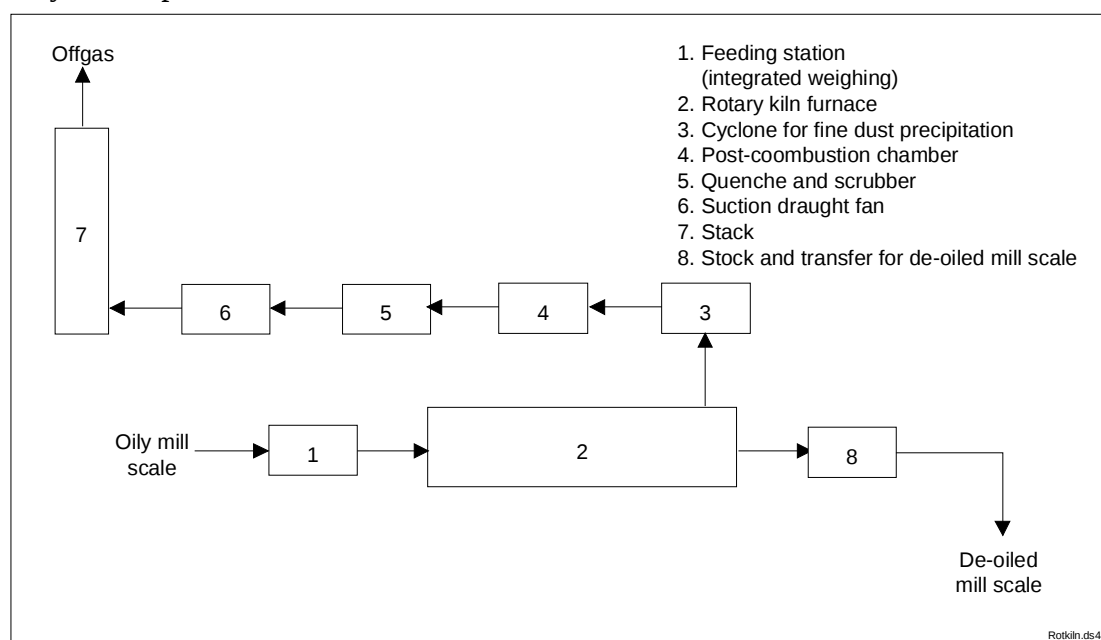
Figure A.4-8: Diagrammatic view of an oily mill scale treatment plant
