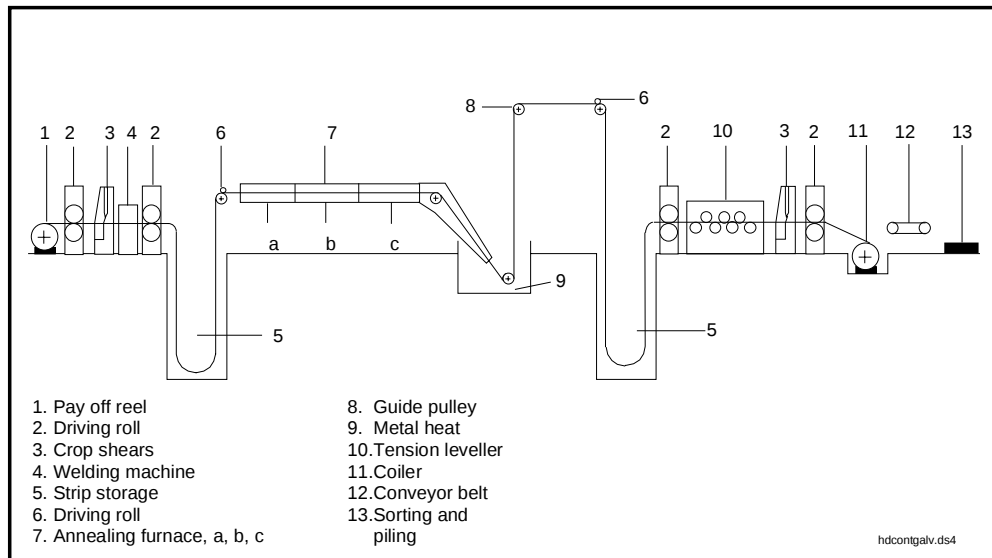
Figure B.2-3: Diagrammatic view of a continuous hot dip galvanising line
