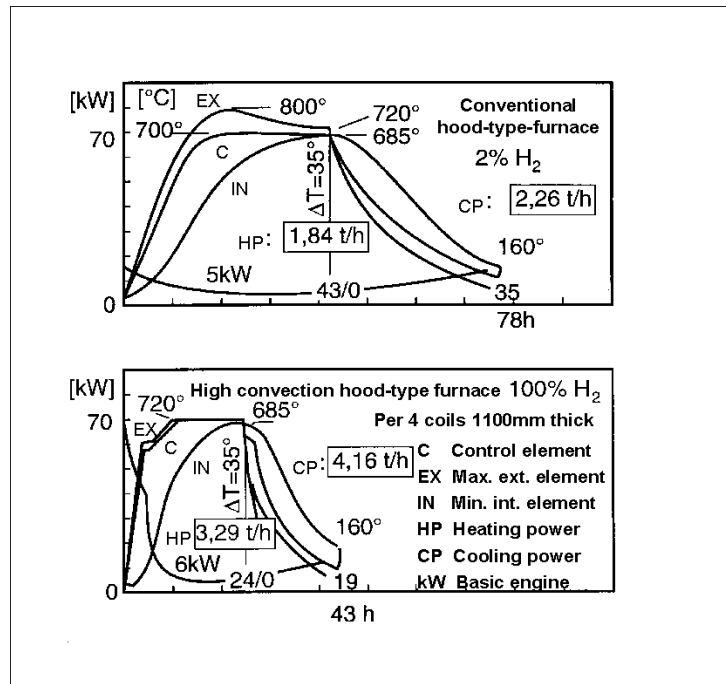
Figure A.4-11: Comparison of hood-type annealing furnaces (course of power and temperature / time)
