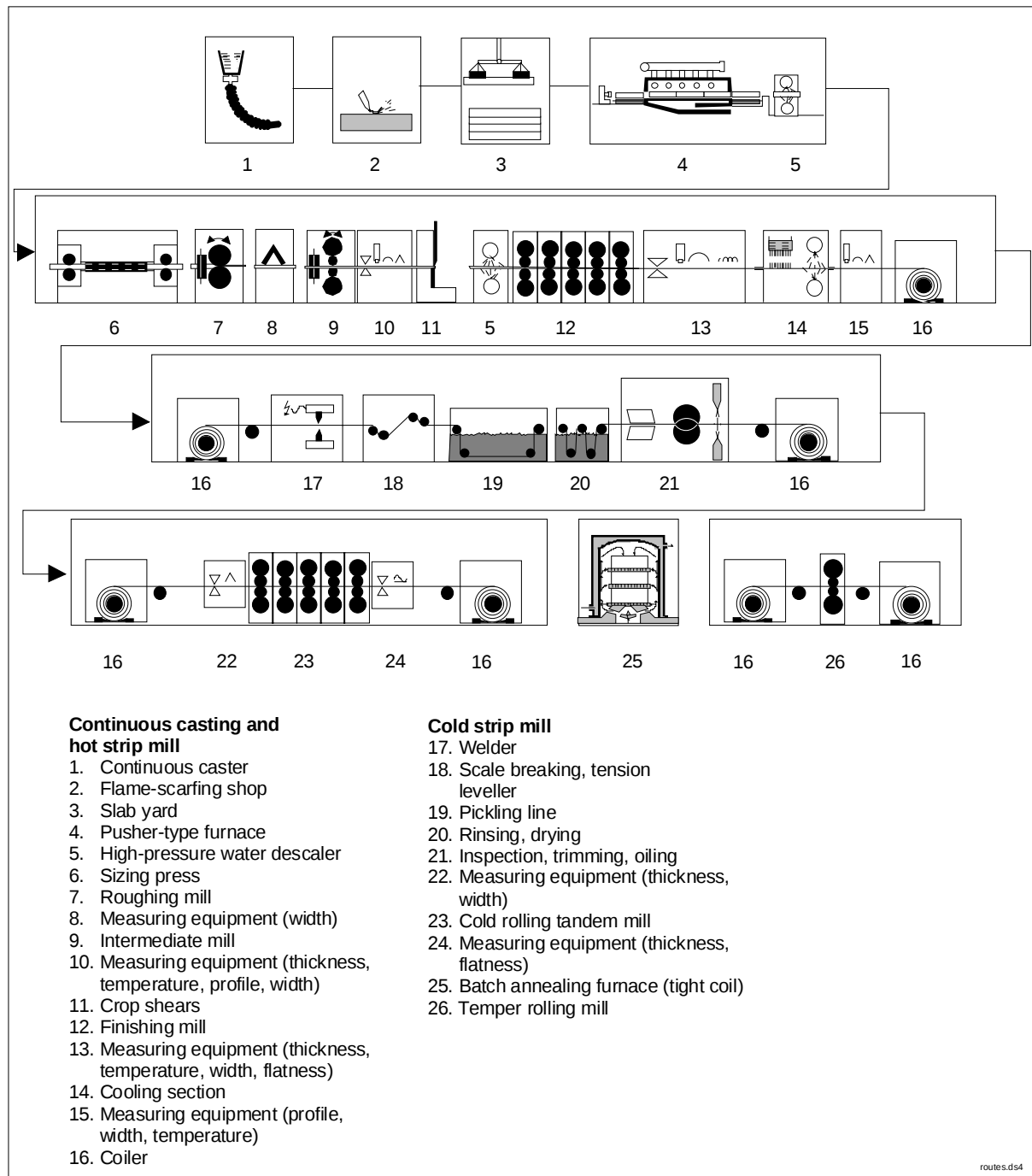
Figure A.2-2: Overview of processes from continuous casting to cold strip mill
