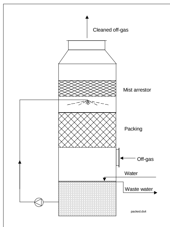
Figure A.4-10: Diagrammatic view of a packed scrubber for absorptive gas cleaning
