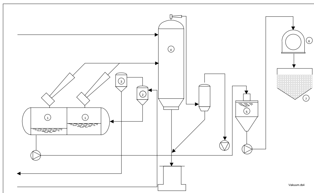
Figure A.4-14: Diagrammatic view of the vacuum cooling crystallisation process ( \text{H}_2\text{SO}_4 )
