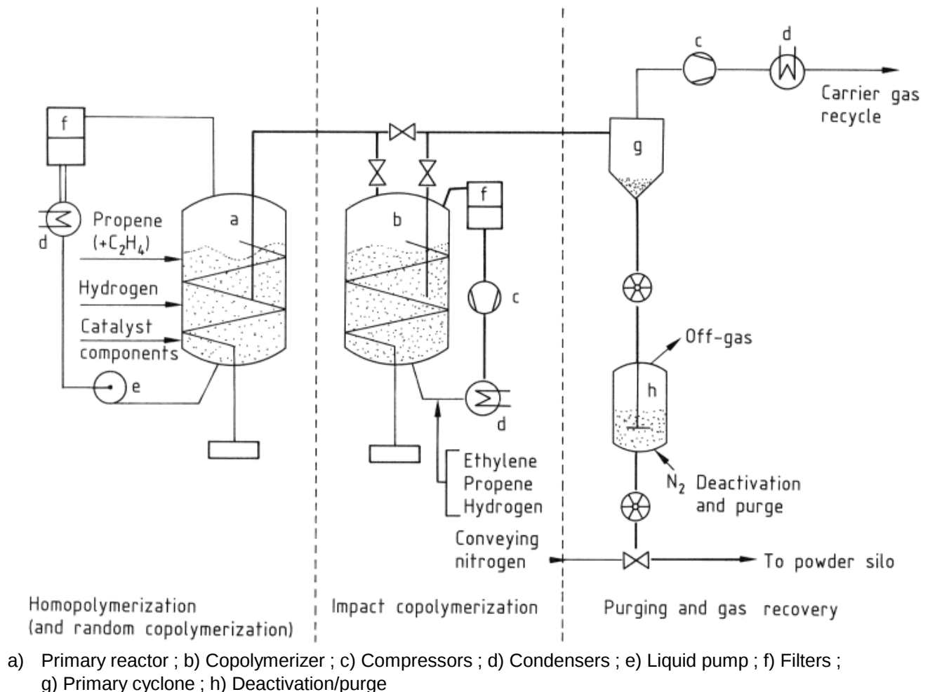
Figure 8.6: Process flow chart for a gas phase process to produce iPP according to the BASF process /2/
