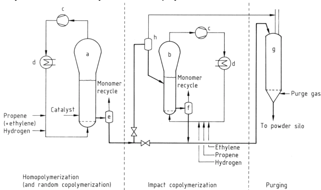
Figure 8.5: Process flow chart for a gas phase process to produce iPP in a fluidized bed according to the Unipol process /2/
