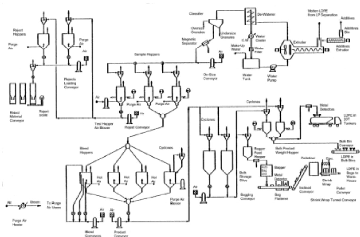
Figure 6.4: Flow chart for PE-LD extrusion and packaging /3/
