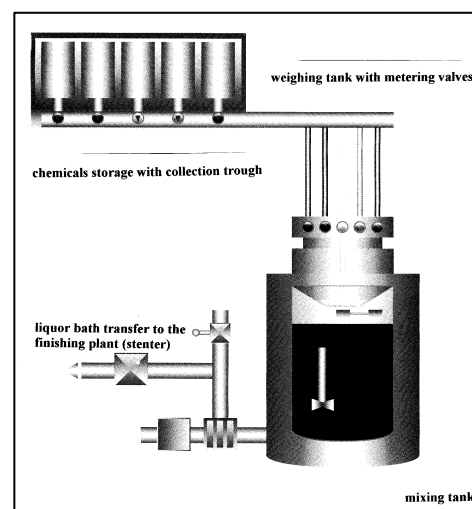
Figure 4.4: Example for the on-line preparation equipment of padding liquor for the finishing of woven and knit fabric (pictures from Mutschink GmbH, D-47918 Tönisvorst)
