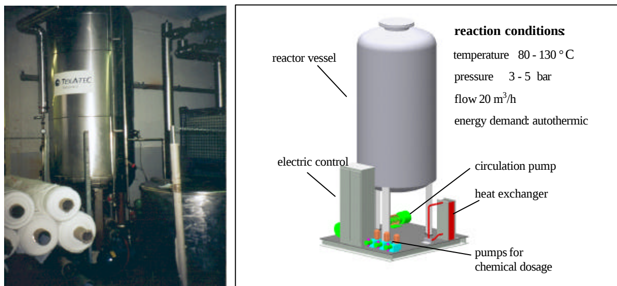
Figure 4.57: Picture and principle scheme for treatment of selected, segregated high-loaded textile wastewater streams by catalytic oxidation with Q/H 2 O 2 and picture of the reactor at Schoeller AG, CH-Sevelen which is in operation since 1996
