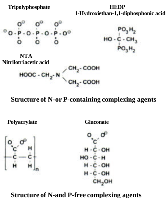
Figure 4.9: Chemical structure of complexing agents [Bachus, 1999]
