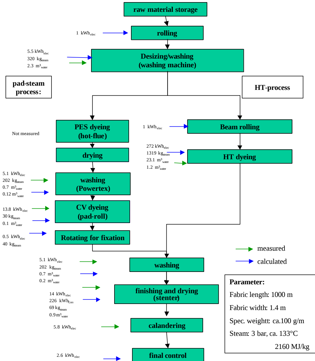
Figure 3.10: Distribution of thermal and electric energy consumption for the finishing of viscose/polyester fabric- [Eutech/ITA/LTT, 2000]
