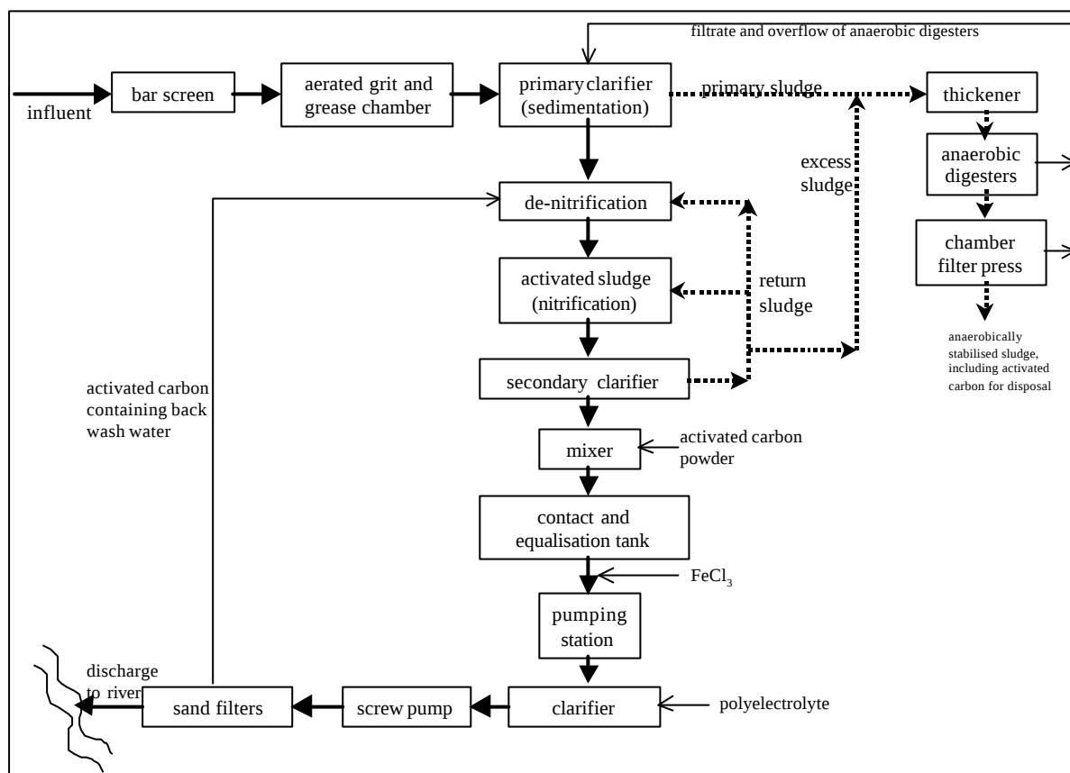
Figure 4.49: Plant 6 - combined treatment of textile wastewater and municipal wastewater
