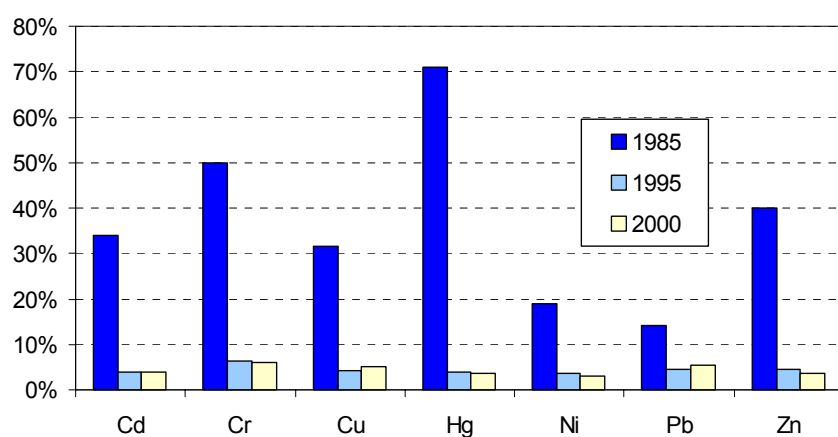
Figure 6-11 Changes of the share of direct industrial discharges in the total emissions of the years 1985-2000.
