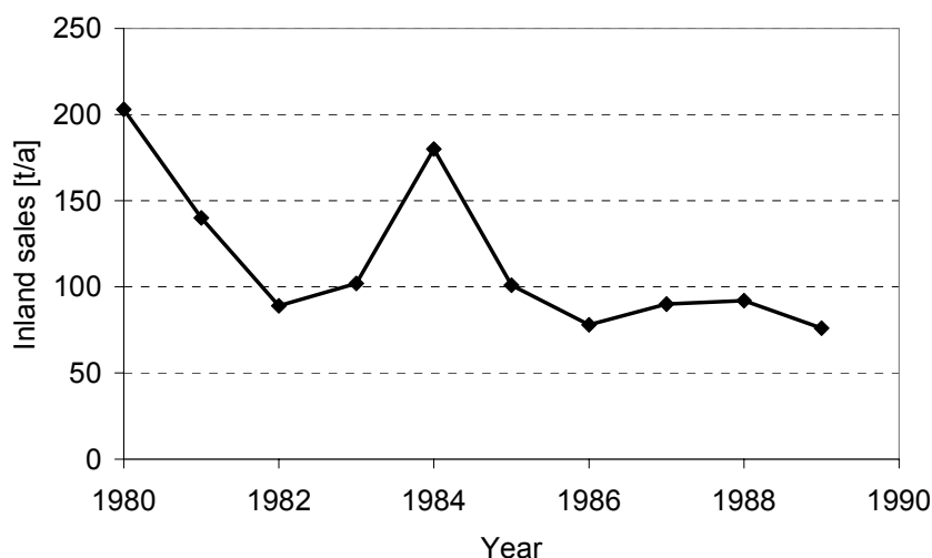
Figure 4-1 Lindane sales volume in the former GDR between 1980-1989 (Schmidt, 1993).
