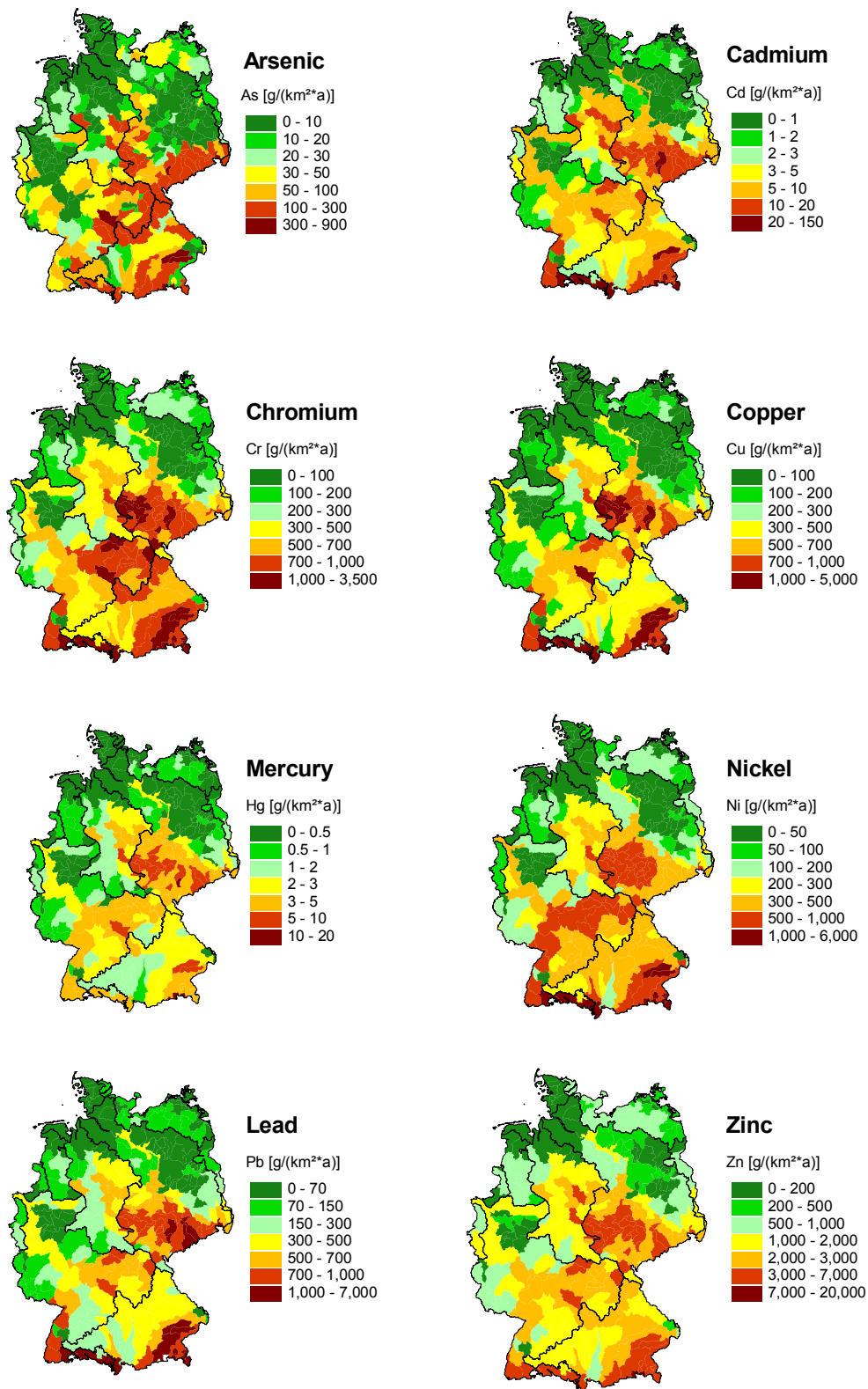
Figure 6-15 Distribution of heavy metal emissions by erosion.
