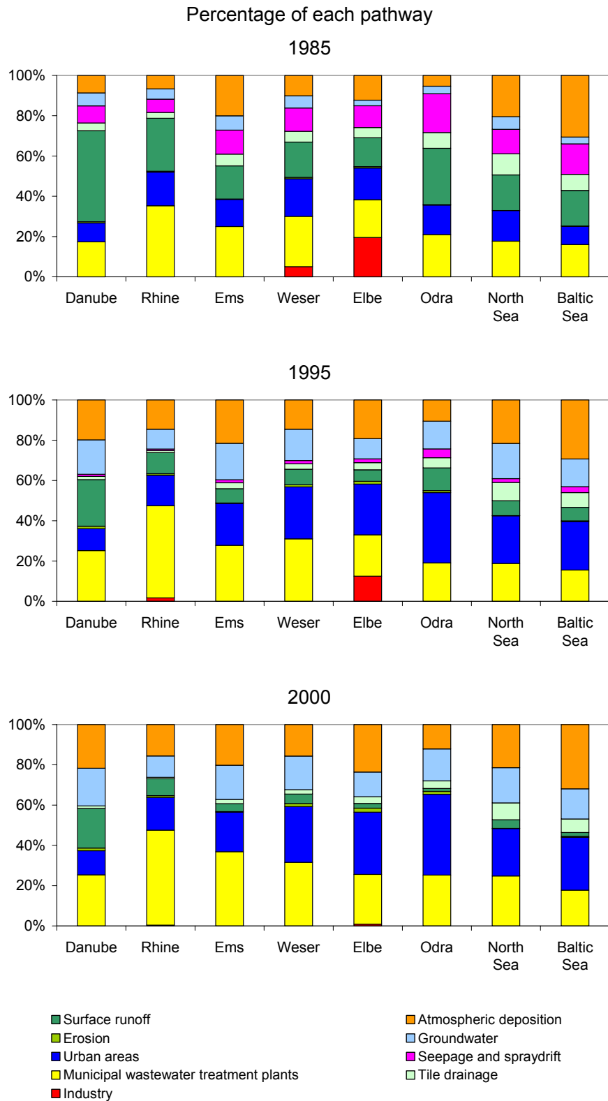
Figure 7-1 Lindane emissions into German river basins.
