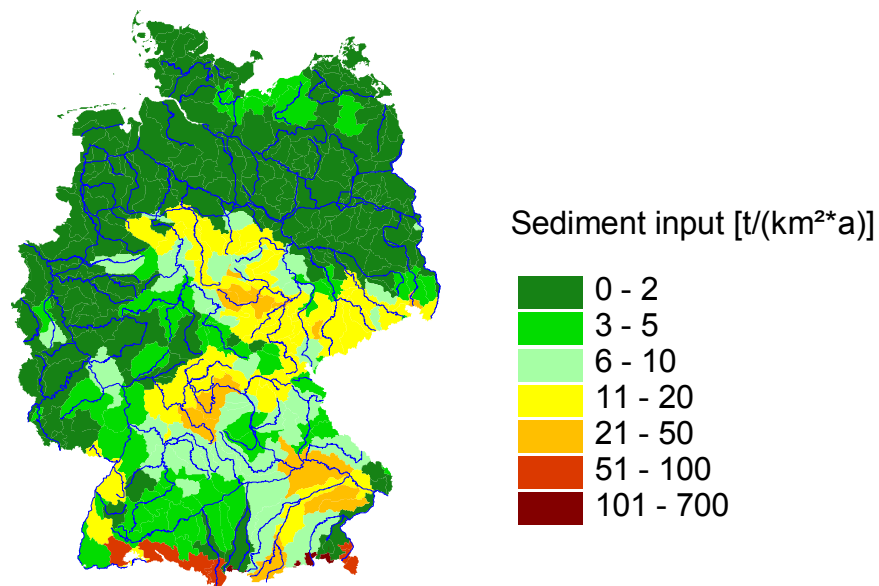
Figure 3-4 Specific sediment input in German river systems obtained from MONERIS for 1995.
