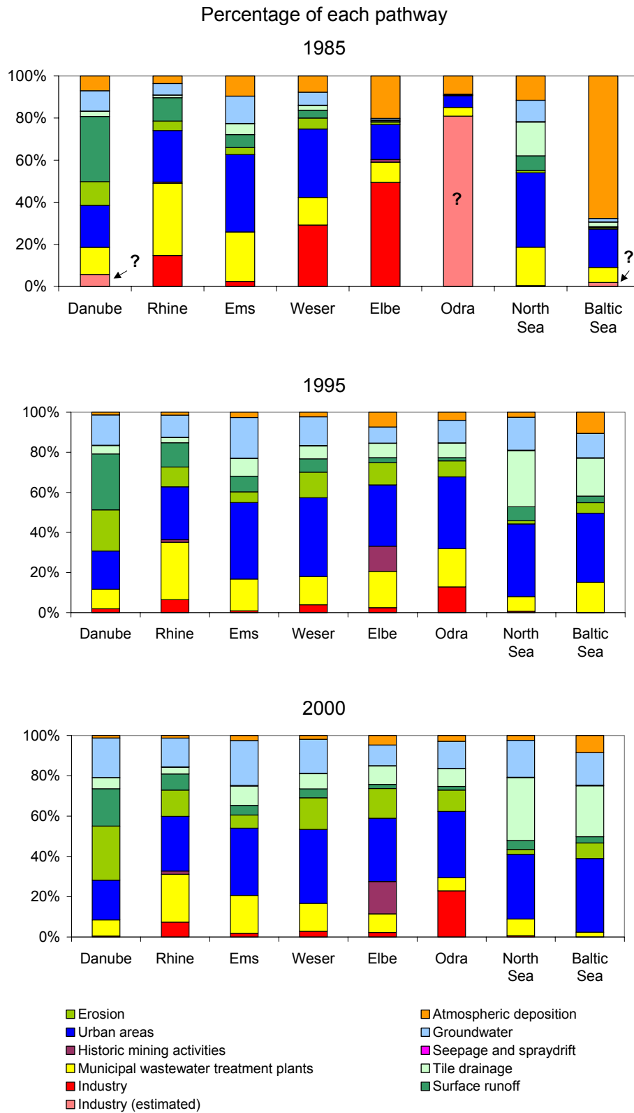
Figure 6-1 Cadmium emissions into German river basins.
