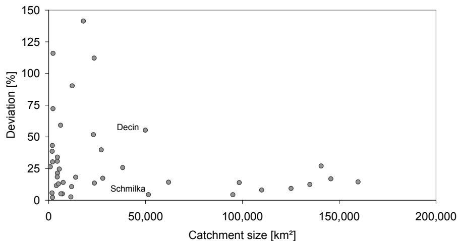
Figure 6-18 Deviation of calculated loads and loads measured monitoring stations versus catchment size on the example of Cu.
