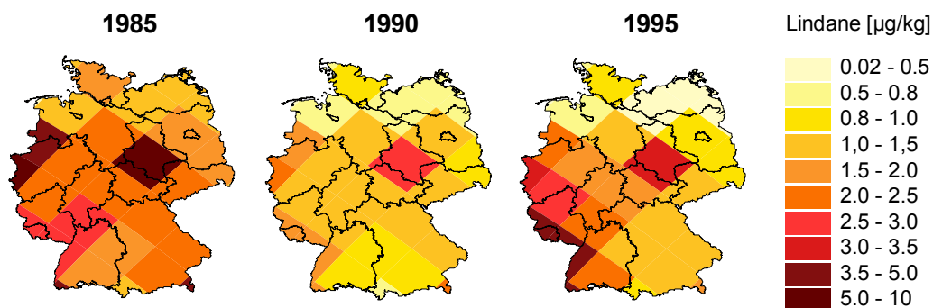
Figure 4-6 Lindane contents in the topsoil for 1985, 1990 and 1995 (MSC-East, 2001).
