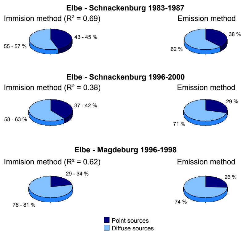
Figure 7-4 Comparison of the load shares from point and diffuse sources established following the immision and emission methods for the Elbe near Schnackenburg and Magdeburg.
