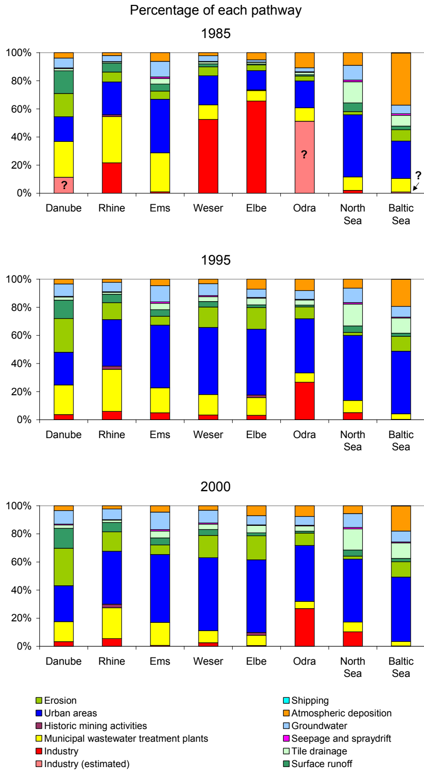
Figure 6-7 Zinc emissions into German river basins.
