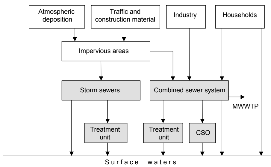
Figure 3-7 Sources and pathways of heavy metals from urban areas (changed according to Stotz/Knoche, 1999a).
