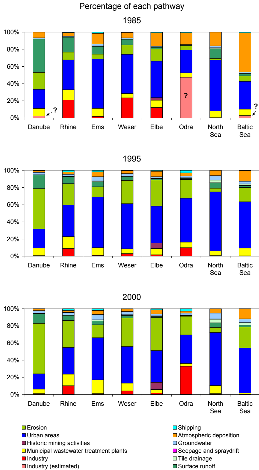
Figure 6-6 Lead emissions into German river basins.
