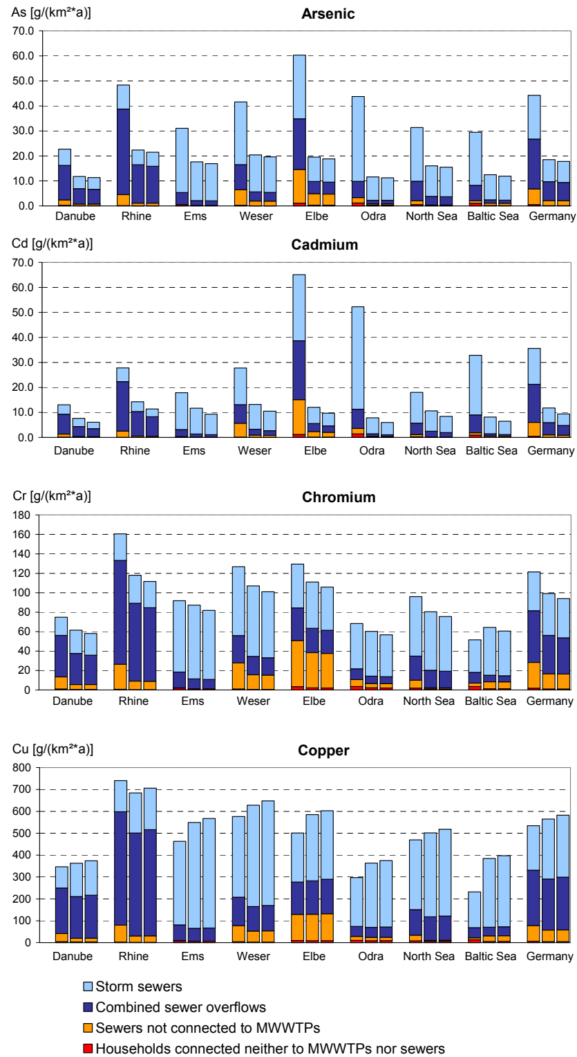
Figure 6-16a-d Specific emissions from urban areas in g/(km 2 catchment area · a).
