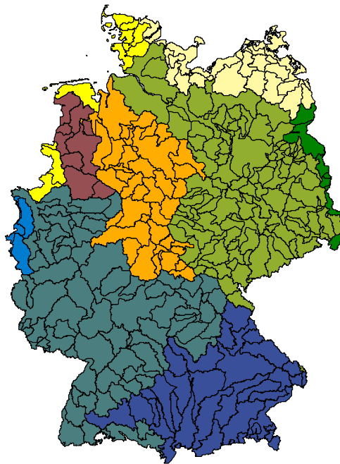
Figure 2-2 River systems in the MONERIS model (Behrendt et al., 1999).
