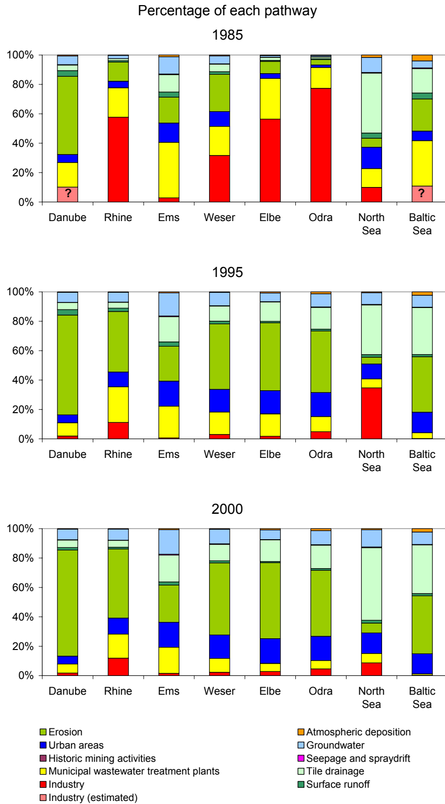
Figure 6-2 Chromium emissions into German river basins.
