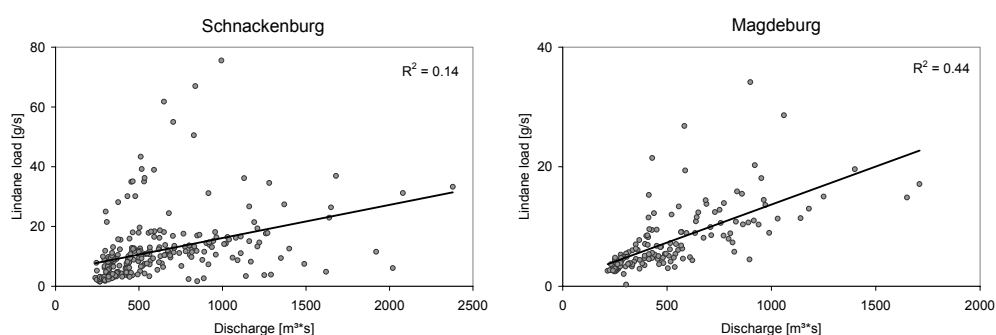
Figure 7-5 Relation between lindane load and discharge for Schnackenburg (1996-2000) and Magdeburg (1996-1998).
