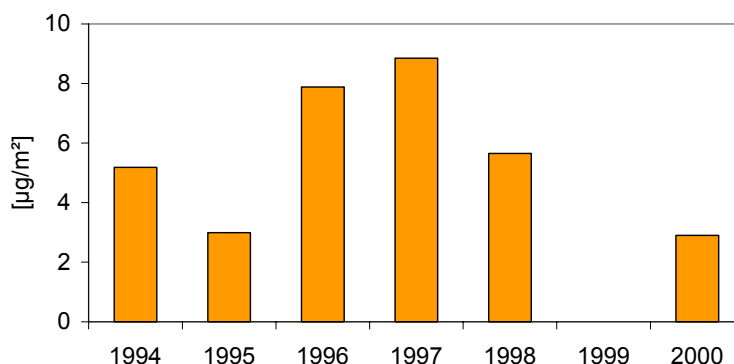
Figure 4-5 Lindane deposition at the surveying spot Zingst (wet-only) (UBA, 2000, 2001).
