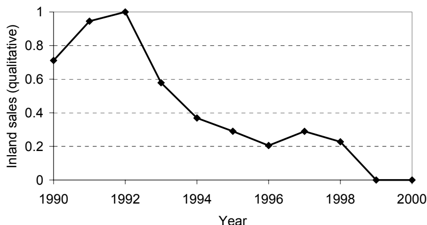
Figure 4-2 Development of German lindane inland sales (standardised) from 1990-2000 (according to BBA information, 2001, unpublished).
