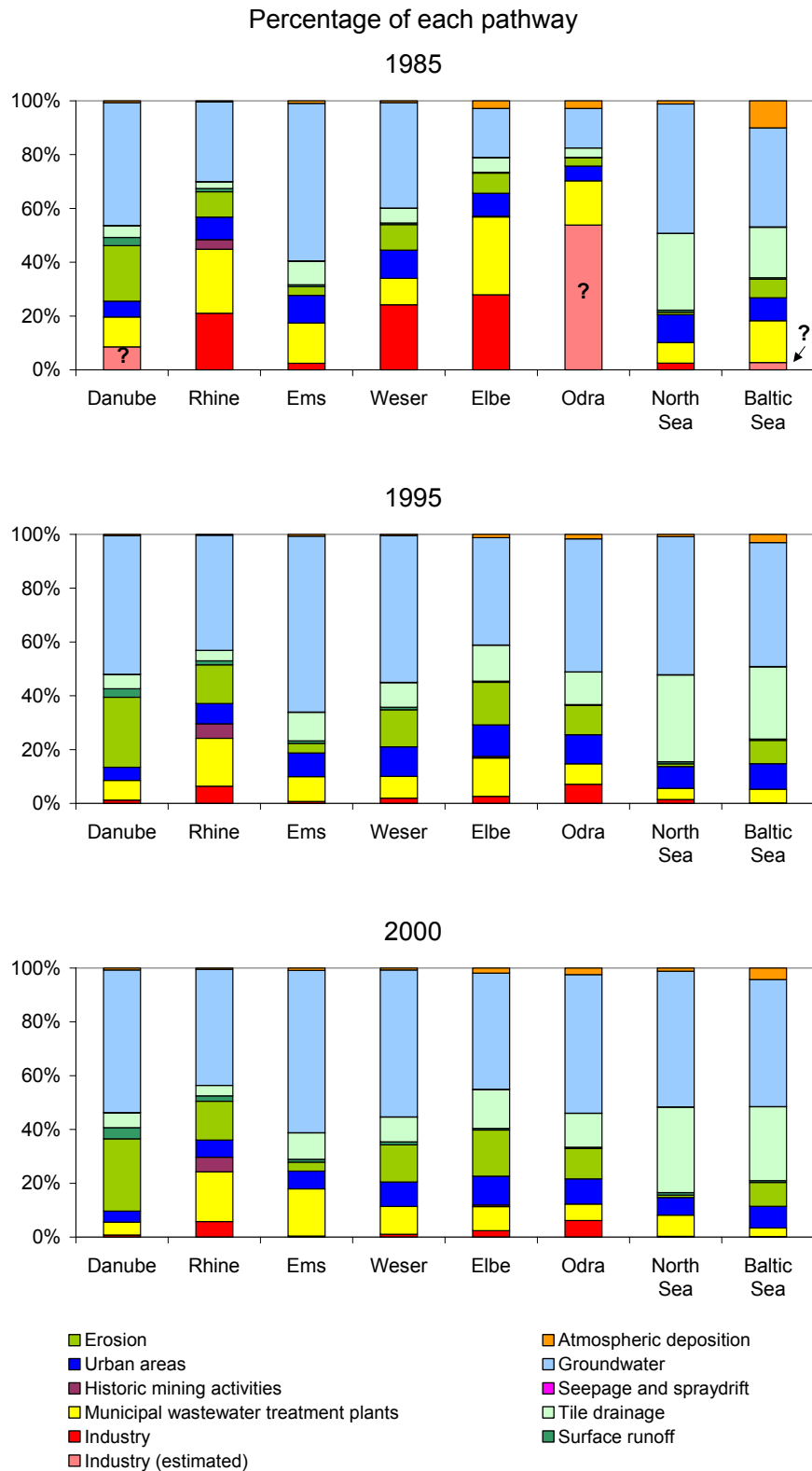
Figure 6-5 Nickel emissions into German river basins.
