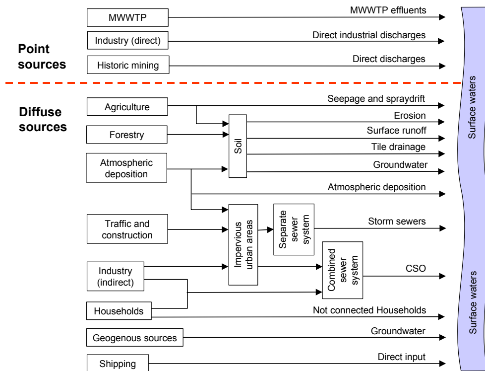
Figure 2-1 Sources and pathways of substances in river basins.
