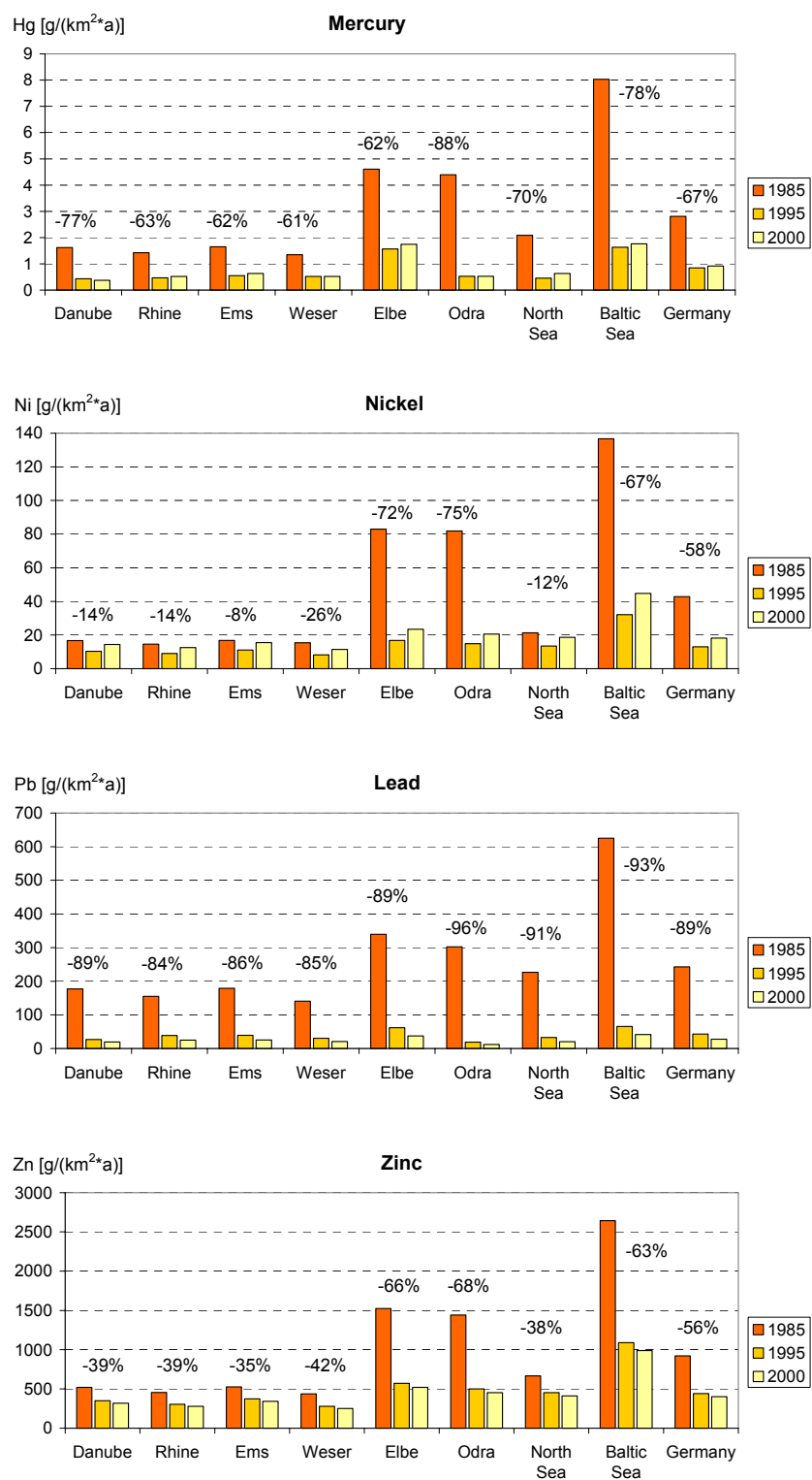
Figure 6-14e-h Surface specific heavy metal emissions from direct atmospheric deposition on the water surface in g/(km 2 catchment area·a).
