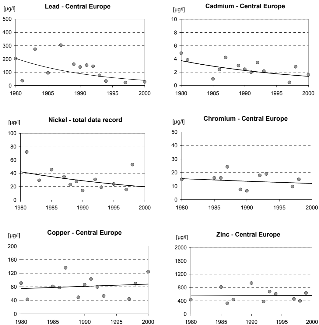
Figure 3-10 Concentrations in the runoff from paved areas for 1980-2000.
