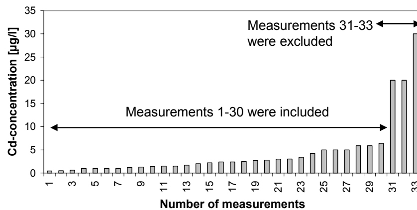
Figure 3-9 Ranking of Cd-concentrations in storm sewers.
