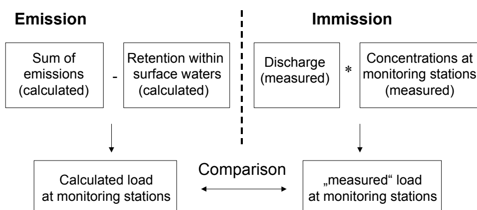
Figure 5-1 Relation between emission and immission.
