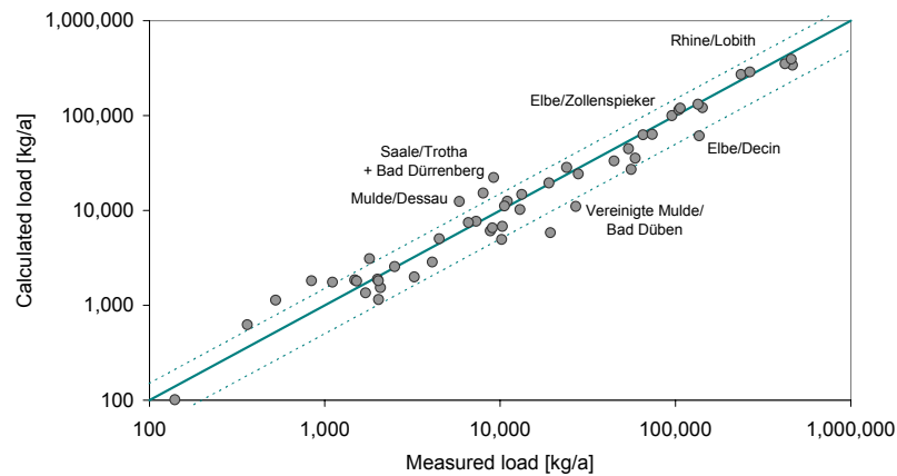
Figure 6-17a-c Comparison between calculated loads with loads measured at monitoring stations.
