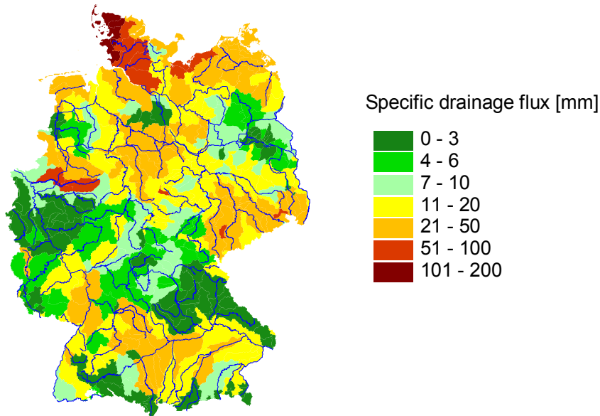
Figure 3-6 Specific drain rates for the German river basins from MONERIS (1995).
