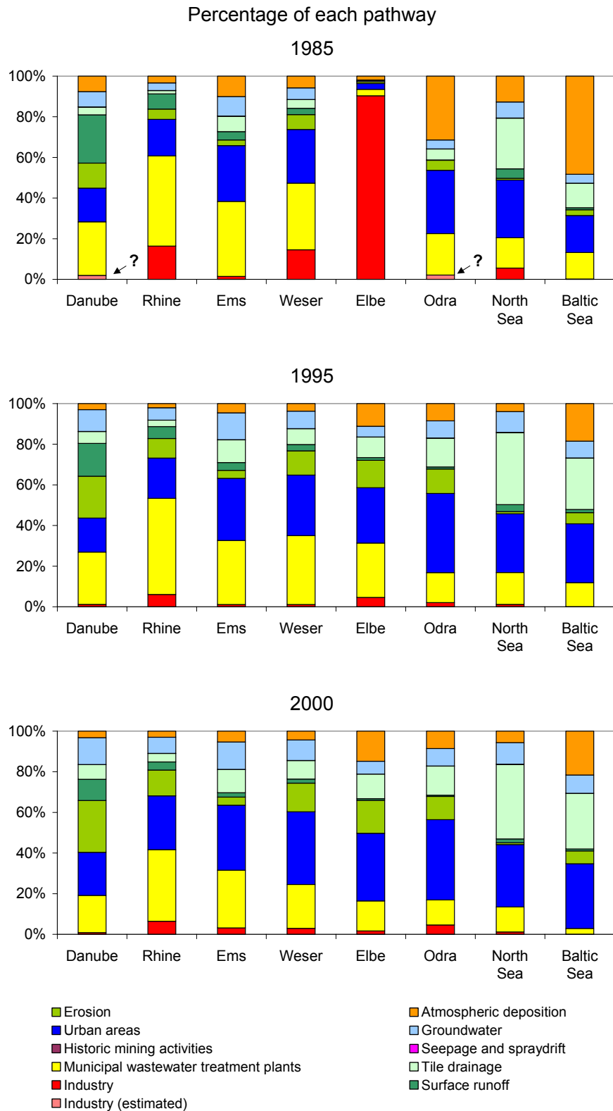
Figure 6-4 Mercury emissions into German river basins.
