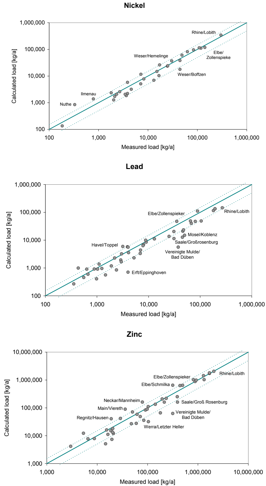
Figure 6-17d-f Comparison between calculated loads with loads measured at monitoring stations.
