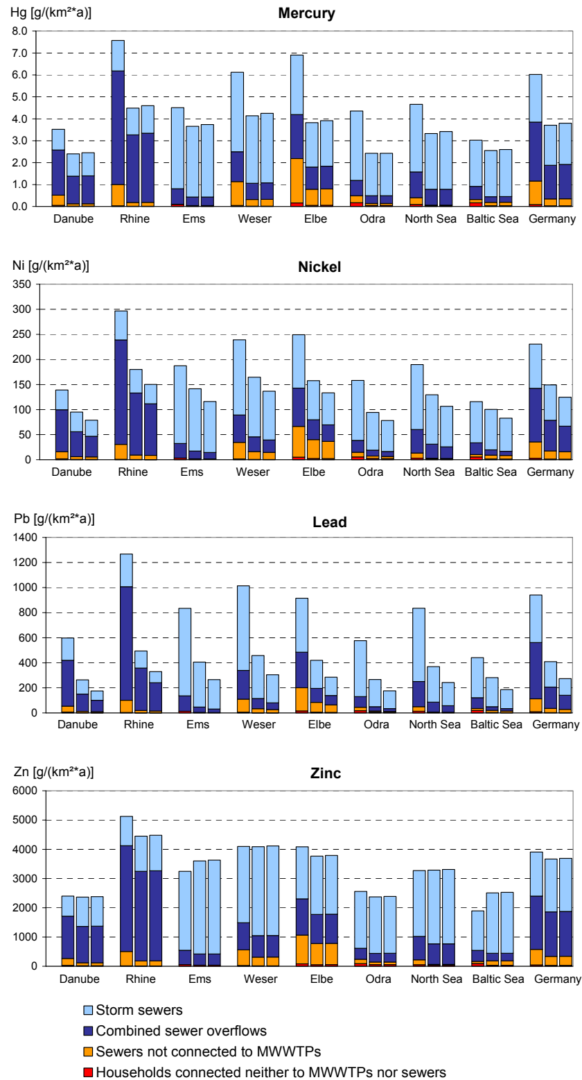
Figure 6-16e-h Specific emissions from urban areas in g/(km 2 catchment area · a).
