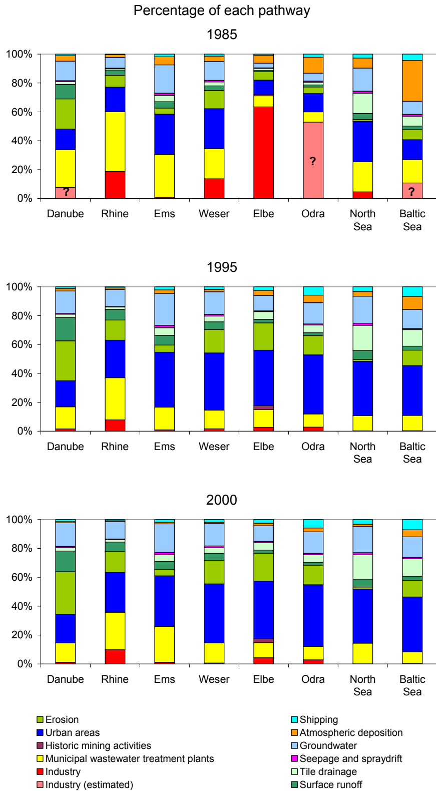
Figure 6-3 Copper emissions into German river basins.
