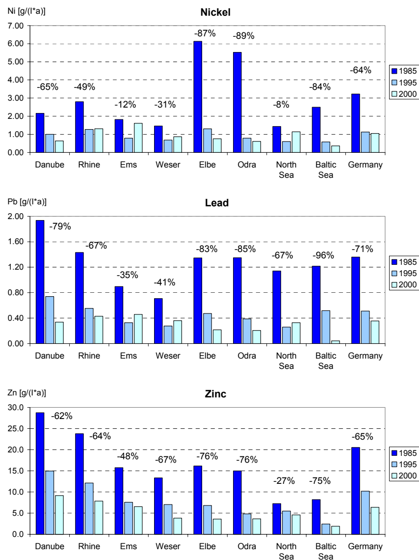
Figure 6-9e-g Specific heavy metal emissions per connected inhabitant via municipal wastewater treatment plant in g/(I·a).
