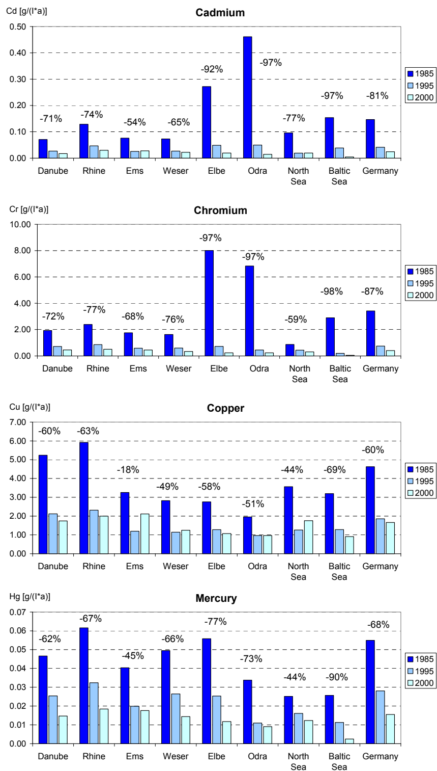
Figure 6-9a-d Specific heavy metal input per connected inhabitant via municipal wastewater treatment plants in g/(l*a).
