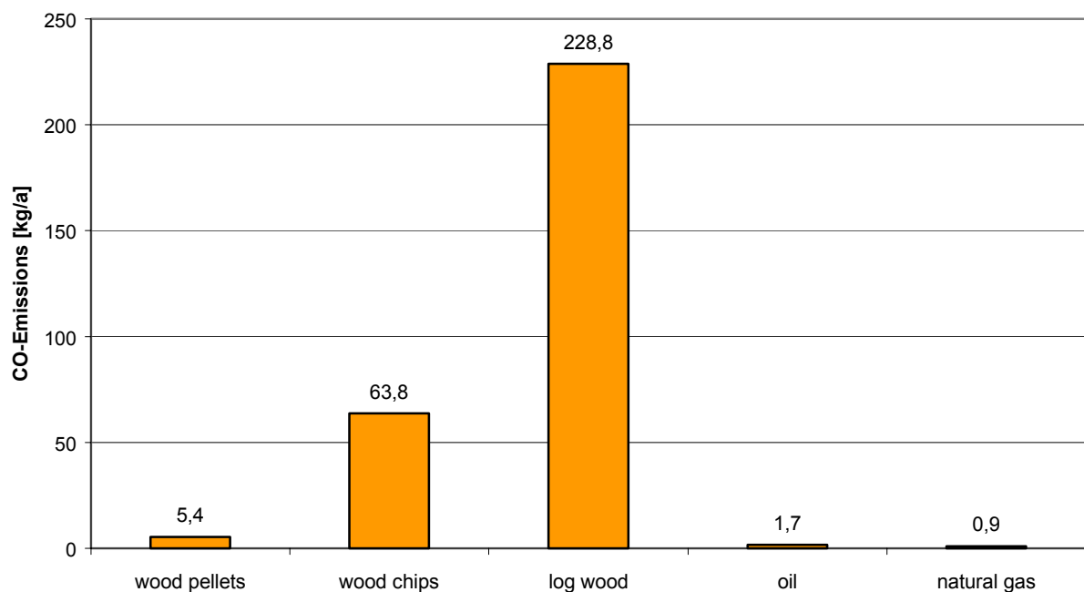
Figure 24: Carbon monoxide emissions
