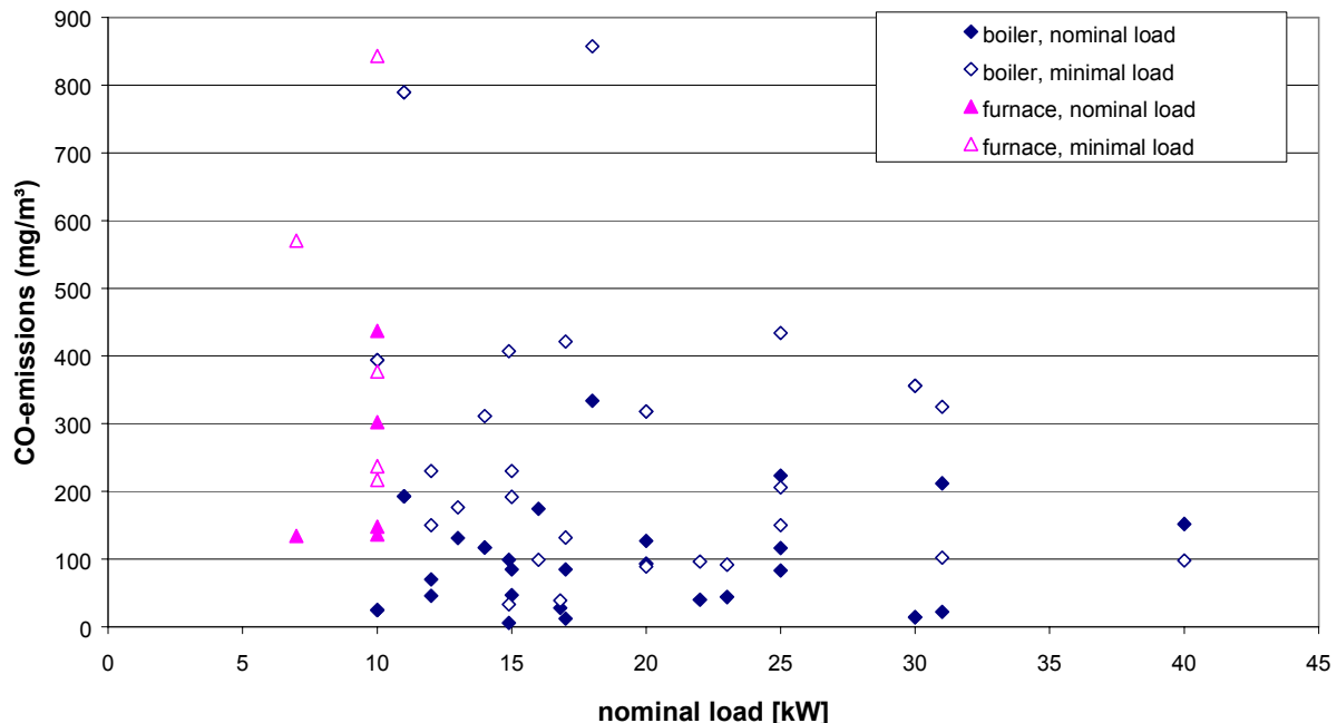
Figure 15: Carbon Monoxide Emissions of the Tested Pellet Firings (BLT since 1999)
