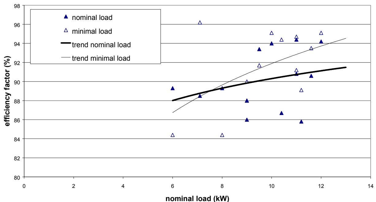
Figure 11: Firing Efficiencies of the Examined Pellet Furnaces
