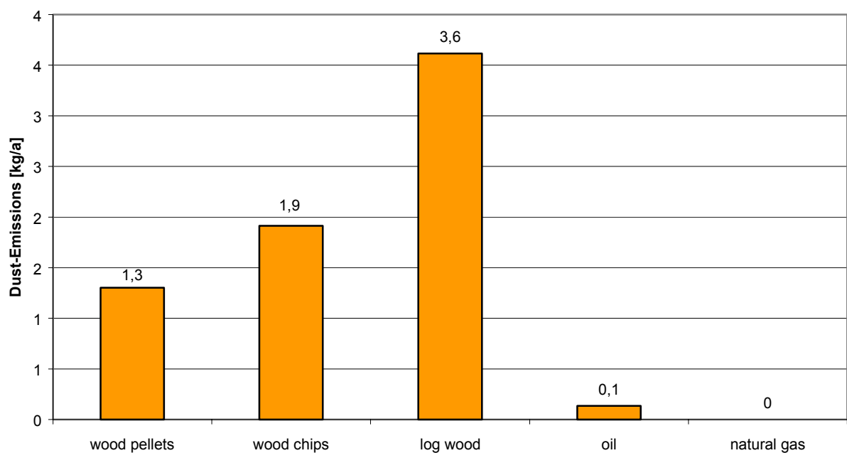
Figure 27: Dust Emissions
