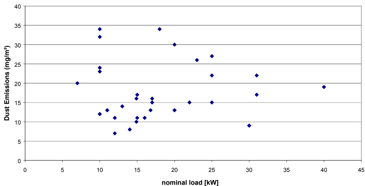
Figure 21: Dust Emissions of the Tested Pellet Firings (BLT since 1999)
