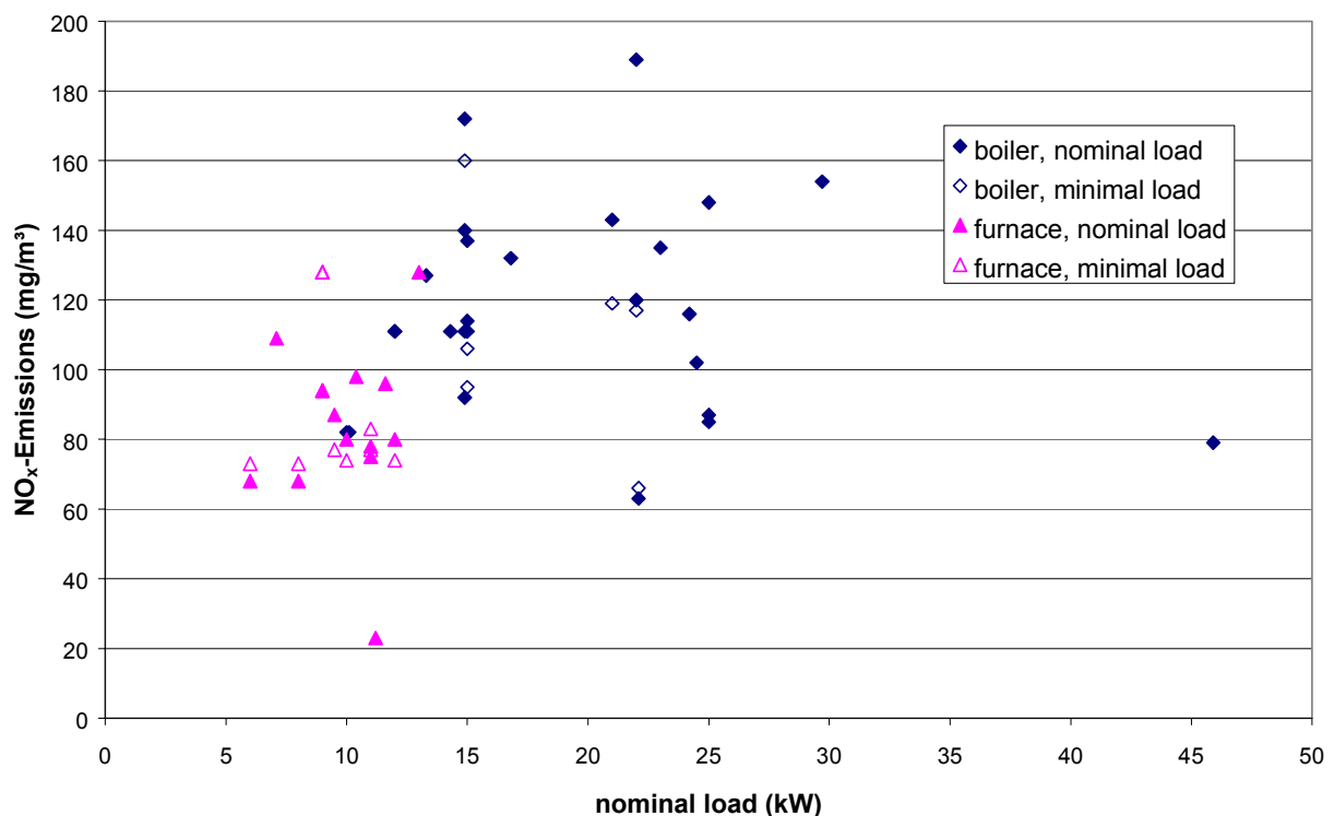
Figure 18: NO x Emissions of the Examined Pellet Firings
