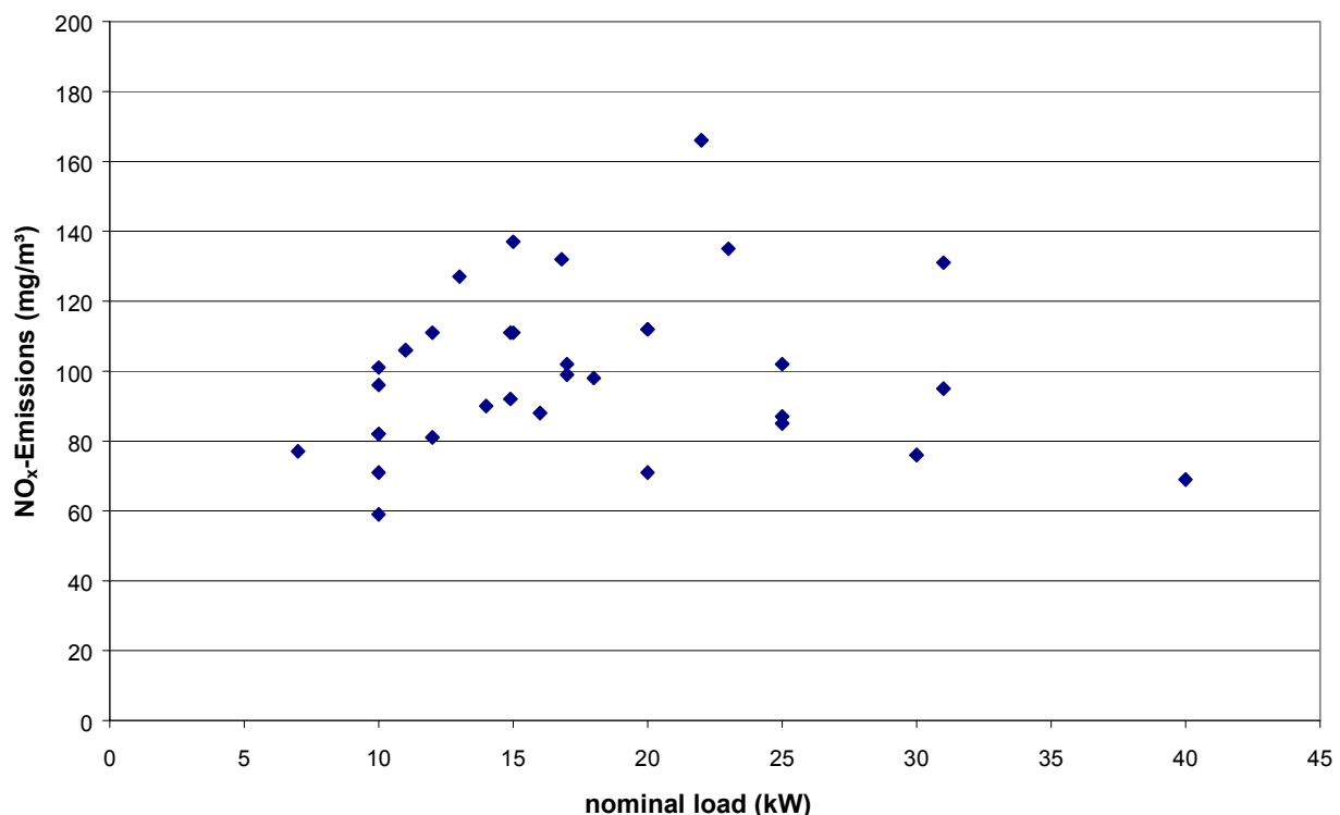
Figure 19: Nitrogen Oxide Emissions of the Tested Pellet Firings (BLT since 1999)
