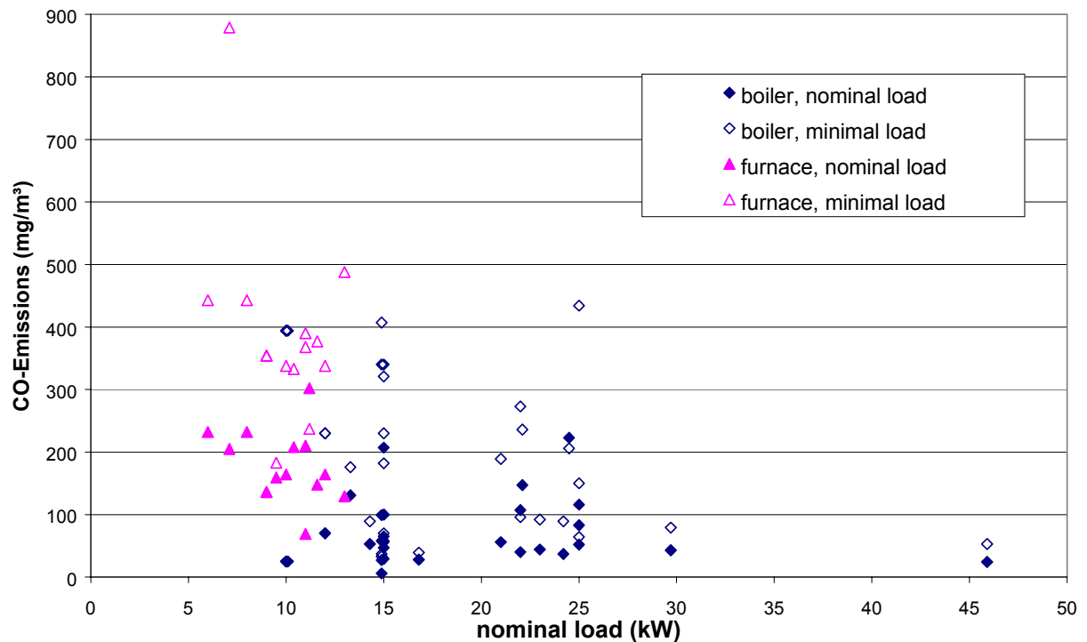
Figure 14: Carbon Monoxide Emissions of the Examined Pellet Firings
