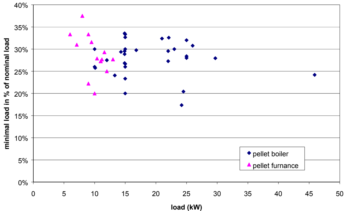
Figure 8: Minimal Load of the Examined Pellet Firings in Relation to Nominal Load
