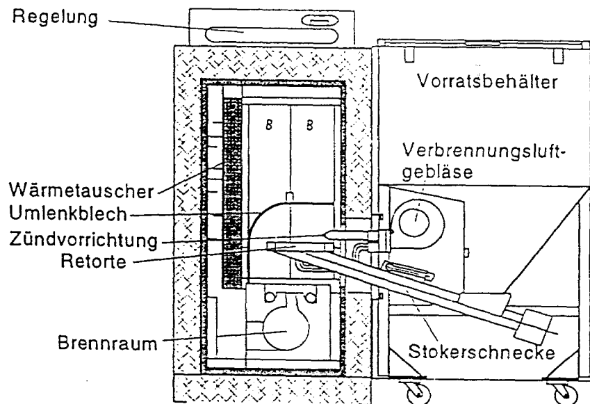
Figure 3: Pellet Boiler with Storage Vessel
