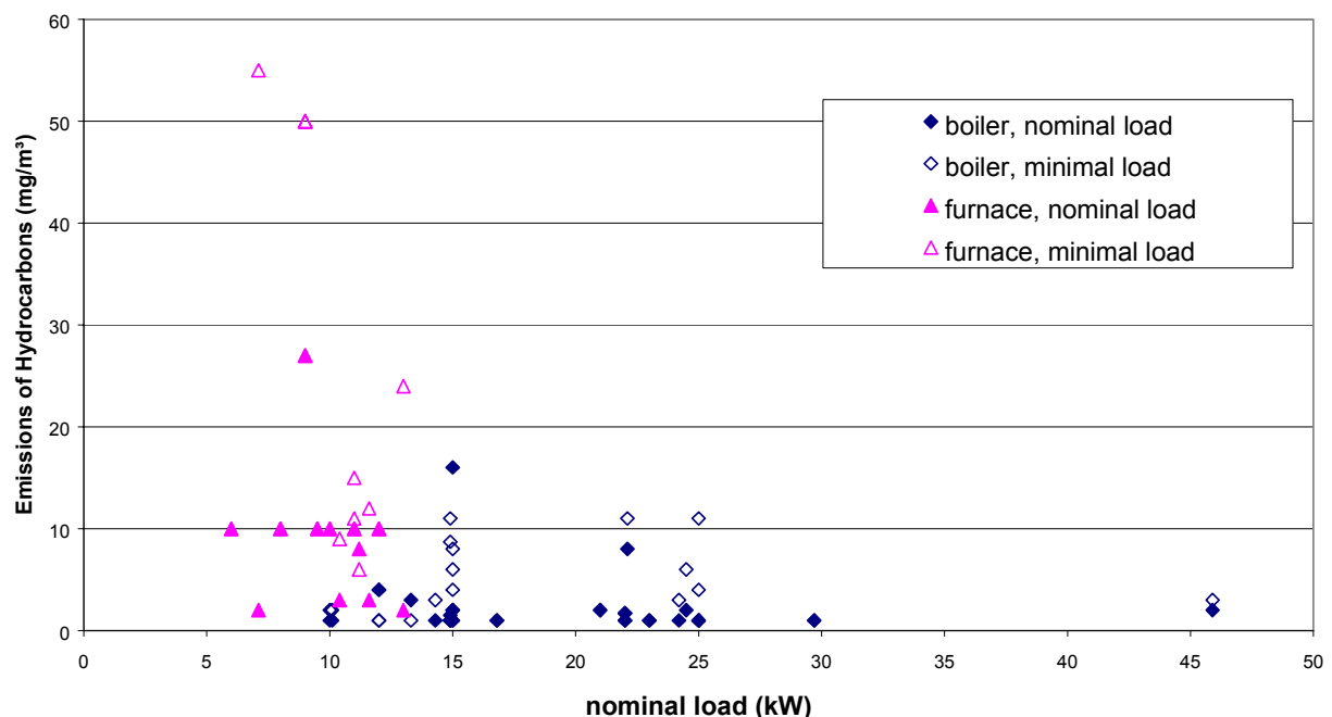
Figure 16: Emissions of Hydrocarbons ( C_{total} )
