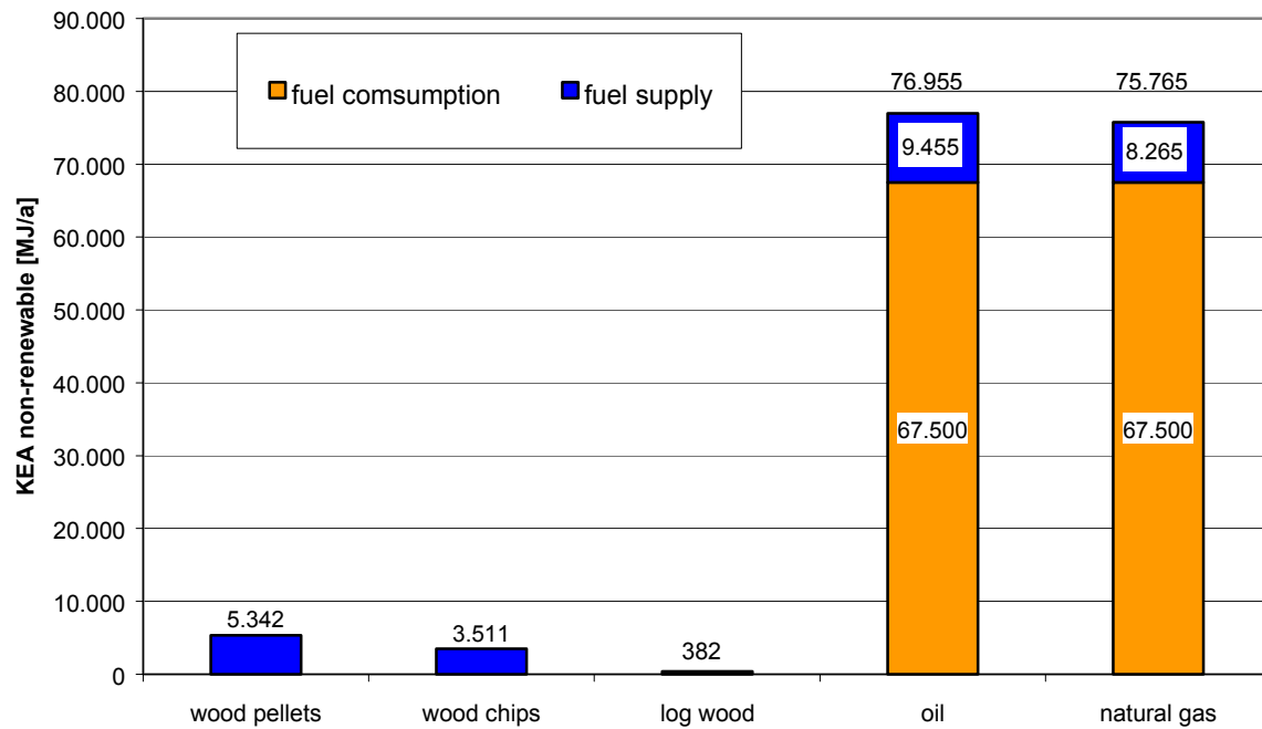
Figure 22: Cumulated Use of Non-Renewable Primary Energy
