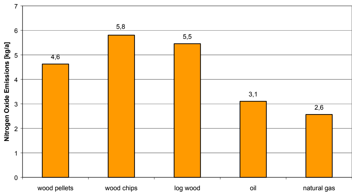
Figure 26: Nitrogen Oxide Emissions
