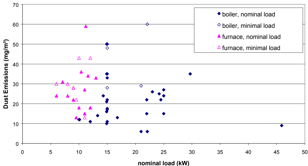
Figure 20: Dust Emissions of the Examined Pellet Firings
