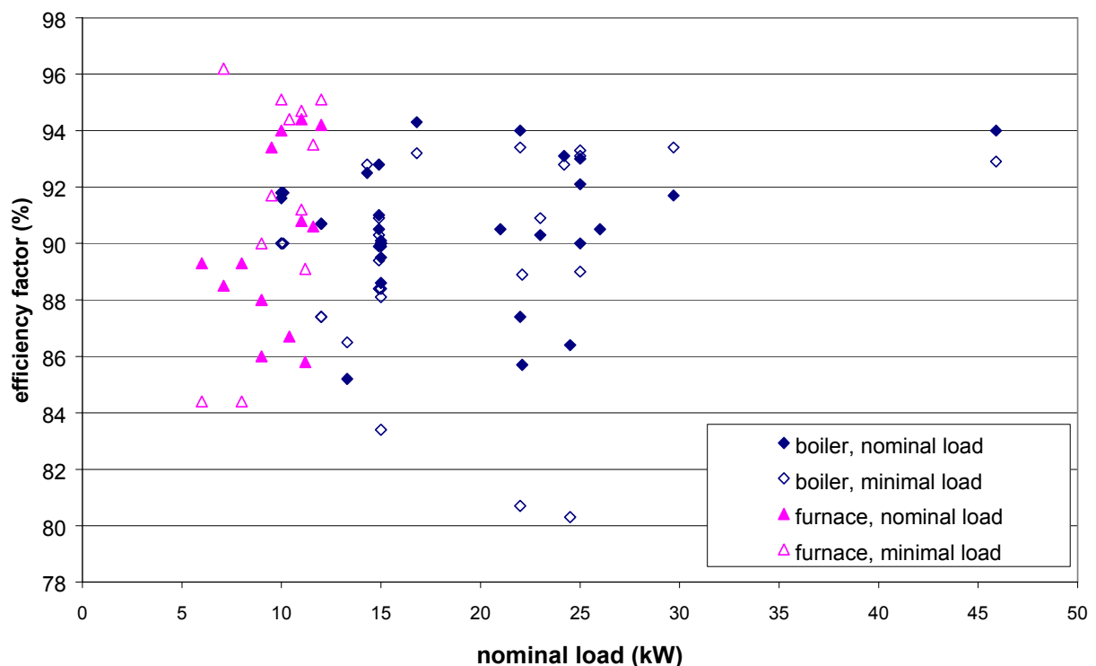
Figure 9: Efficiencies of the Examined Pellet Firings (Pellet Boilers: Boiler Efficiency, Pellet Furnaces: Firing Efficiency)
