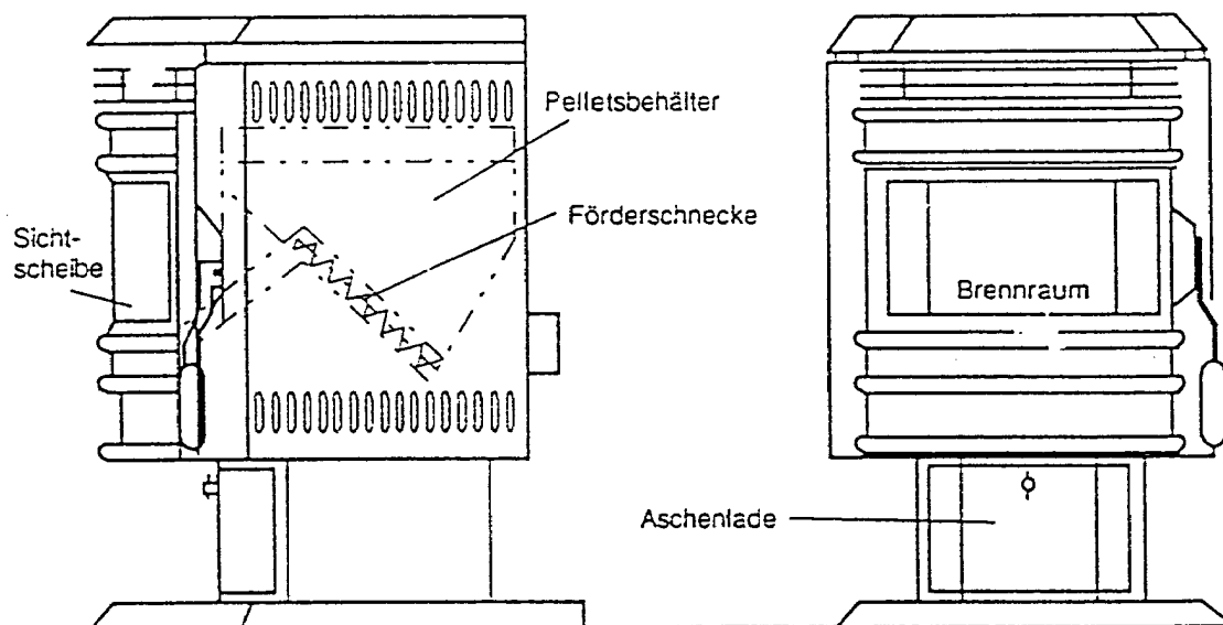
Figure 2: Pellet Furnace
