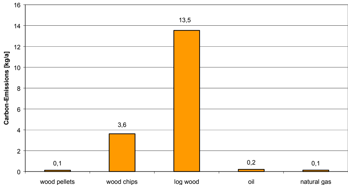
Figure 25: Emissions of Hydrocarbons
