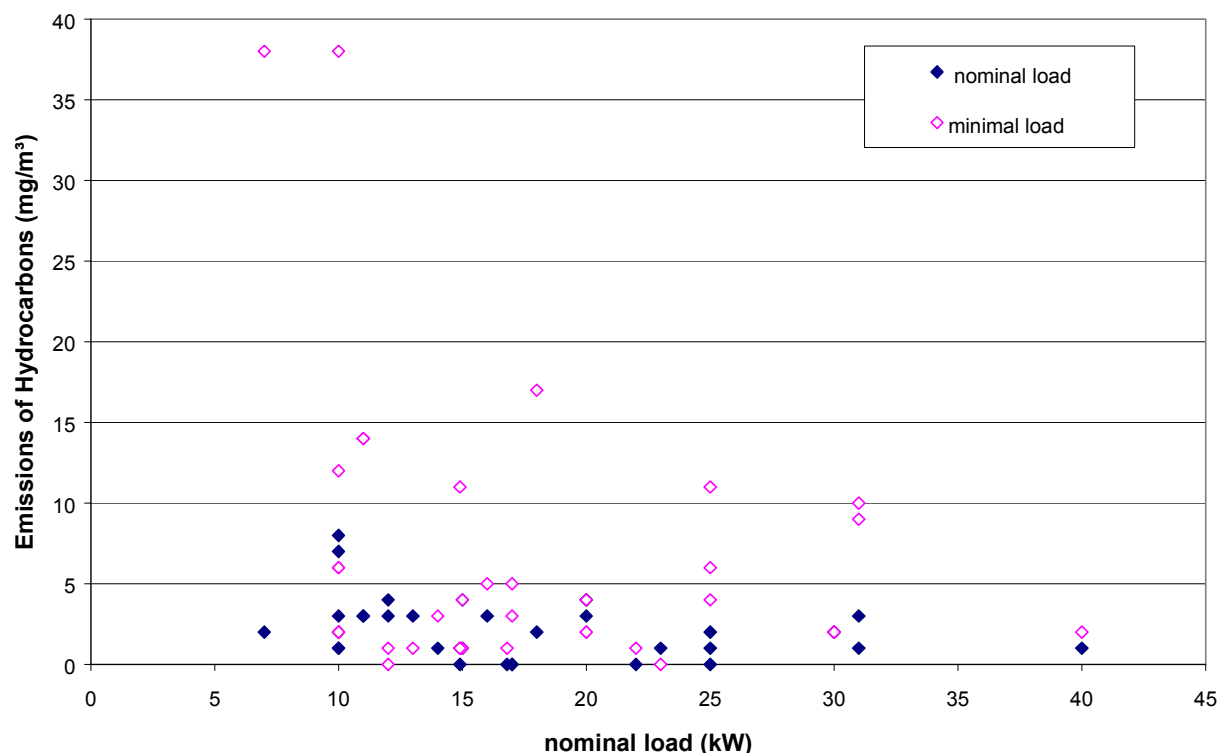
Figure 17: Emission of Hydrocarbons of the Tested Pellet Firings (BLT since 1999)
