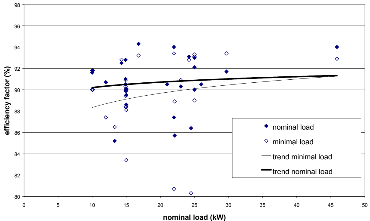
Figure 10: Boiler Efficiencies of the Examined Pellet Boilers
