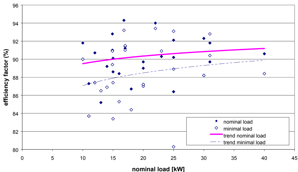
Figure 12: Boiler Efficiencies of Tested Pellet Boilers (BLT Wieselburg, since 1999)
