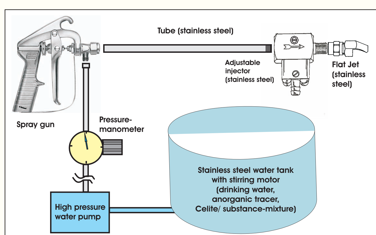
Fig. 3: Application: Liquid dosing of solved Metilox® (above), dosing of suspended Metilox® (below)
