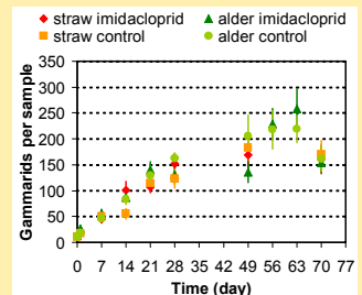
Fig. 6: Mean number of gammarids per sample (n=4)
