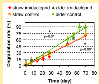
Fig. 7: Mean degradation rate of leaf fraction > 2000µm (n=4)
