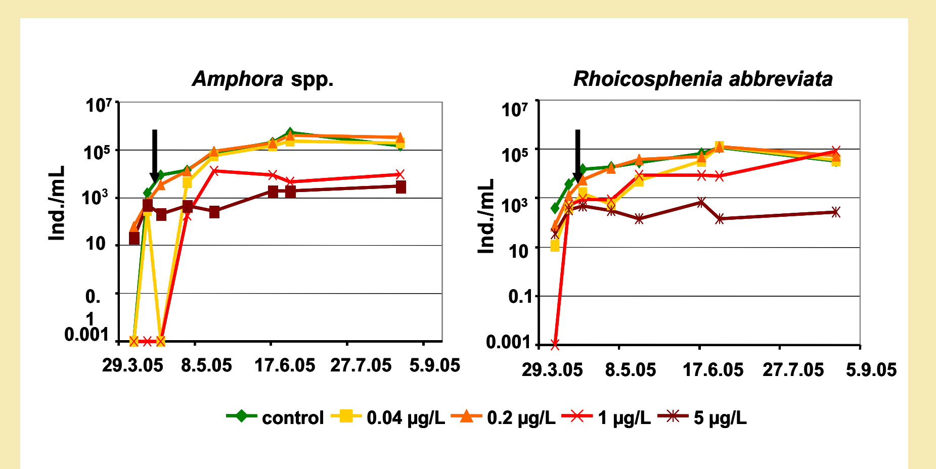
Fig. 8: Dynamics of two periphyton species in the pond mesocosms. Arrow: day of application
