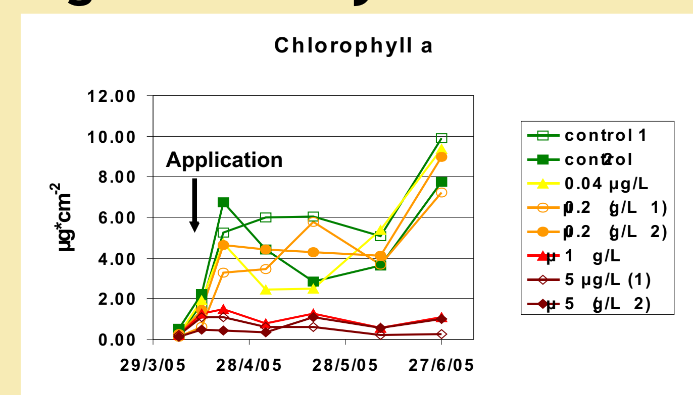
Fig. 5: Dynamics of chlorophyll-a on the substrates at the different Irgarol concentrations.
