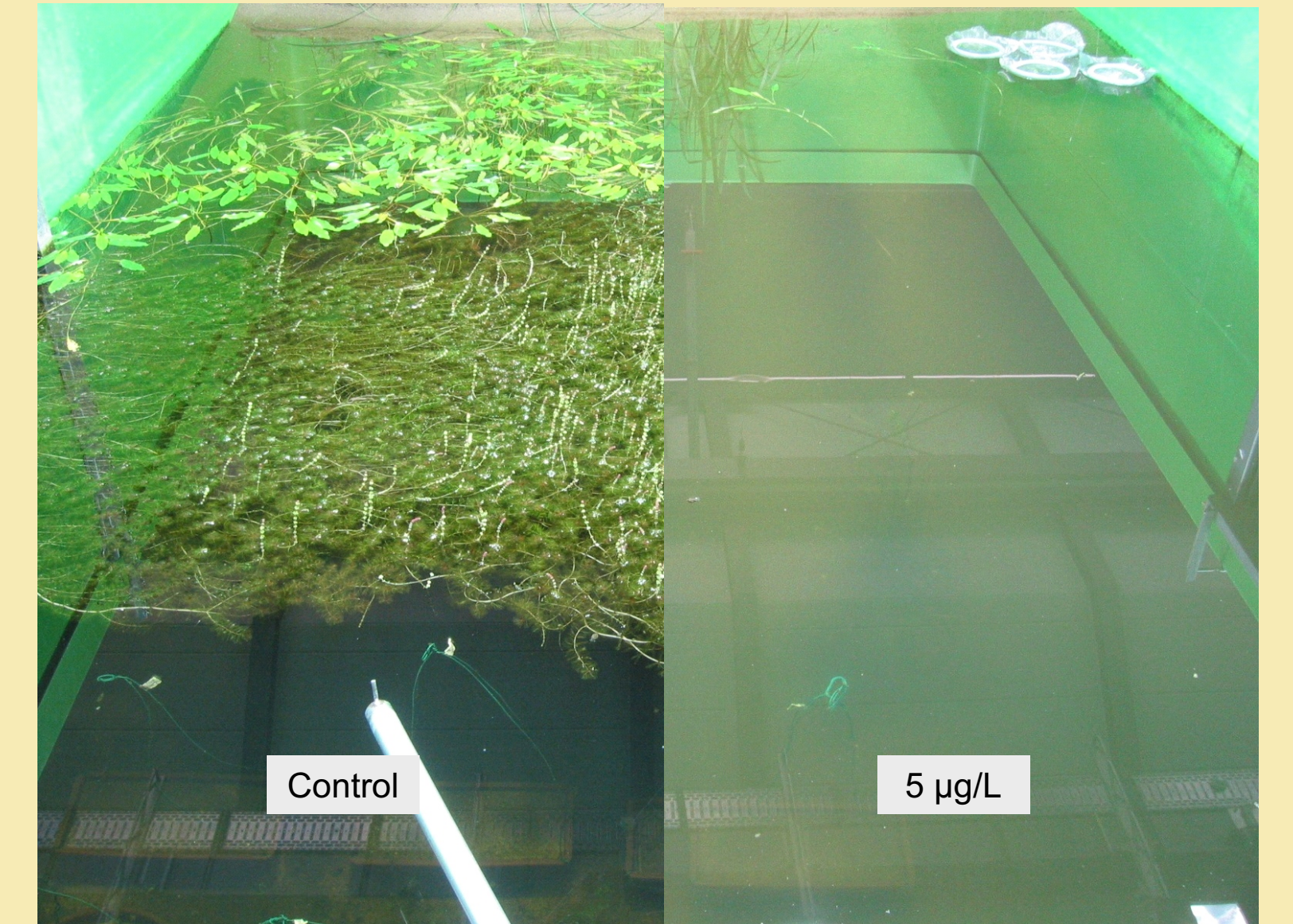
Fig. 2: Control pond and pond contaminated with 5 \mu\text{g/L} Irgarol (14.06.05)
