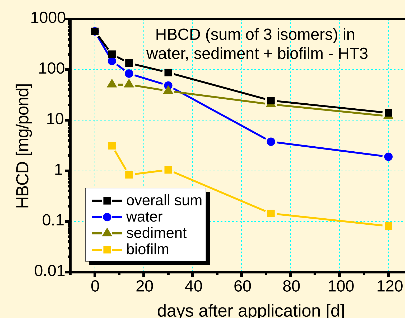
Fig. 6: HBCD (sum of isomers) - pond budget (HT3) for a 120-d-period incl. water, sediment and biofilm
