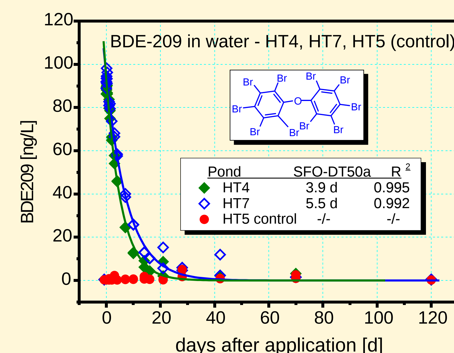
Fig. 3: BDE-209 - water concentration and DT50 in the spiked ponds (HT4, HT7) and in the control pond (HT5)
