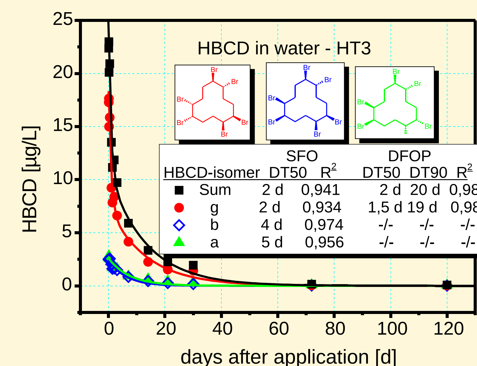
Fig. 5: HBCD (isomers + sum) - water concentration and DT50 in the spiked pond (HT3)
