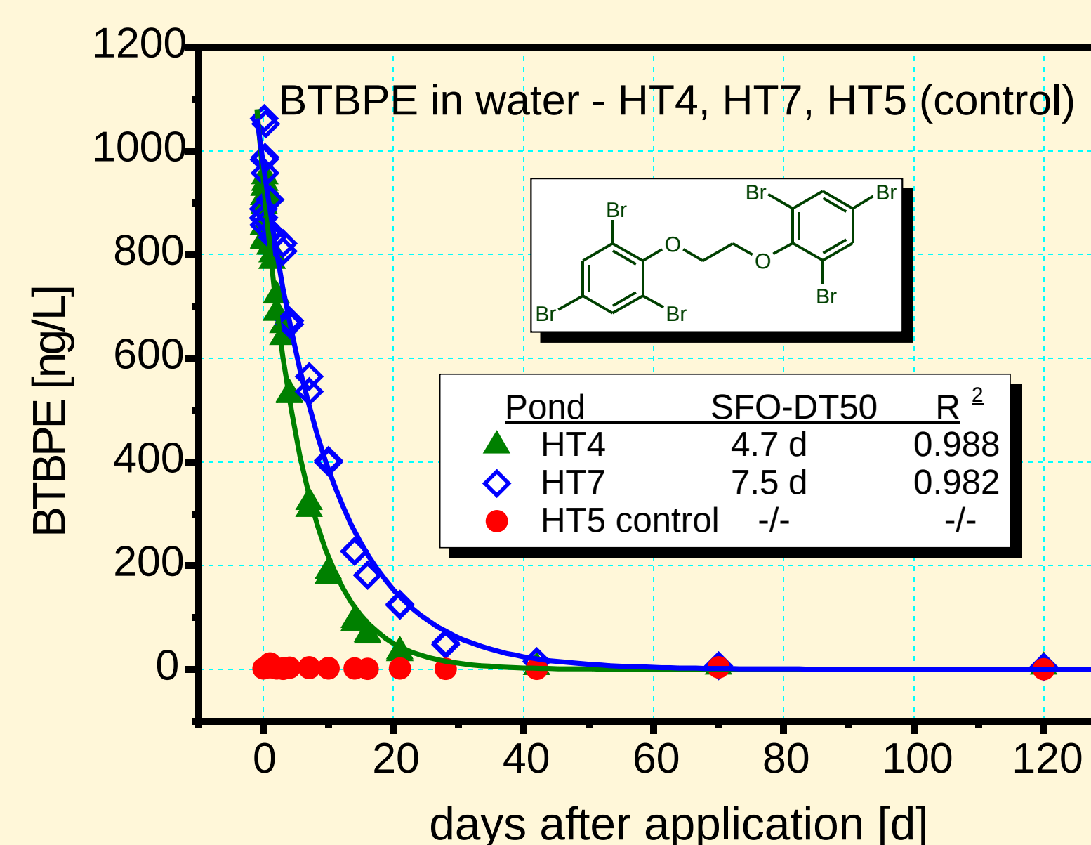
Fig. 2: BTBPE - water concentration and DT50 in the spiked ponds (HT4, HT7) and in the control pond (HT5)
