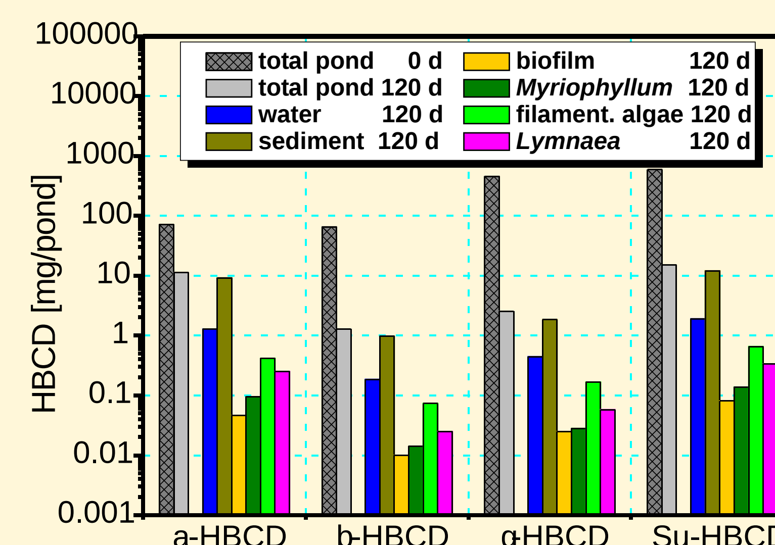
Fig. 7: HBCD (sum + isomers) - pond budget of HT3 at day 0 and day 120 incl. water, sediment, biofilm, macrophytes ( Myriophyllum spicatum , filamentous algae) and snails ( Lymnaea stagnalis ) at day 120
