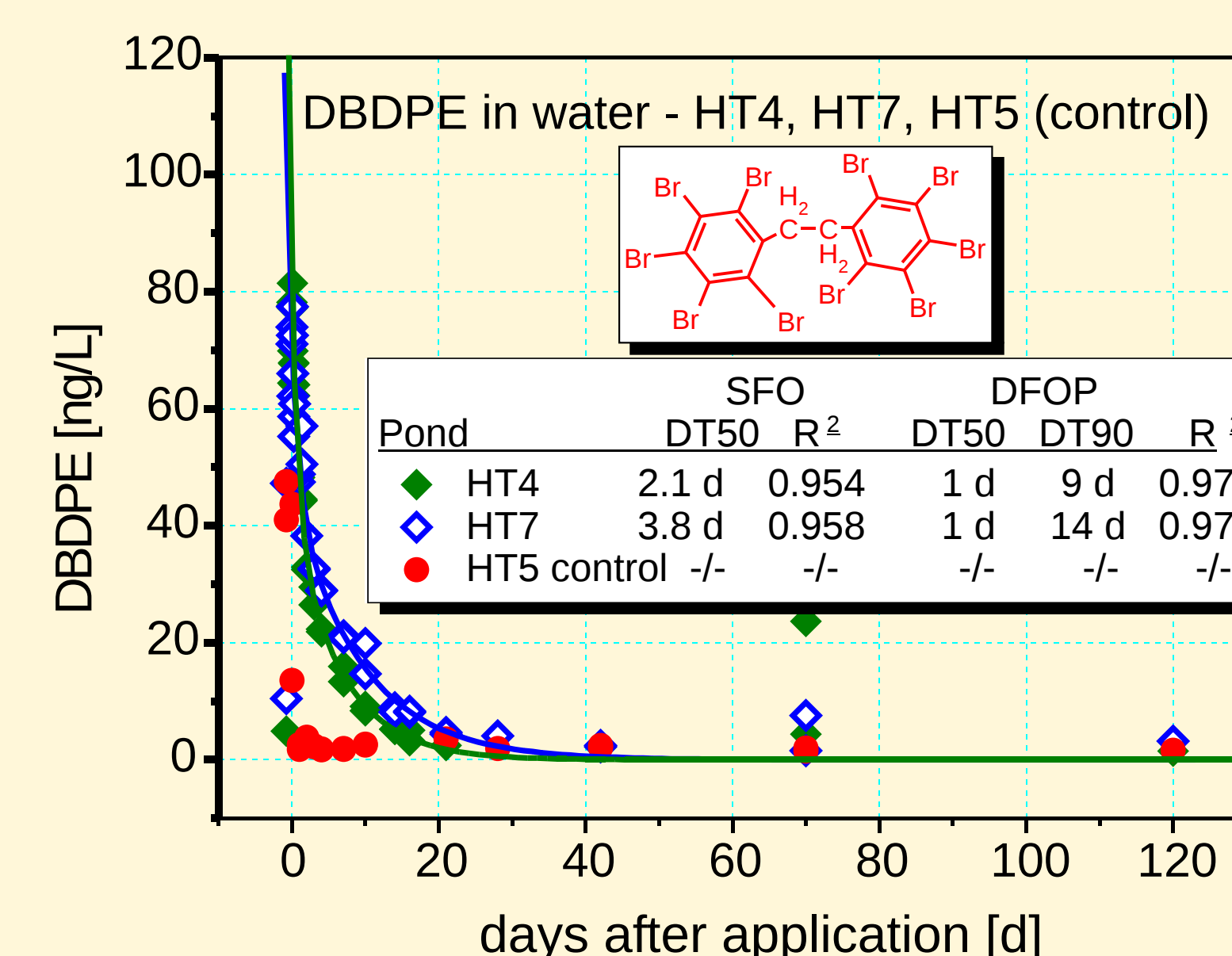
Fig. 4: DBDPE - water concentration and DT50 in the spiked ponds (HT4, HT7) and in the control pond (HT5)
