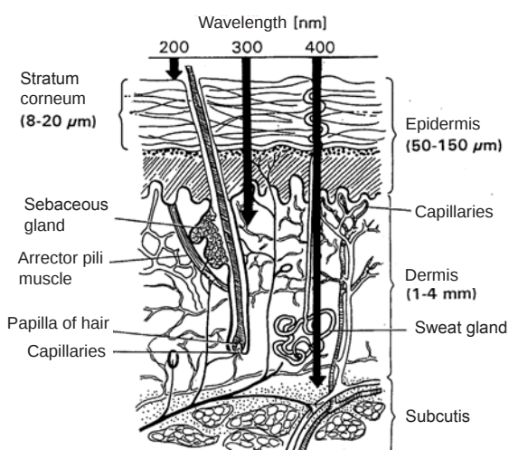
Figure 2: Spectral UV penetration of the skin surface. Reproduced from: Bundesgesundheitsblatt, Sonderheft "UV-Strahlung und Gesundheit", vol. 27 (1994).
