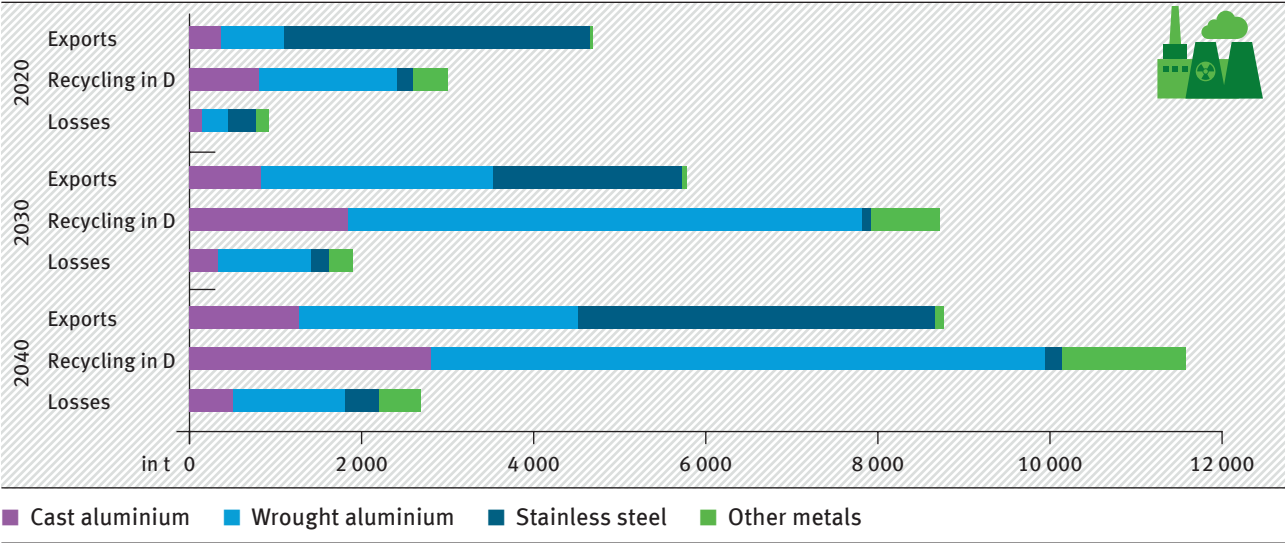
Material fate sector 4 power generation plants: conventional and renewable energy plants in tonnes per year
