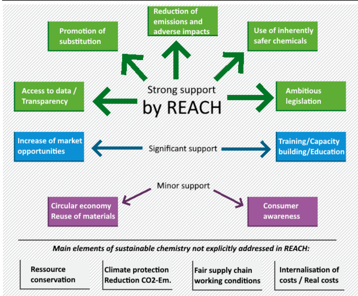
Figure 1: Main elements of sustainable chemistry (green boxes) explicitly addressed in REACH and main elements not explicitly addressed (white boxes).
