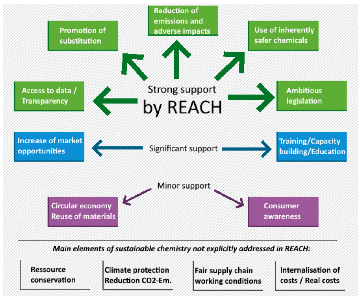
Figure 1: Main elements of sustainable chemistry (green boxes) explicitly addressed in REACH and main elements not explicitly addressed (grey boxes).
