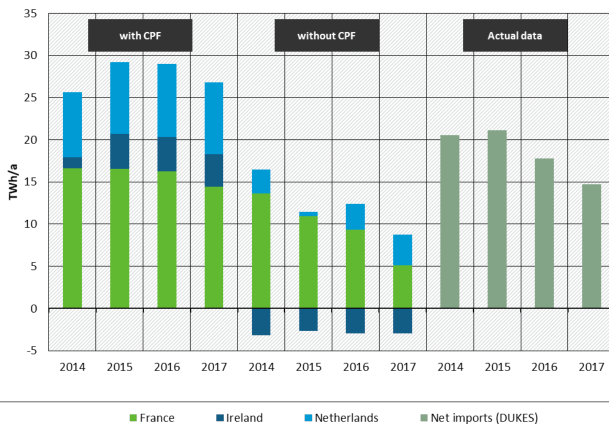
Figure 5: Net imports of UK (Tier 2 model results and actual data). >0: import; <0: export
