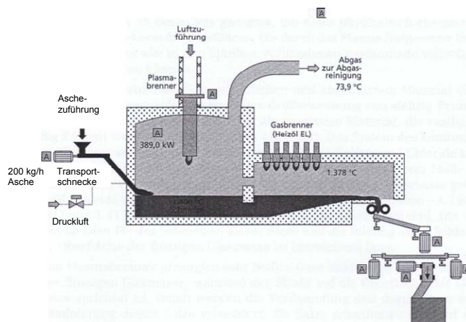
Figure Z.10: Simplified process scheme of the plasma melting furnace
