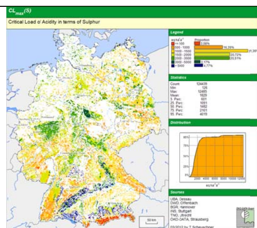
Figure DE-3: CL_{max}(S)
