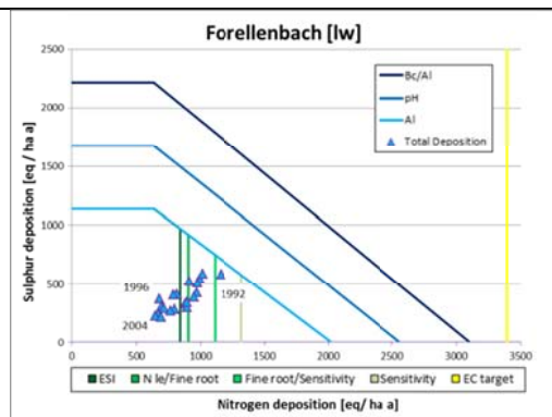
Figure DE-1: Example of Critical Load Function
