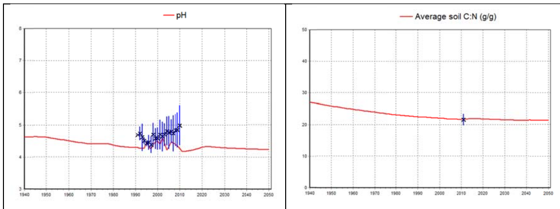
Figure DE-9: pH value (left) and C:N ratio (right) modelled with the VSD+ model on the ICP IM plot “Forellenbach”
