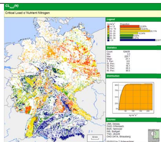
Figure DE-5: CL_{nut}(N)
