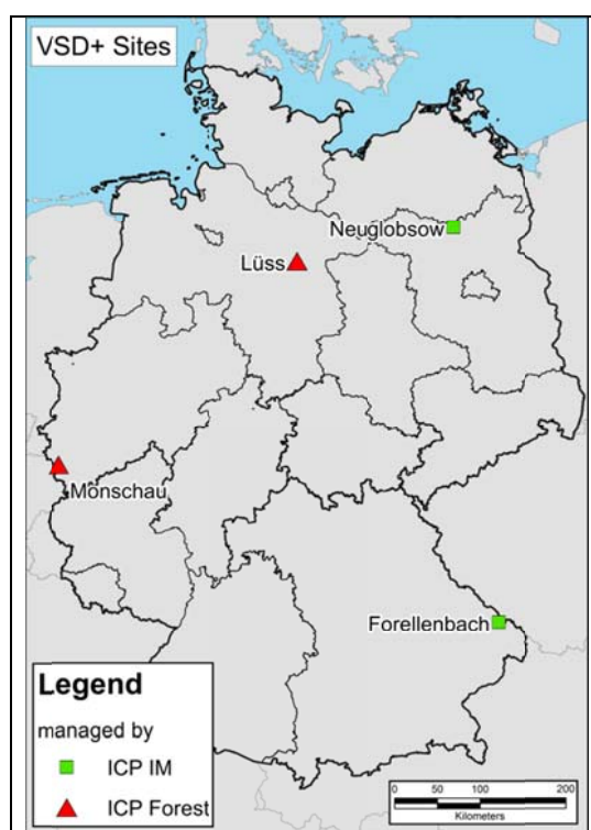
Figure DE-7: Selected sites for the VSD+ model in Germany
