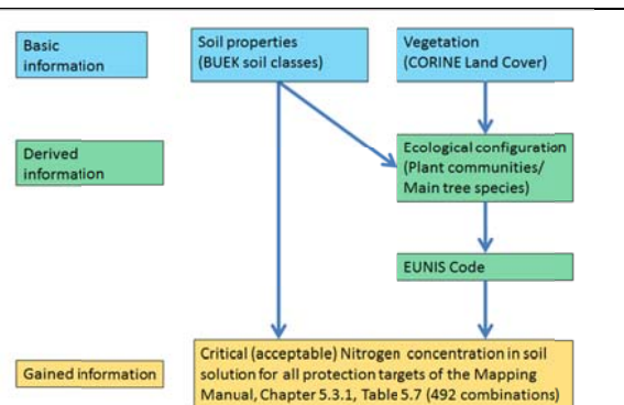
Figure DE-2: Deriving critical N concentrations
