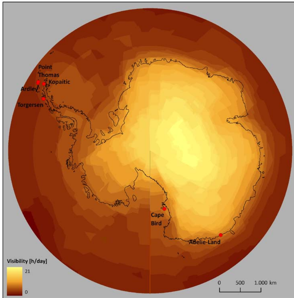
Figure 4: Visibility distribution of optical remote sensing systems, dependent on day length (Giesen 2006) and cloud cover (Jubier 2006) between 60 and 90° S and between November and February.
