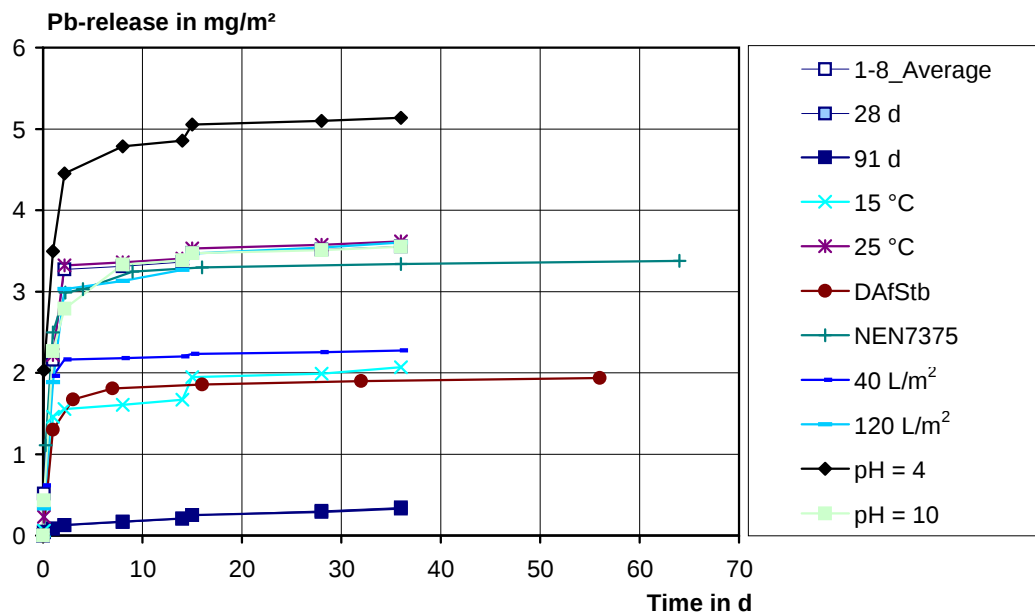
Figure 13: Release of lead for the variation of the test conditions according to Table 5 (first concreting)
