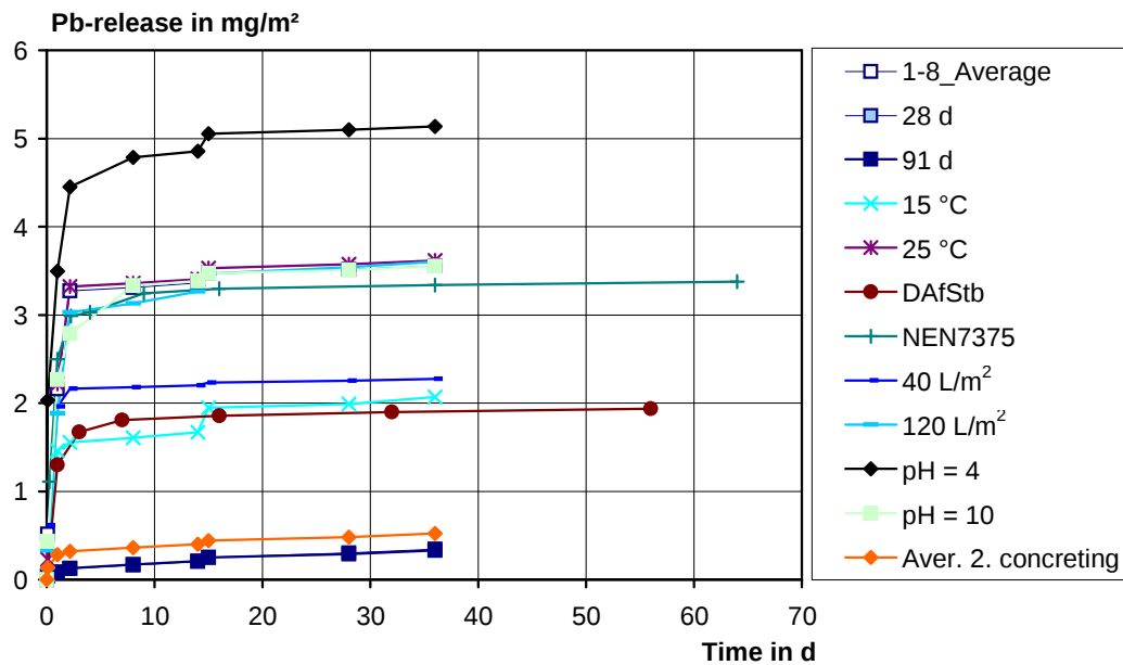
Figure 35: Release of lead for all concretes of the first and second concreting
