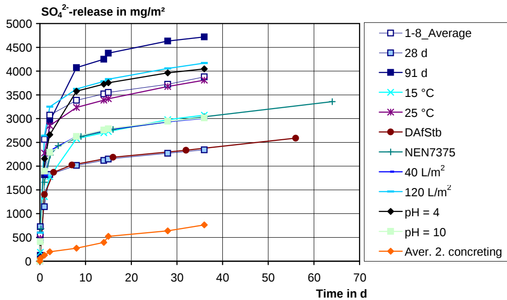
Figure 42: Release of sulphate for all concretes of the first and second concreting
