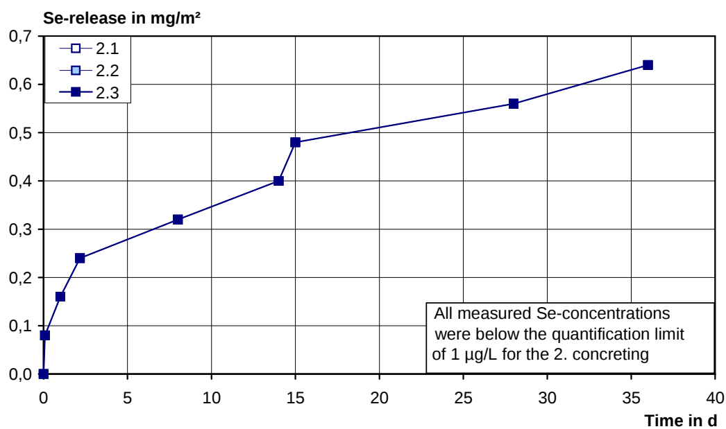
Figure 30: Release of selenium in the triplicate test (second concreting)
