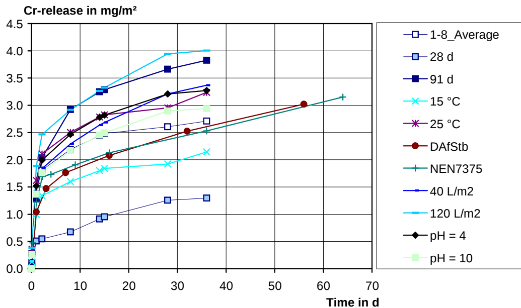
Figure 15: Release of chromium for the variation of the test conditions according to Table 5 (first concreting)
