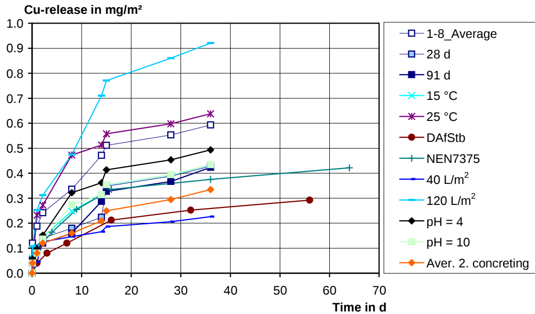
Figure 39: Release of copper for all concretes of the first and second concreting
