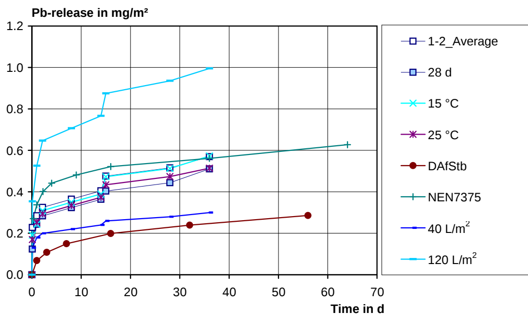
Figure 57: Release of lead for the variation of the test conditions according to Table 10
