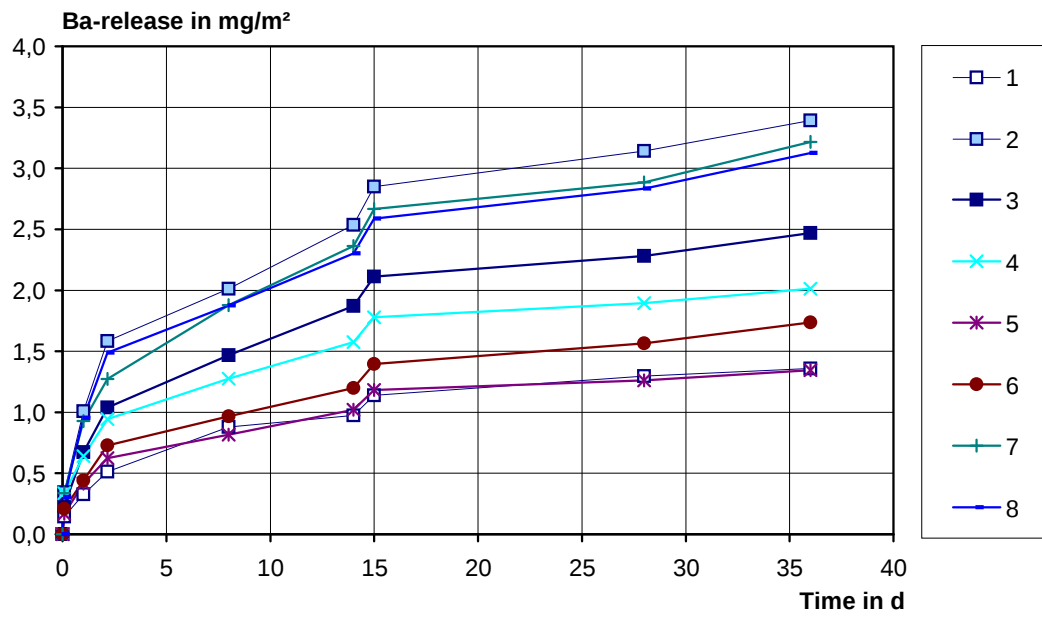
Figure 1: Release of barium in the eightfold test (first concreting)
