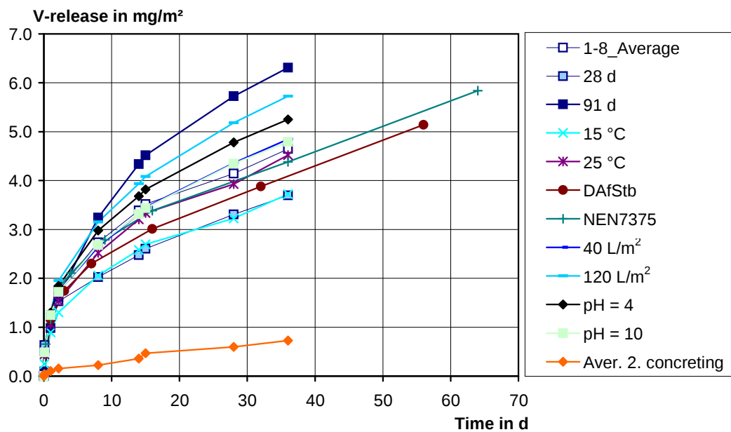
Figure 43: Release of vanadium for all concretes of the first and second concreting
