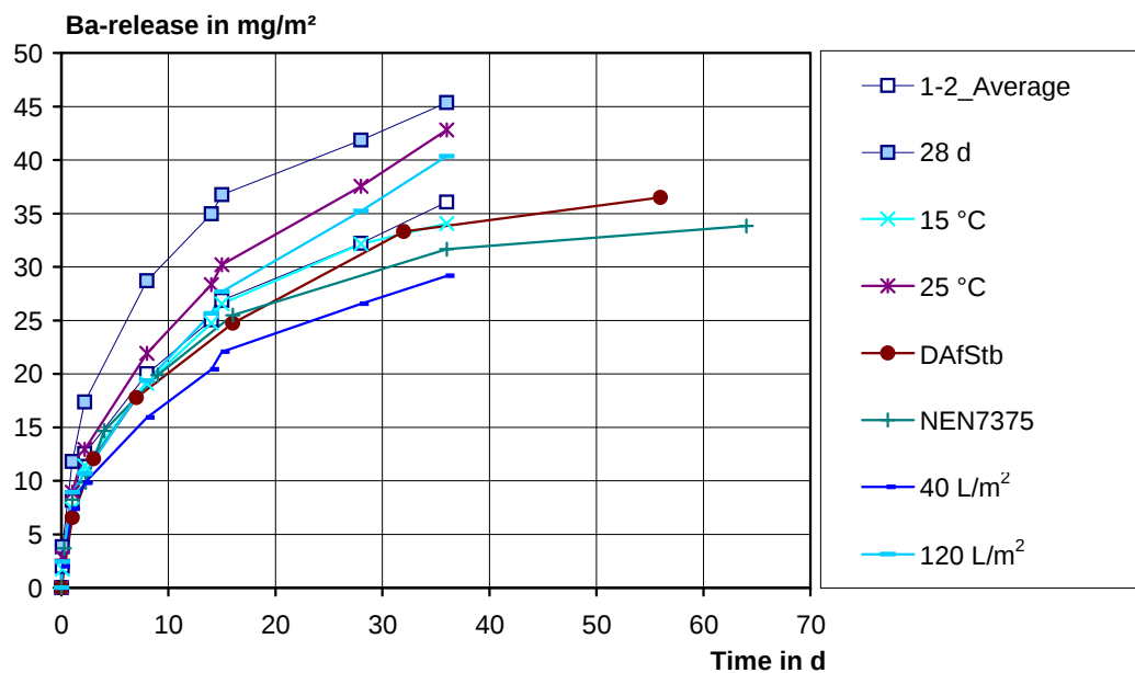
Figure 56: Release of barium for the variation of the test conditions according to Table 10
