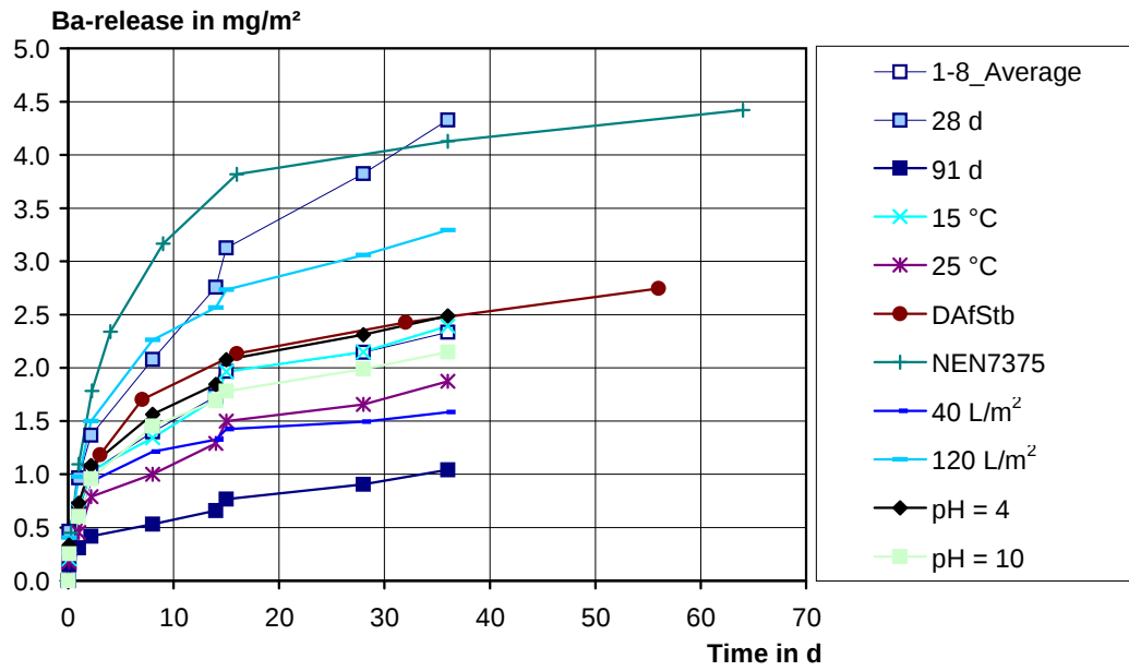
Figure 12: Release of barium for the variation of the test conditions according to Table 5 (first concreting)
