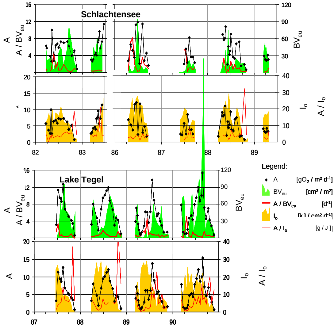
Figure 44. Integrals of gross primary production ( A ; black curves) in Schlachtensee and Lake Tegel in relation to
