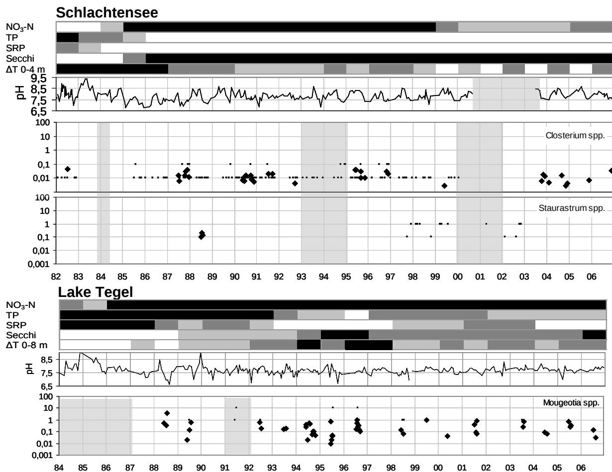
Fig. 39. Conjugatophyta pulations in Schlachtensee and in Lake Tegel in relation to abiotic conditions
