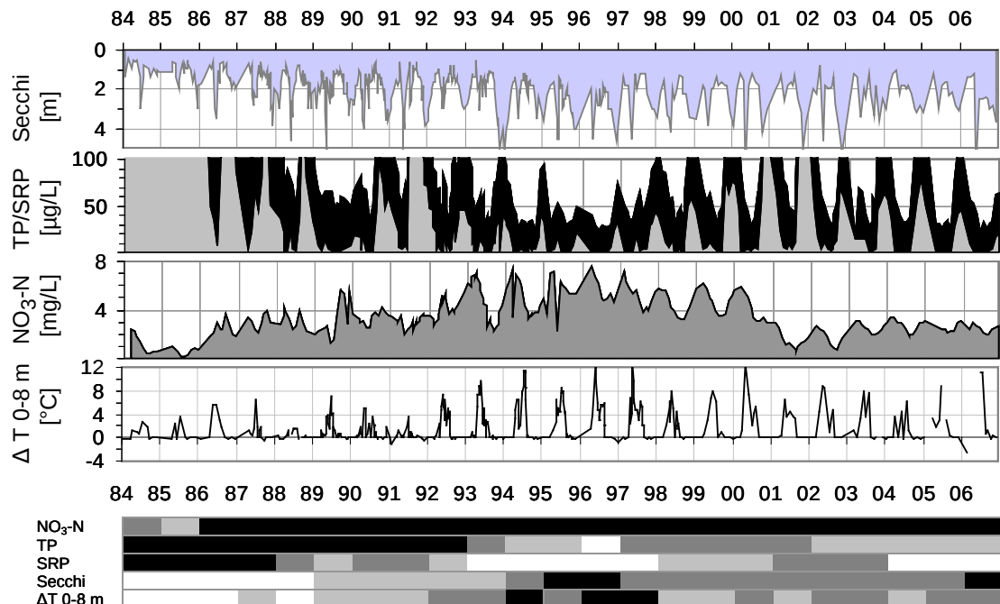
Figure 19. Hydrophysical and chemical growth conditions for phytoplankton
