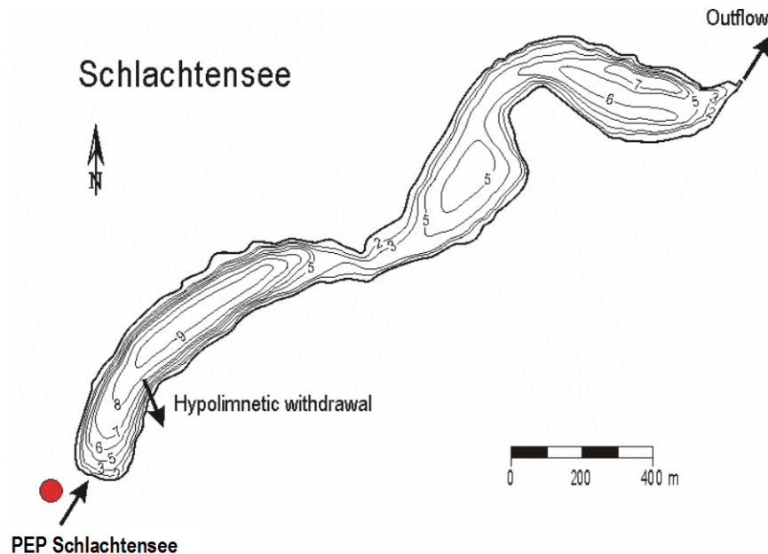
Figure 14. Map of Schlachtensee with bathymetric lines, the position of PEP and that of hypolimnetic withdrawal (Schauser & Chorus 2007)
