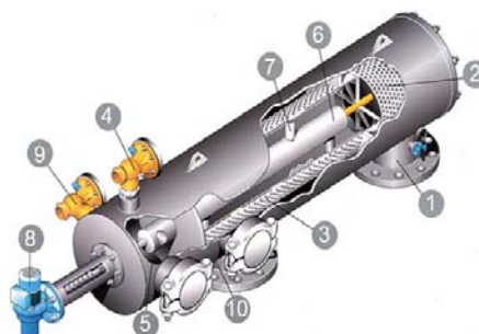
Figure 4: Screen filter. 1 Inlet; 2 Coarse screen; 3 Fine screen; 4 – 9 Backflushing system; 10 Outlet. ( http://www.process-controls.com/Pelmar/Pelmar_SE_Series.html )
