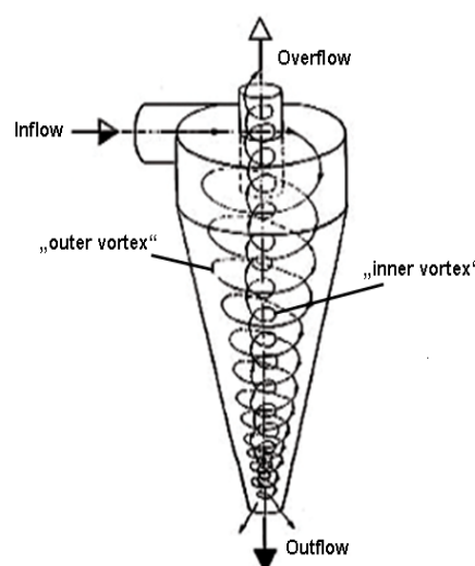
Figure 6: Hydroclone working principle
