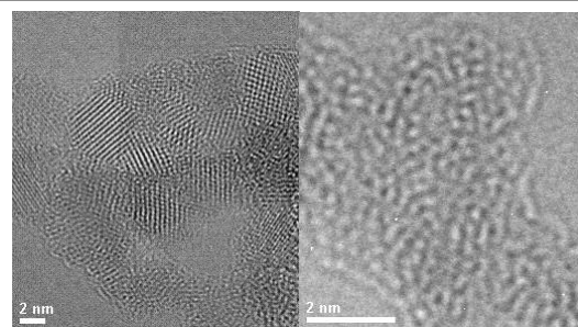
Figure II.1.3.2.d: left: thermally aftertreated crystalline TiO 2 NP; 1090000x magnification. On the right: thermally untreated amorphous TiO 2 NP; 559000x magnification.
