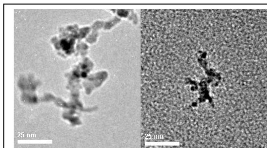
Figure II.1.3.2.c: left: thermally aftertreated crystalline TiO 2 NP; 39170x magnification. Right: thermally untreated amorphous TiO 2 NP; 39170x magnification
