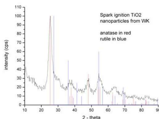
Figure II.1.3.2.f: X-ray diffraction analysis (XRD) of a TiO 2 NP sample on a silicone wafer demonstrating dominance of anatase.
