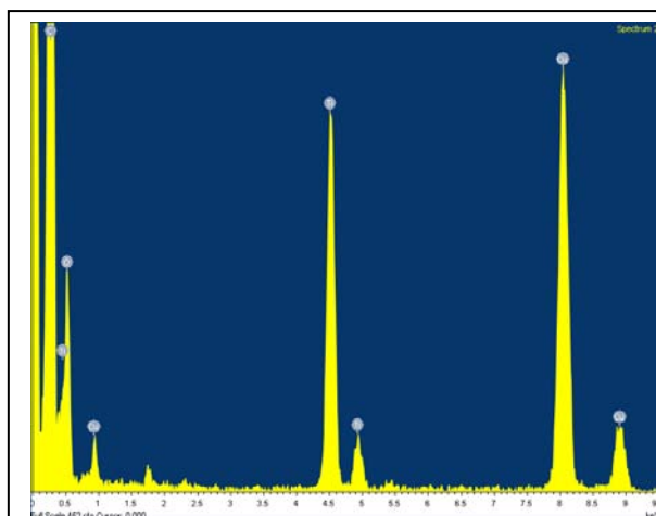
Figure II.1.3.2.e: XEDS analysis in the HRTEM confirms that the NP are chemically composed of TiO 2 . Beside the peaks for Ti and O 2 the copper lines of the EM substrate are recognised.
