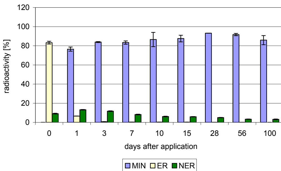
Fig. 6.7: Transformation of ^{14}\text{C} -cyanamide in silty clay soil after standard application (balances: 94 \pm 3 \% )
