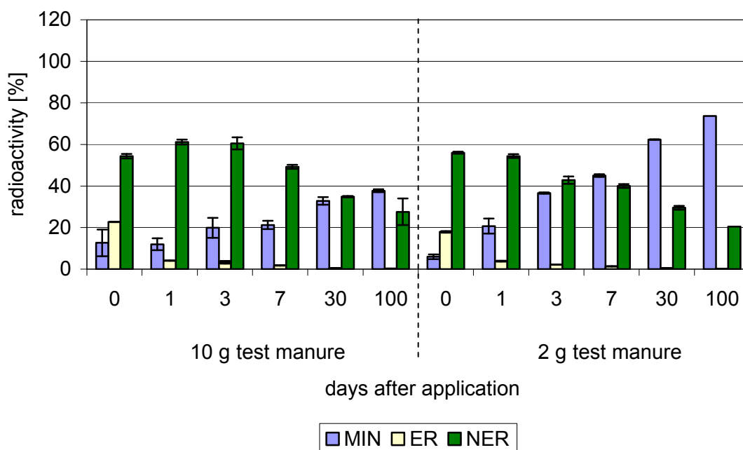
Fig. 6.8: Transformation of ^{14}\text{C} -cyanamide in silty clay soil after application of different amounts of bovine test manure (balances: 84 \pm 13 %)
