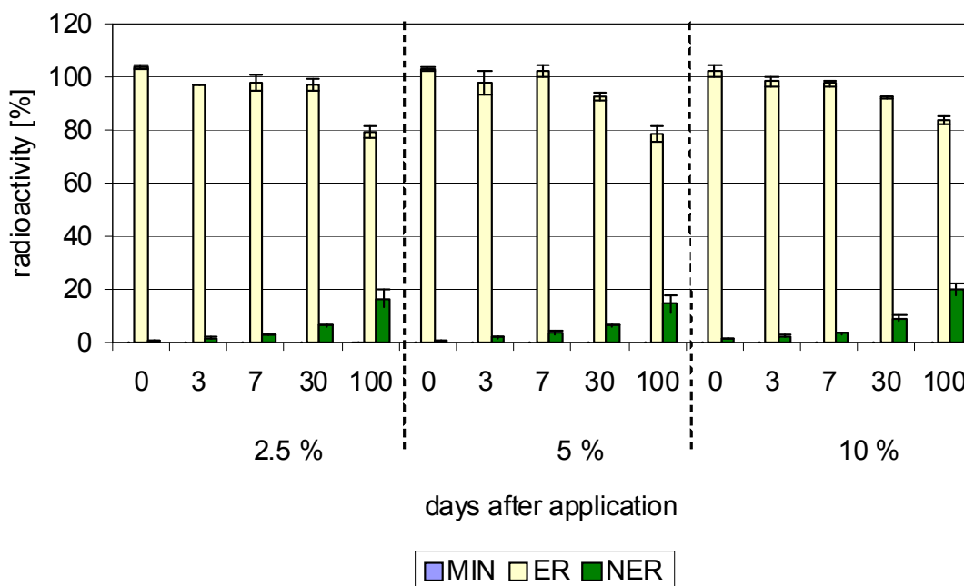
Fig. 5.3: Transformation of 14 C-imazalil in pig reference manure at different dry substance contents and at 20 ± 1 °C (balances: 101 ± 3%)
