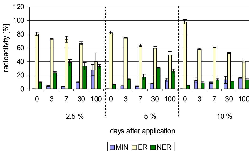
Fig. 5.7: Transformation tests of ^{14}\text{C} -cyanamide in pig manure at different dry substance contents and at 20 \pm 1^\circ\text{C} (balances: 92 \pm 12\% )
