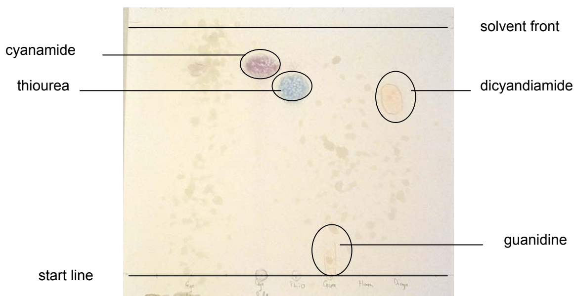
Fig. 4.9: Visualization of RTLC spots of cyanamide and transformation products by ferricyanide-nitroprusside dyeing on a silica gel plate developed using ethyl acetate/methanol (3:1)
