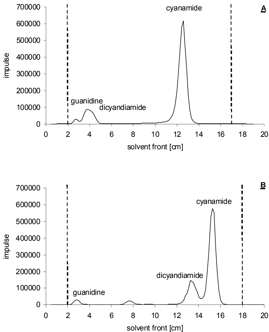
Fig. 5.4: Performance of two radio thin layer chromatographic systems for analyzing the stock-standard solution of ^{14}\text{C} -cyanamide dissolved in ethanol. Silica gel plates developed using ethyl acetate (A) and ethyl acetate/methanol (3:1) (B)
