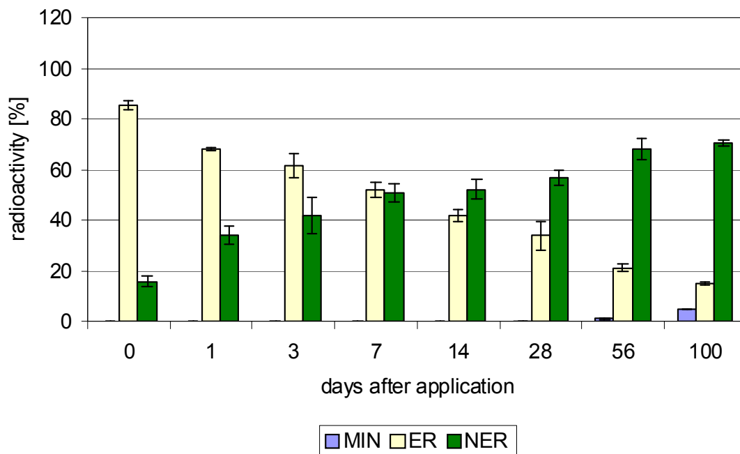
Fig. 6.2: Transformation of ^{14}\text{C} -imazalil in silty clay soil (45% of \text{WHC}_{\text{max}} ) after bovine test-manure application (balances: 97 \pm 6 \% )
