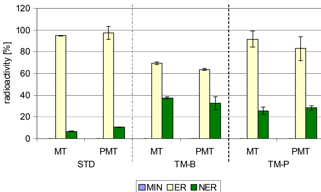
Fig. 6.6: Microbial (MT) and photoinduced microbial transformation (PMT) of ^{14}\text{C} -imazalil in silty clay soil after standard (STD) and test-manure application (TM) on the basis of bovine manure (B) and pig manure (P) within 3 days
