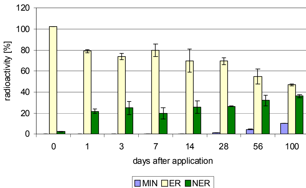
Fig. 6.1: Transformation of ^{14}\text{C} -imazalil in silty clay soil after standard application (balances: 98 \pm 4\% )
