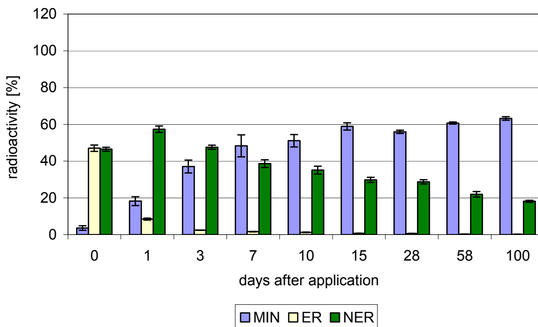
Fig. 6.9: Transformation of ^{14}\text{C} -cyanamide in silty clay soil after pig test-manure application (balances: 87 \pm 5\% )
