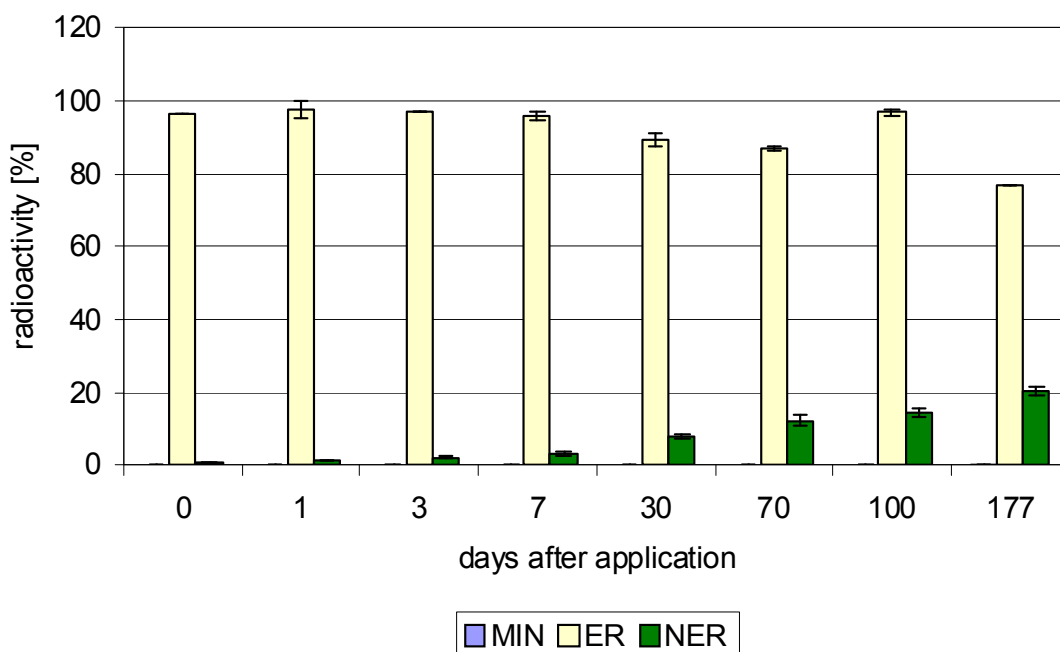
Fig. 5.2: Transformation of ^{14}\text{C} -imazalil in pig reference manure (balances: 100 \pm 5 \% )
