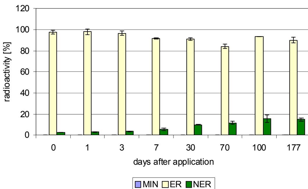
Fig. 5.1: Transformation of ^{14}\text{C} -imazalil in bovine reference manure (balances: 101 ± 4 %)
