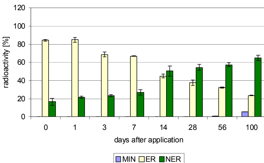
Fig. 6.3: Transformation of 14 C-imazalil in silty clay soil (35 % of WHC max ) after bovine test-manure application (balances: 96 ± 5 %)
