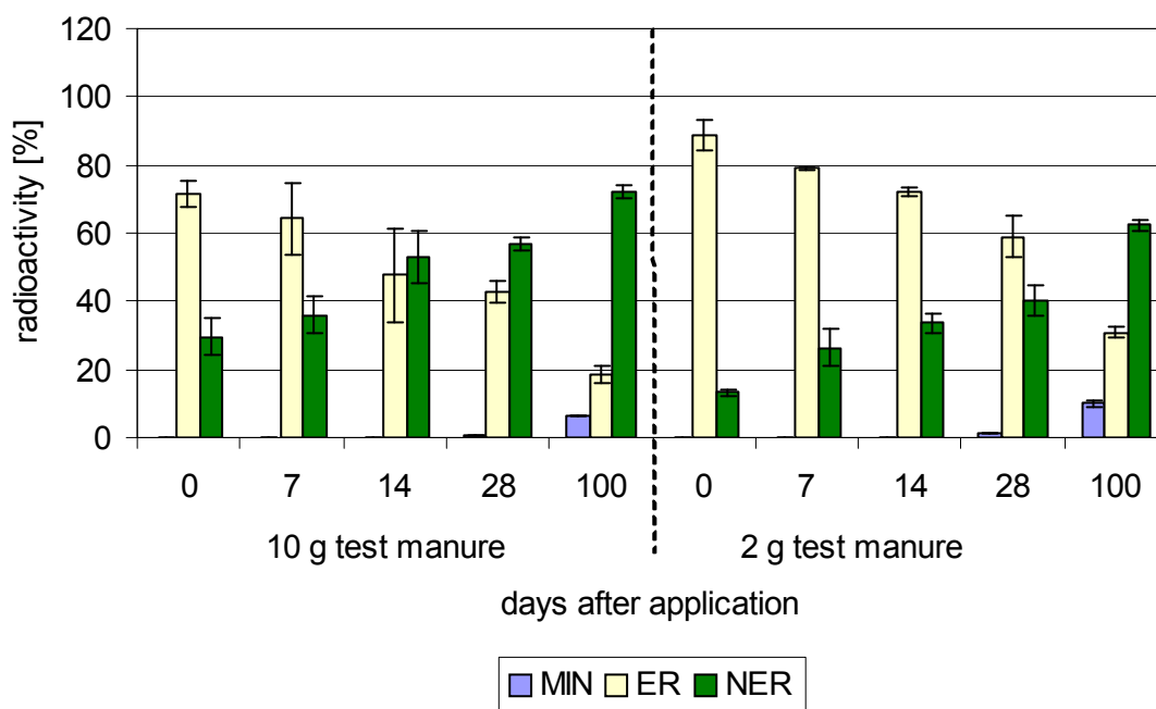
Fig. 6.4: Transformation of ^{14}\text{C} -imazalil in silty clay soil (35 % of \text{WHC}_{\text{max}} ) after application of different amounts of bovine test manure (balances: 102 \pm 3 %)
