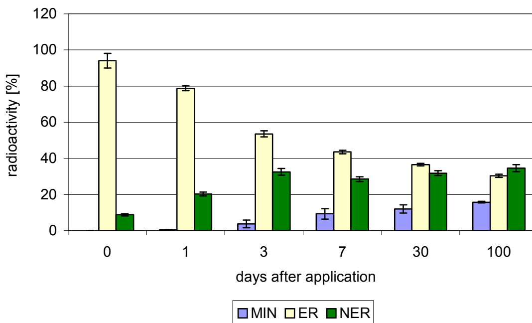
Fig. 5.5: Transformation of ^{14}\text{C} -cyanamide in bovine reference manure (balances: 89 \pm 10 %)
