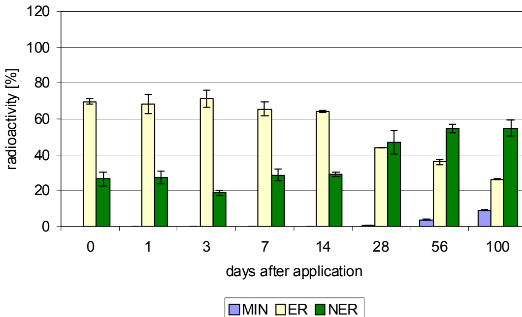
Fig. 6.5: Transformation of ^{14}\text{C} -imazalil in silty clay soil (35 % of \text{WHC}_{\text{max}} ) after pig test-manure application (balances: 93 \pm 1\% )
