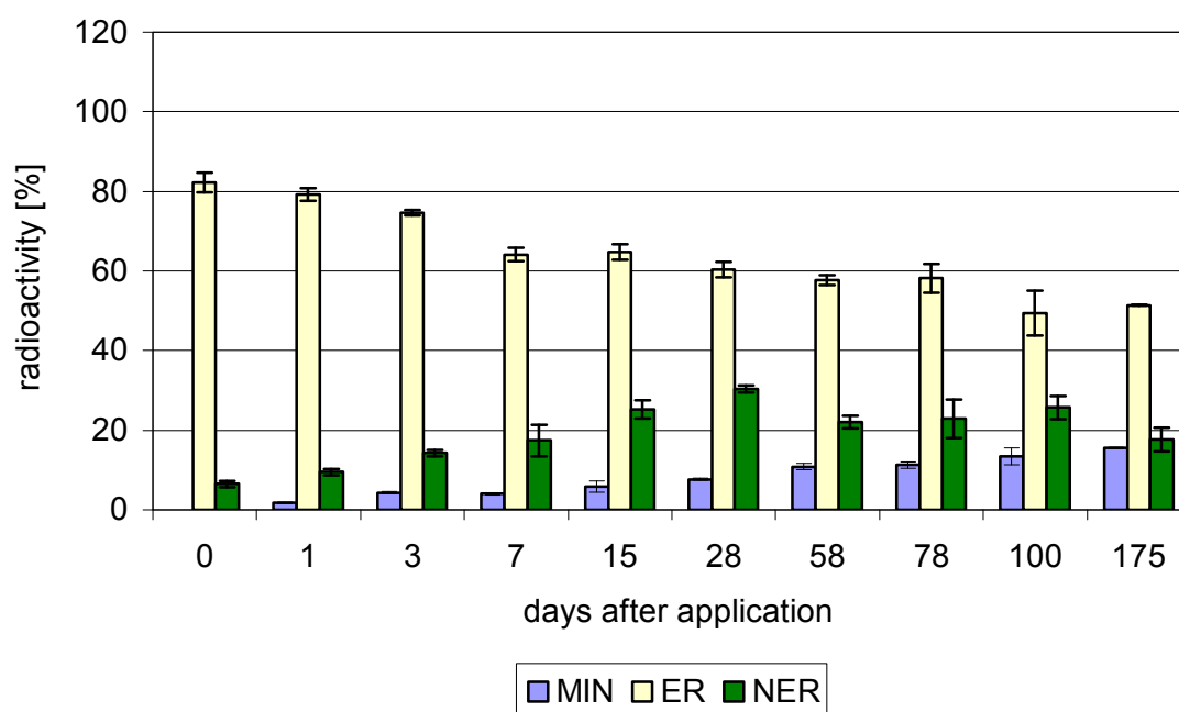
Fig. 5.6: Transformation of ^{14}\text{C} -cyanamide in pig reference manure (balances: 91 \pm 4 %)
