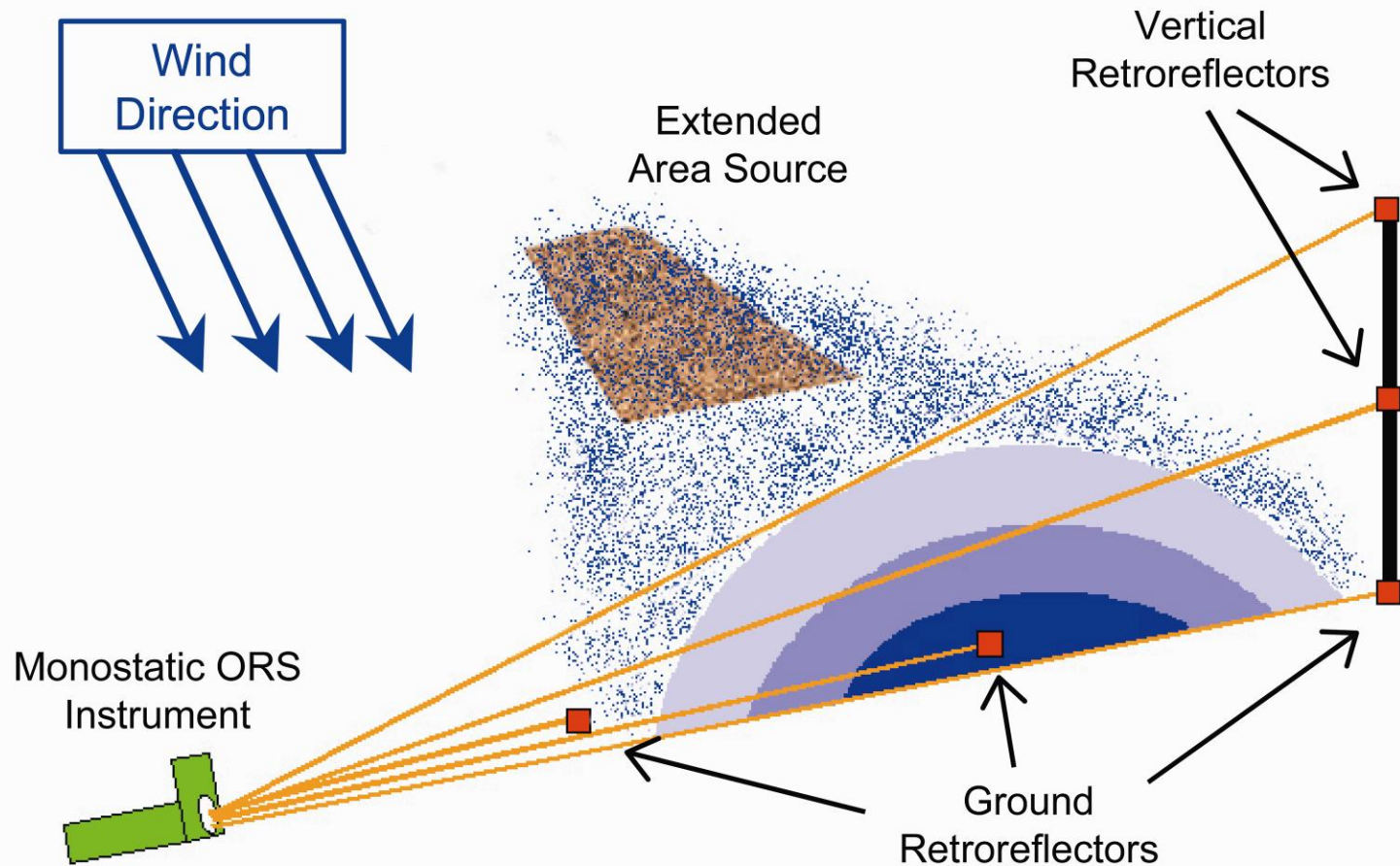
Vertical Radial Plume Mapping (VRPM)
