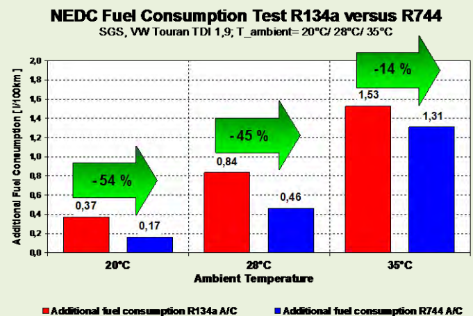
Fig. 3: Difference in fuel consumption between R 134a vs. CO 2 for a MAC system in a Volkswagen Touran (8).
