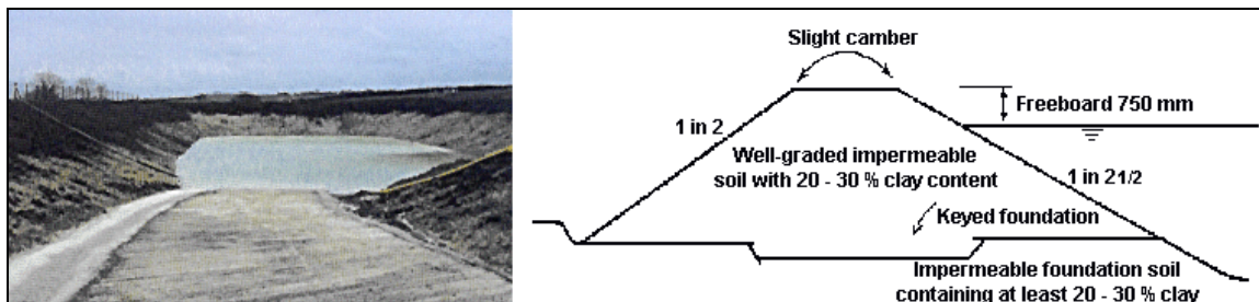
Abbildung 3.17: Example of an earth-banked slurry store and design features
