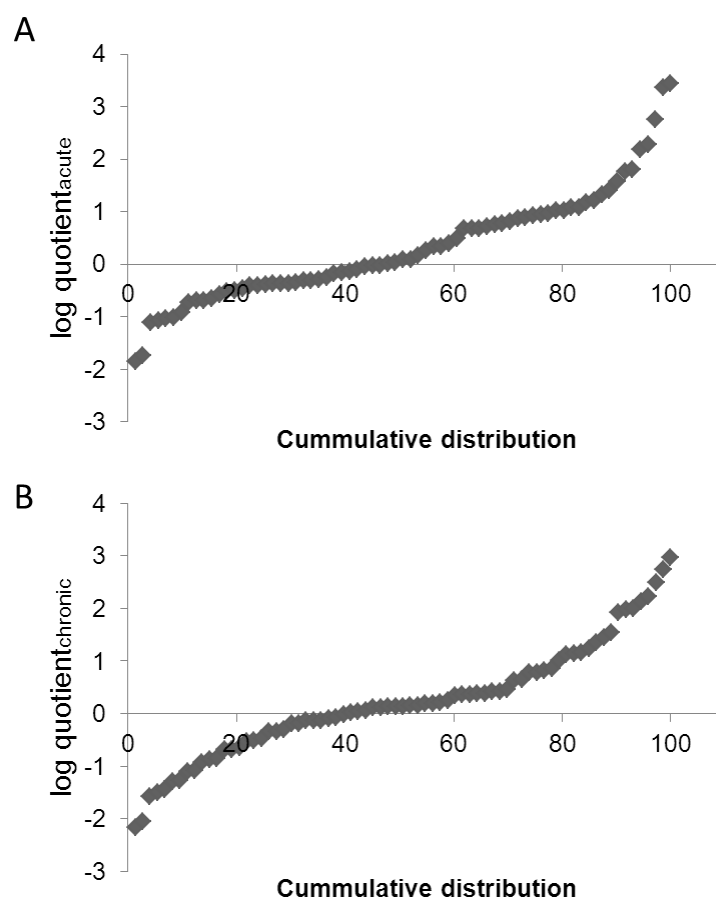
Figure 8: Sensitivity distribution between Daphnia and fish for pesticides in acute and chronic testing
