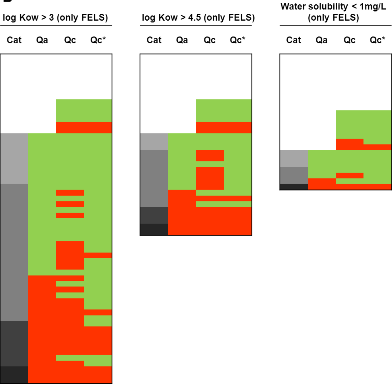
Sensitivity distribution between Daphnia and fish of substances with a log Kow >3 or >4.5, or of substances with poor water solubility (<1 mg/L) was elucidated by a heat map diagram as described in figure 4 for (A) the complete dataset and for (B) data only underlaid by FELS test.
