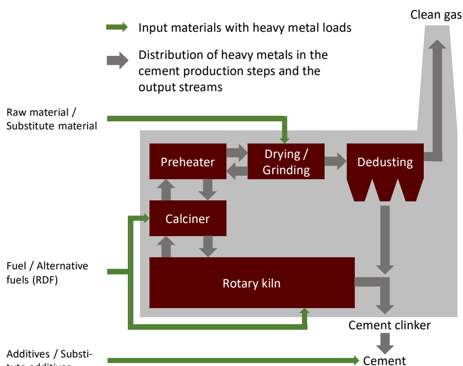
Figure 3: Heavy metal distribution in cement production
