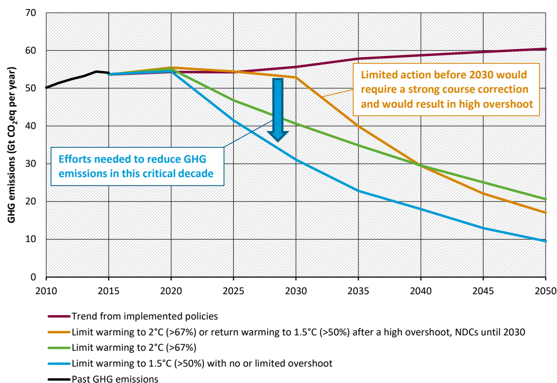
Figure 1: Global GHG emissions of modelled pathways, and projected emissions
